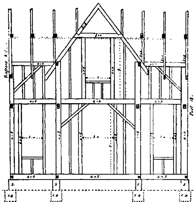
Figure 7: Balloon Frame and Traditional Frame
