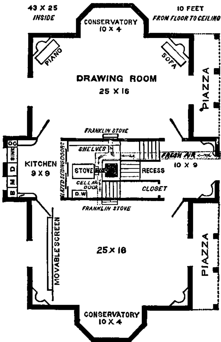
Figure 10: Flexible and Compact Floor Plan
