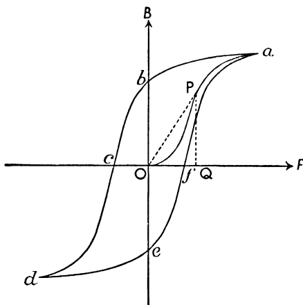
FIG. 114 Hysteresis Curve
