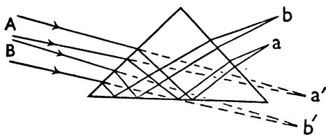
FIG. 33 Inversion of Image by Reflecting Prism a'b' Position of Image without Prism ba Inverted Image produced with Prism
