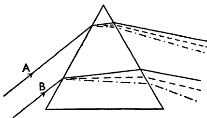
FIG. 60 Dispersion of Rays of Different Colours by Triangular Prism
