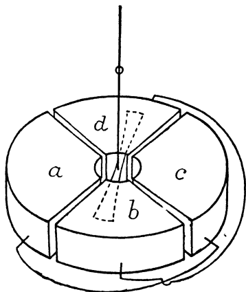
FIG. 129 The Quadrant Electrometer
