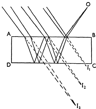
FIG. 29 Formation of Multiple Images by a Thick Mirror
