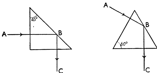
FIG. 32 Totally Reflecting Prisms ABC Path of Light
