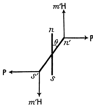
FIG. 109 Equilibrium position n's' of Needle in Tangent (B) Position of Gauss
