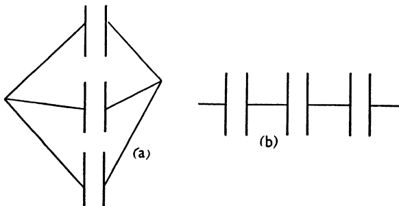
FIG. 84 Condensers joined (a) in Parallel (b) in Series
