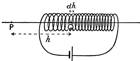
FIG. 119 Solenoid carrying Current
