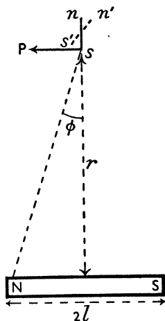
FIG. 108 The Tangent (B) Position of Gauss
