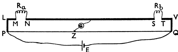
FIG. 99 The Metre Bridge
