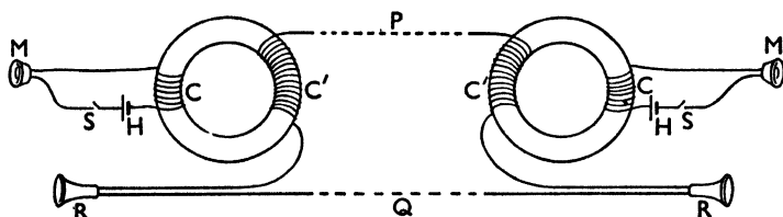
FIG. 137 Telephone Circuit
