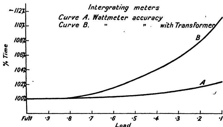
FIG. 68.—Tests of Accuracy of Wattmeters.
