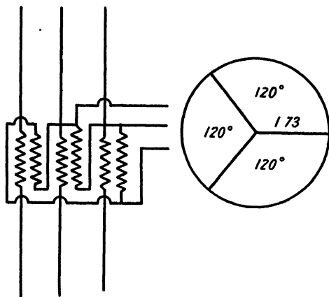
FIG. 37.—Diagram of Delta Connexion.
