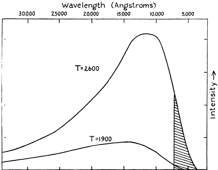
Fig. 71.—Energy curves for 1900° and 2600° K.
