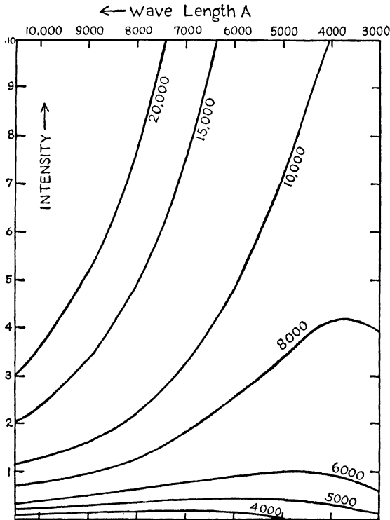
Fig. 34.—Energy emitted by a perfect radiator.
