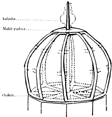
FIG. 19.—Construction of Ribbed Dome.
