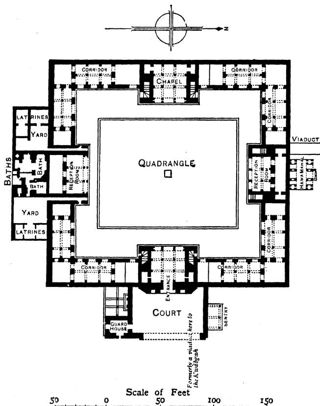
FIG. 42.—Ground Plan of Jodh Bât's Palace.
