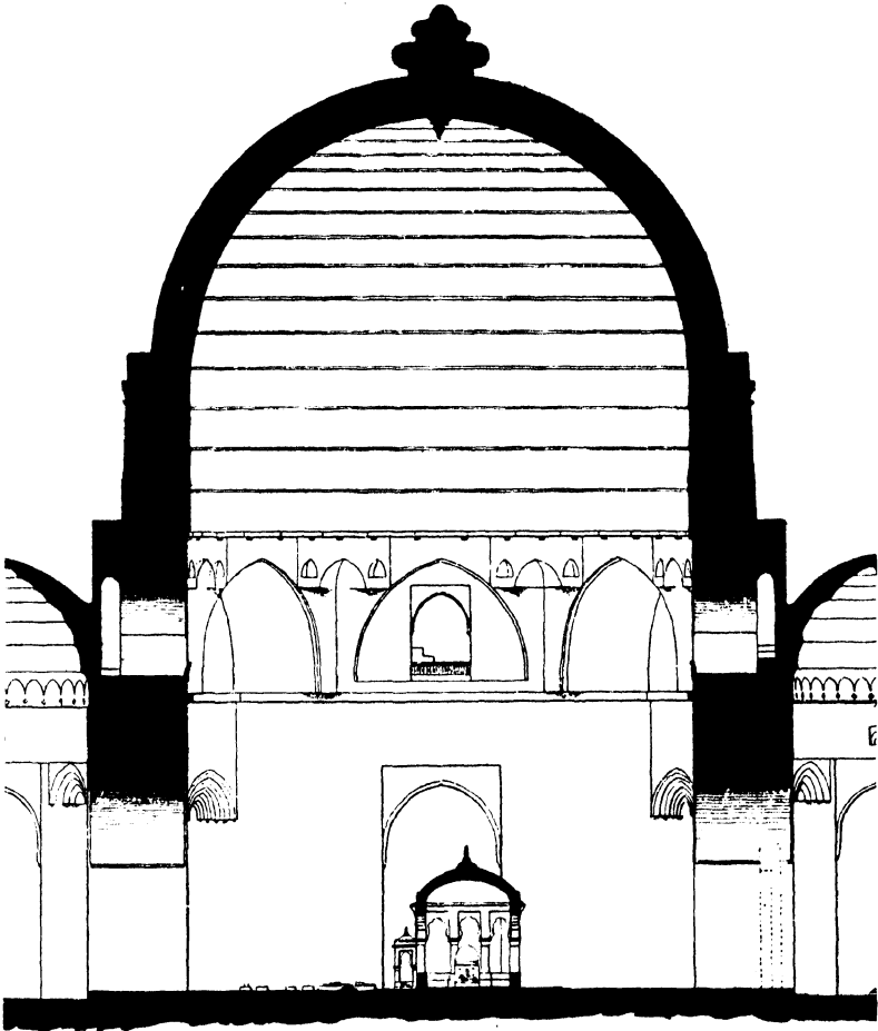
FIG. 27.—Daryâ Khan's Tomb : Section of Principal Dome (drawn by the Archæological Survey of India).
