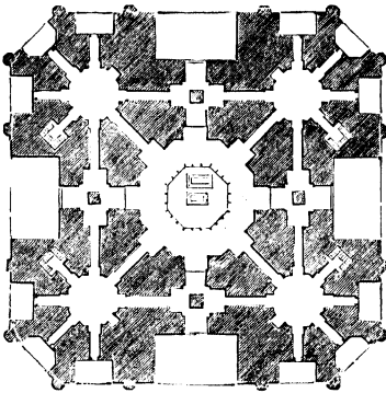
FIG. 1.—Plan of Tâj Mausoleum (from Fergusson's "Indian Architecture").
