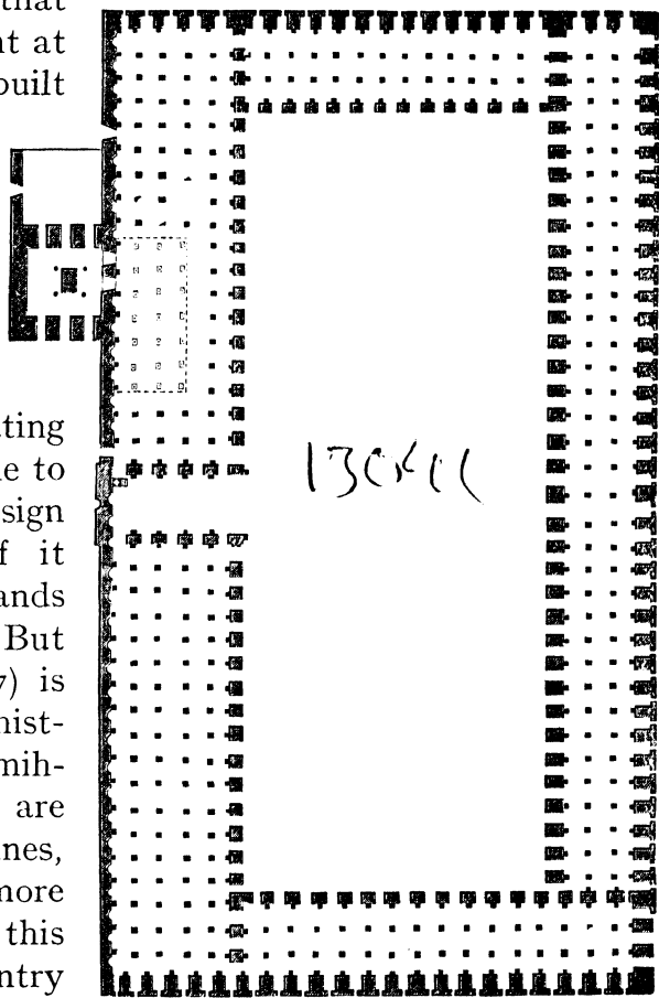
FIG. 7.—Plan of Âdînah Mosque (from Fergusson's "History").
