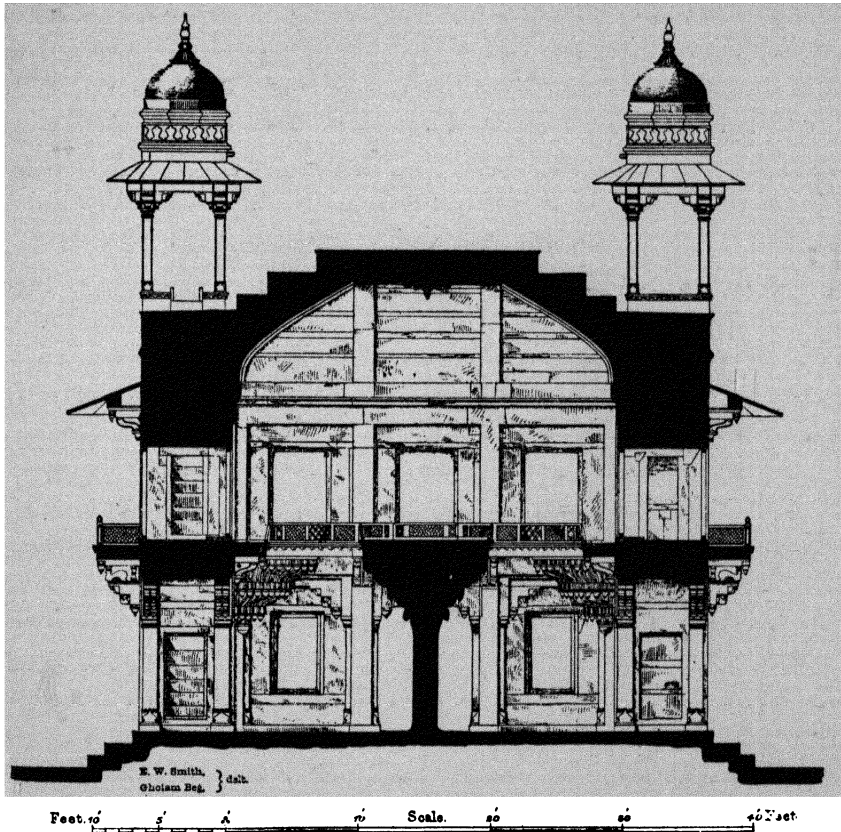
FIG. 40.—Section of the Dîwân-i-Khâs, Fatehpur-Sikrî (drawn by the Archæological Survey of India).
