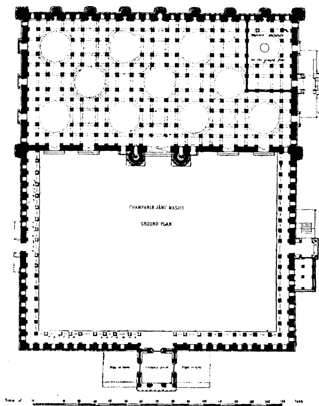
FIG. 33.—Plan of Jāmi' Masjid, Champanīr (drawn by the Archæological Survey of India).
