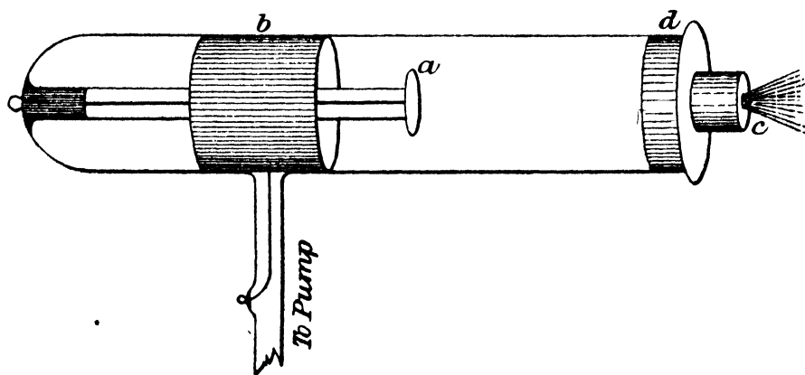
FIG. 7.—Tube for showing penetration of the cathode rays into the open. a is the disk-shaped cathode; a metal tube, b , serves as anode. Opposite the cathode is the thin aluminium window, c , carried by the brass cap, d . The rays issue from this window.
