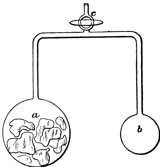
FIG. 24.—Arrangement for showing the condensation of the emanation. An inverted U-shaped tube carries at each end a glass bulb. The larger bulb, a , contains zinc sulphide or other fluorescent materials. The arrangement is exhausted of air, and the emanation introduced through the stopcock, c , which is then closed. The zinc sulphide glows brilliantly. On immersing b in liquid air, the emanation all condenses, and a loses its luminosity. When b is allowed to heat up again, the luminosity is restored.
