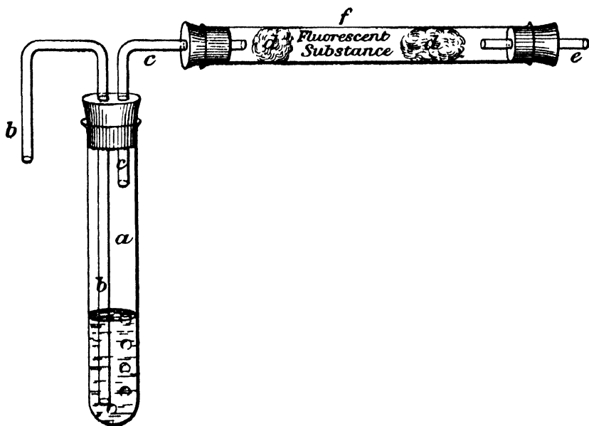
FIG. 28.—Apparatus for observing the connection. a is a test tube, containing radium solution. This tube is closed by a cork with two holes admitting two smaller tubes. One of these, b , passes to the bottom of the tube. The other, c , only just enters it. c is connected by means of another cork to the wider tube, f . f contains the fluorescent substance, confined between plugs of cotton wool, d , d . A small exit tube, e , is fitted to f by a cork.
