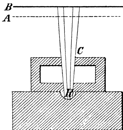
FIG. 22.—Bragg and Kleeman's apparatus. The radio-active surface R is of small size. A narrow cone of \alpha -rays from it is defined by the metal stop C . This cone falls perpendicularly on the ionisation chamber, consisting of a narrow space between two metal plates A, B , the first, A , being of gauze, to allow the \alpha -rays to enter. The ionisation chamber is movable to and from R .
