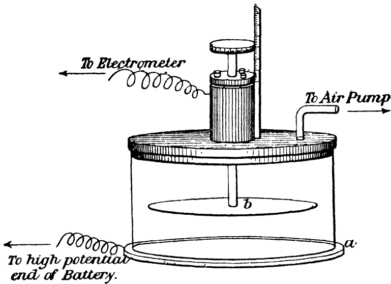
FIG. 21.—Parallel plate arrangement for investigating electrical conduction under Becquerel rays. The bottom plate, a , on which the radio-active substance is spread, is kept at any desired high potential. The upper plate, b , is movable, and parallel to the first. The distance can be altered and measured by the micrometer screw. A stuffing-box provides for air-tightness. The top cover of the glass jar is of ebonite to provide for insulation.
