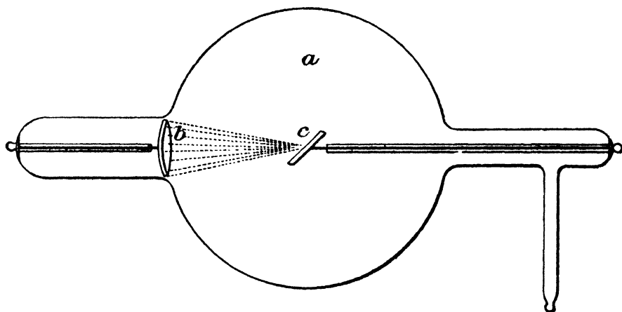
FIG. 8.—Focus bulb, a , for production of Röntgen rays. The cathode, b , is saucer-shaped, and the cathode rays from it (represented by dotted lines), converge on the plate-shaped anode, c , inclined at 45 degrees. The Röntgen rays issue from the front of this anode.
