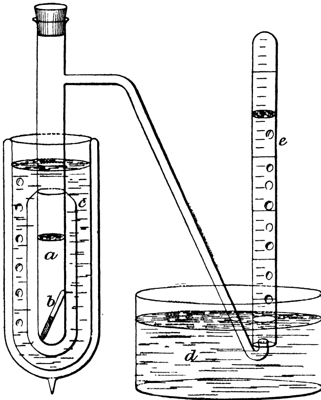
FIG. 26.—Measurement of the heat of emission of radium at the temperature of liquid air or liquid hydrogen. A double-walled vessel, a (vacuum jacketed), contains the liquid hydrogen. The radium, b , in a sealed tube, is immersed in this, and causes ebullition. The evolved gas is collected over water in d , in a graduated tube, e . To prevent the access of external heat, a is immersed in an outer vessel, c , also containing liquid hydrogen.
