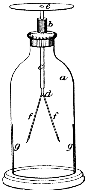
FIG. 10.—Gold-leaf electroscope of the ordinary form. A bell-jar, a , is fitted with an ebonite stopper, b . Through this passes a brass rod, c . c carries at its upper end a round brass disk, e . At its lower end a pair of gold leaves, f, f . g, g are strips of tinfoil communicating with the base of the instrument, and so with the earth. When a charge of electricity is imparted to c , the leaves stand apart by mutual repulsion, as shown. If they diverge far enough to touch g, g , they are discharged, and will collapse.
