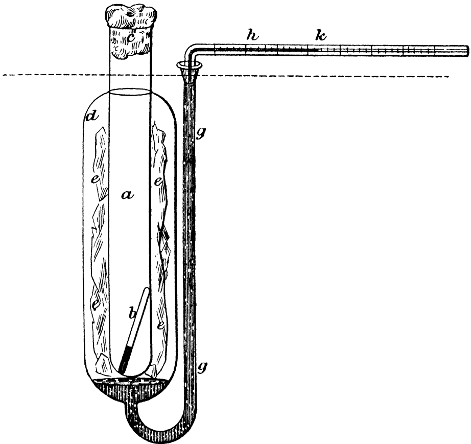
FIG. 25.—Bunsen's ice calorimeter, used in observing the heating effect of radium. a is a vessel like a test tube, into which the sealed tube, b , containing the radium, can be dropped. a is plugged at c with cotton wool, to guard against external heating. Round a is the outer chamber, d , which is quite full of freezing water, with a lump of ice, e e e e , round a . The bottom contains mercury, as does also the side tube, g g , and the horizontal graduated tube, h, k , of small diameter. The whole instrument is packed in ice up to the level of the dotted line, to prevent heat getting in from outside. While the radium is inside, the end, k , of the mercury thread is observed to be constantly receding, owing to the melting and contraction of the ice by the heat it liberates. As soon as the radium is withdrawn the thread becomes again stationary.
