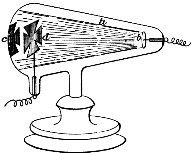
FIG. 4.—Arrangement for showing that the cathode rays are stopped by a solid obstacle, and cast a sharp shadow. A pear-shaped vessel, a , is used, which is highly exhausted. The plane or slightly convex cathode, b , sends out the rays, which cause brilliant green fluorescent luminosity on the opposite wall, c . The metal cross, d , which serves as anode, stands in the path of the rays, and casts a sharp black shadow on the luminous background.
