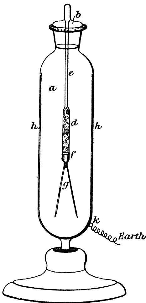
FIG. 16.—Arrangement for exhibiting the self-electrification of radium. A glass cylinder, a , is provided with a stopper, b . From this the thin glass tube, d , containing radium, is hung by the glass rod, e , which serves as an insulating support. d is covered with a film of phosphoric acid, which makes it a conductor. At the other end is a brass cap, f , which carries the gold leaves, g . The whole is exhausted through b , which subsequently serves as a means of supporting it. d loses negative electricity, thus acquiring a positive charge, and the leaves, g , diverge. The divergence increases until the leaves touch the tinfoil strips, h h , which are connected to the earth through a wire, k , sealed into the glass. This touching discharges the leaves, but they begin to diverge again immediately, if the radium preparation is active. This oscillation of the leaves goes on indefinitely.
