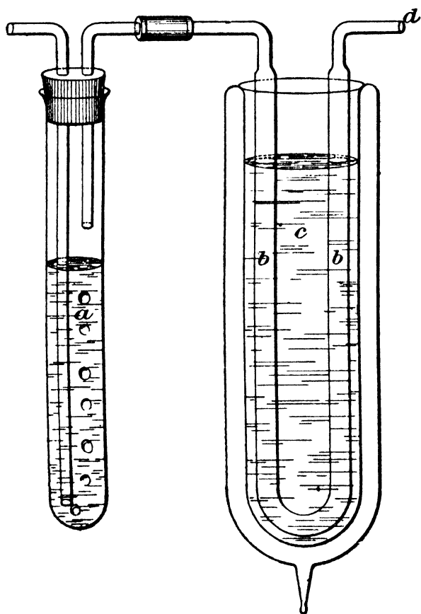
FIG. 23.—Arrangement for condensation of the emanation by liquid air. a is a solution of radium bromide, which yields the emanation. Air is bubbled through it, and carries the emanation through to the U-tube, b , immersed in liquid air, where it is condensed. The liquid air is contained in a double-walled vessel, c , with a vacuum between the walls. This serves to prevent the access of heat. While b is surrounded by liquid air, no emanation can escape through d , and it has lost all discharging power. When the liquid air is removed, the accumulated emanation evaporates, and the issuing air is strongly radio-active.
