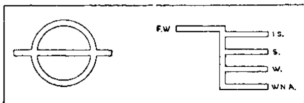
The load line and Plimsoll mark.
