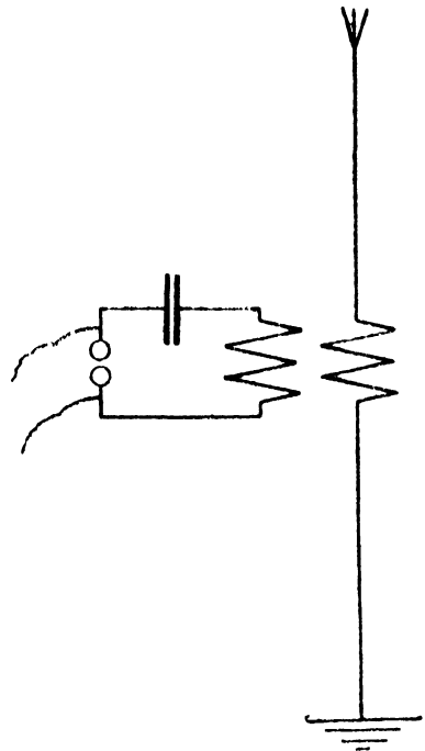
Fig. 8. Braun's Transmitter (1899).
