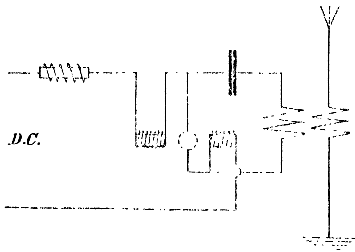
Fig. 10. Poulsen Arc Generator (1903). Showing "coupled circuit," re-introduced in 1924.
