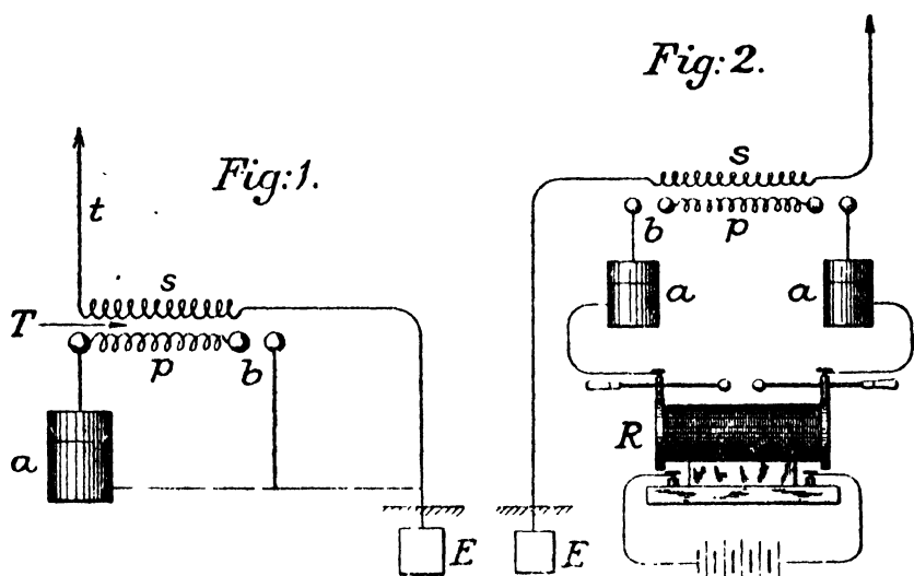
Fig. VII. Braun's Coupled-circuit Transmitter.
