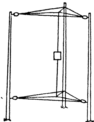
Fig. 13. Counterpoise Aerial (1905).
