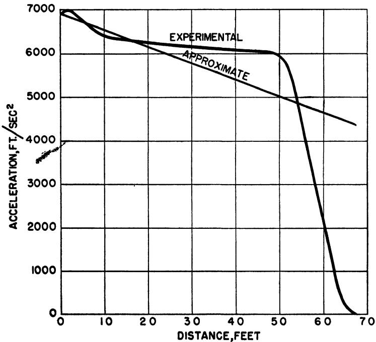
FIG. III.10.1.—Acceleration-distance curve of a rocket.
