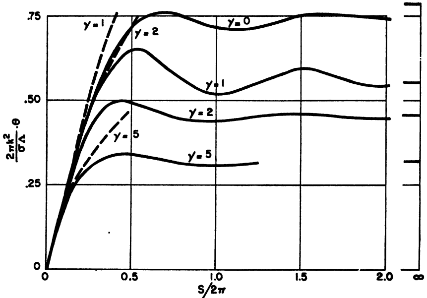
FIG. III.12.1.—Dispersion due to jet misalignment distance for a slowly spinning rocket launched from a zero-length launcher. Dashed lines give vacuum solution. k = radius of gyration about a transverse axis through the C.G. \sigma = wave length of yaw. \Delta = jet misalignment distance. \gamma = number of revolutions per wave length of yaw.
