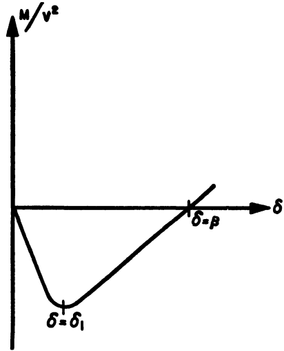
FIG. III.14.1.—Example of upsetting moment curve. M = upsetting moment. v = velocity. \delta = yaw.
