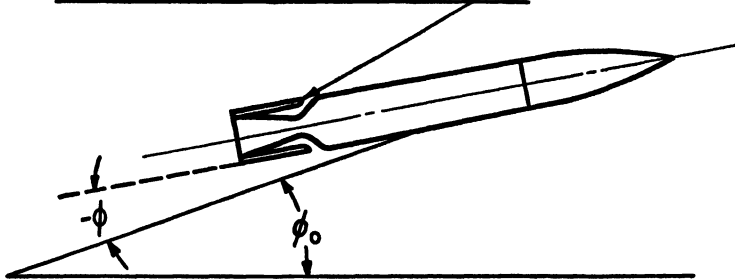
FIG. IV.2.3.—Coordinate system for tipping-off rocket, fixed support. x -axis parallel to launcher. y -axis perpendicular to launcher. Radius of rocket is r .
