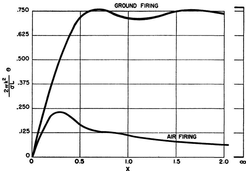
FIG. III.5.2.—Dispersion due to jet malalignment distance for air and ground firing from a zero-length launcher. For air firing, aircraft velocity is one-half of burnt velocity of rocket relative to aircraft.
