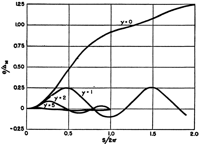
FIG. III.12.3.—Dispersion due to fin malalignment angle for a slowly spinning rocket launched from a zero-length launcher. \Delta_M = fin malalignment angle. \gamma = number of revolutions per wave length of yaw.
