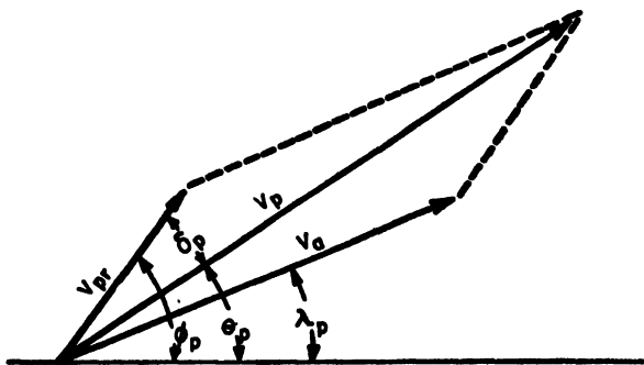
FIG. IV.1.1.—Boundary conditions resulting from a launcher velocity.
