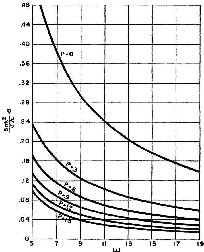
Fig. III.13.3.—Dispersion due to jet misalignment distance for a slowly spinning rocket with burning distance equal to a half wave length of yaw. k = radius of gyration about a transverse axis through the C.G. \sigma = wave length of yaw. \Lambda = jet misalignment distance. \omega as defined by (III.13.1).
