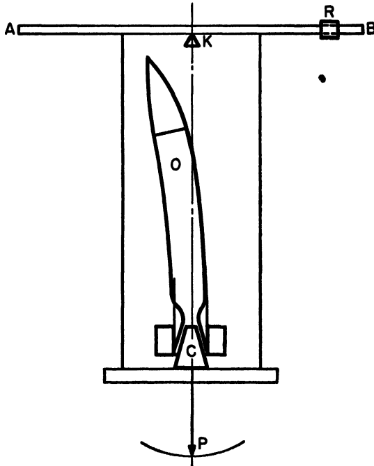
FIG. III.16.1.—Balance for measuring L
