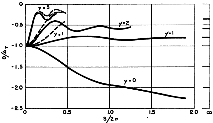
FIG. III.12.2.—Dispersion due to jet misalignment angle for a slowly spinning rocket launched from a zero-length launcher. Dashed lines give vacuum solution. \Delta\tau = jet misalignment angle. \gamma = number of revolutions per wave length of yaw.
