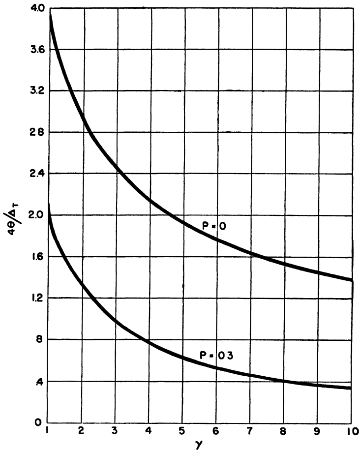
FIG. III.12.5.—Dispersion due to jet malalignment angle for a slowly spinning rocket with large burning distance.
