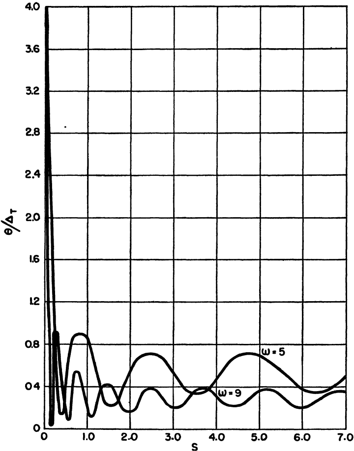
Fig. III.13.2.—Dispersion due to jet malalignment angle for a slowly spinning rocket launched from a zero-length launcher. \Delta r = jet malalignment angle. \omega as defined by (III.13.1).
