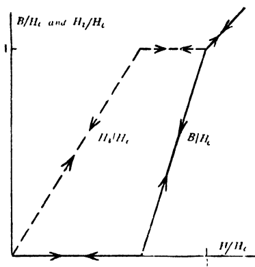
Fig. 7a. B - H curve and H_i - H curve for a sphere (schematic representation of results of de Haas and Guinau(7)).
