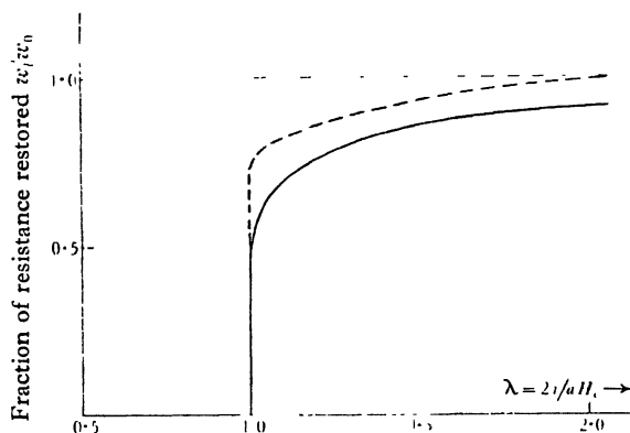
Fig. 12a. Restoration of resistance by a current at constant temperature: full curve—theoretical; broken curve—experimental (Shubnikov and Alexeevski (7)).
