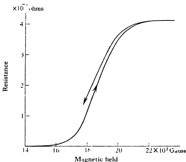
Fig. 19. Restoration of resistance of Pb-Bi eutectic by a magnetic field (4.22° K.) (de Haas and Voogd (4)).
