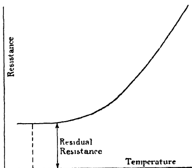
Fig. 1. Schematic resistance-temperature curve for a metal.
