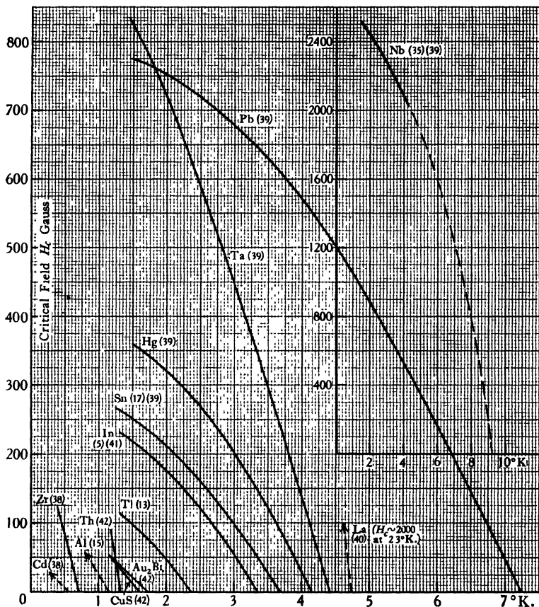
Fig. 23. H_c - T curves. (The bracketed figures give references to the literature.)
