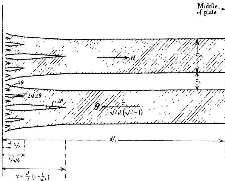
Fig. 9. Penetration of a magnetic field into a plate in the intermediate state (Landau (16)).
