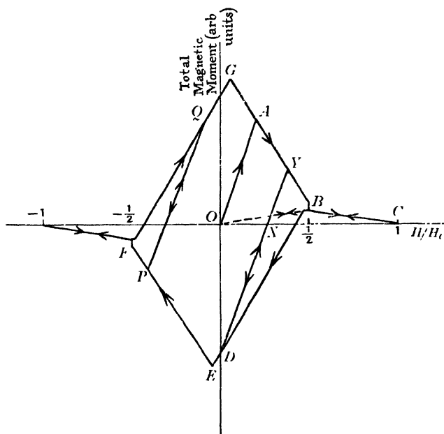
Fig. 10. Magnetization curve of a superconducting ring (schematic).
