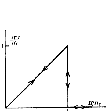
Fig. 4 a . Magnetization curve of a superconducting long cylinder.
