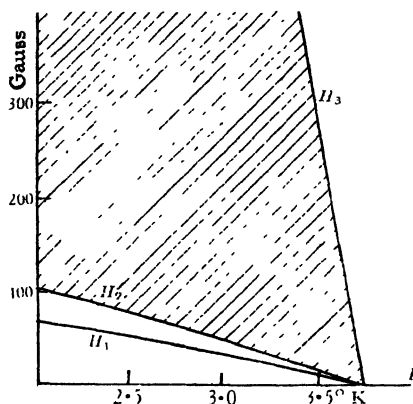
Fig. 21.† Temperature variation of H_1 , H_2 and H_3 for the alloy \text{PbTl}_2 (Rjabinin and Shubnikov (7)).
