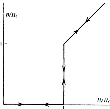
Fig. 4 b . B - H curve of a superconducting long cylinder.
