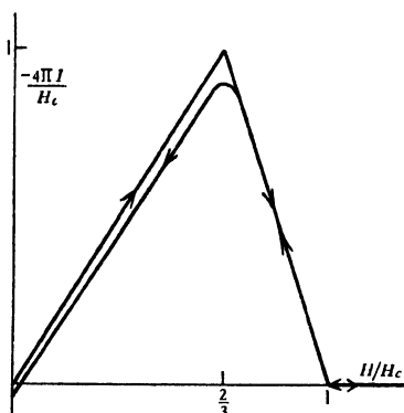
Fig. 7b. Magnetization curve of a lead sphere (Shoenberg (9)).
