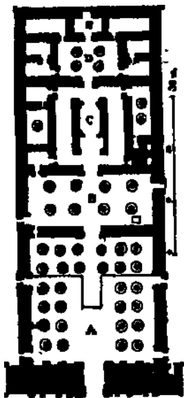
Fro. 73.—Temple of Khonsu at Karnak.
