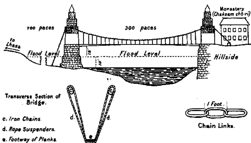
IRON SUSPENSION BRIDGE OVER TSANGPO.
