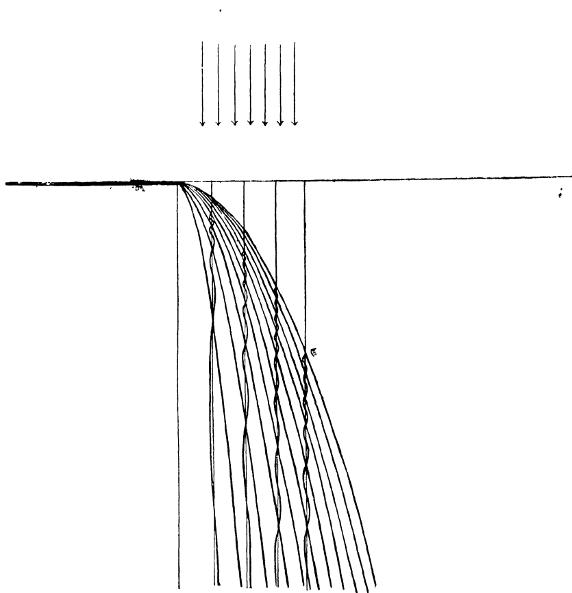
Lines of energy flow in the field due to diffraction at a straight edge.
