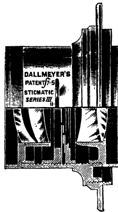
FIG. 37.—Dallmeyer non-convertible Stigmatic Objective (Series III.)
