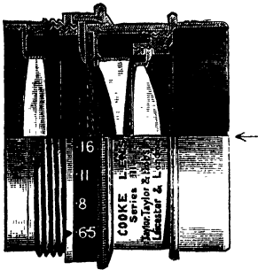
FIG. 38.—Cooke-Taylor Lens (Series III.).
