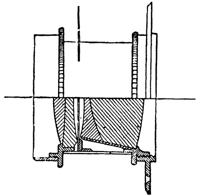
FIG. 14.—Steinheil's Antiplanet .
