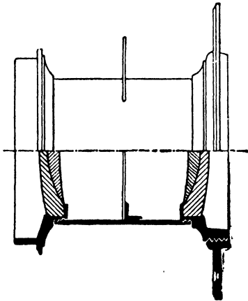
FIG. 21.—Steinheil's Aplanat .
