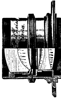
FIG. 16.—Zeiss's Anastigmat , Series IIa.
