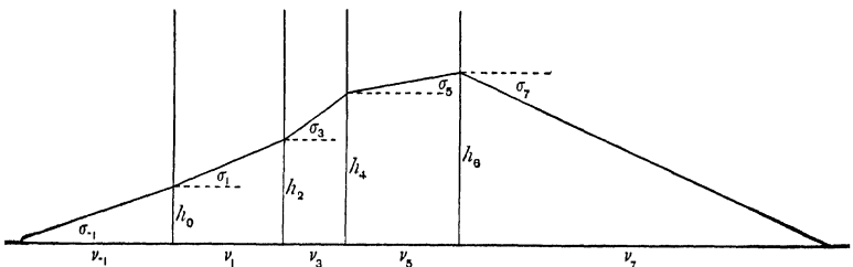
FIG. 48.—Path of a Ray through Optical System.
