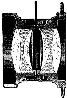
FIG. 22.—Goerz's Double Anastigmat .
