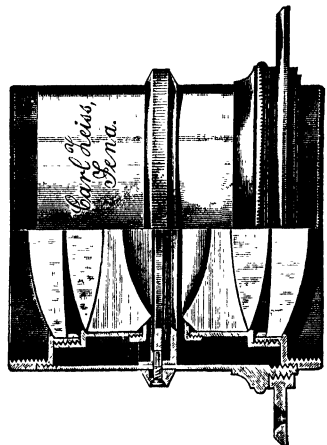
FIG. 28.— Planar Objective of Zeiss .
