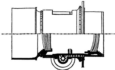
FIG. 13.—Petzval's Portrait-Objective.
