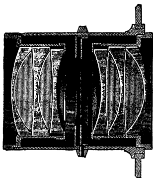
FIG. 22A.—Goerz's Double Anastigmat , Series IIa.
