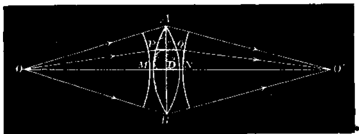
Fig. 58.—Aplanatic Lens.
