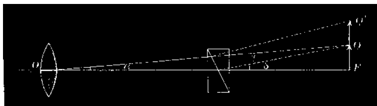
Fig. 162.—Double Image Micrometer.
