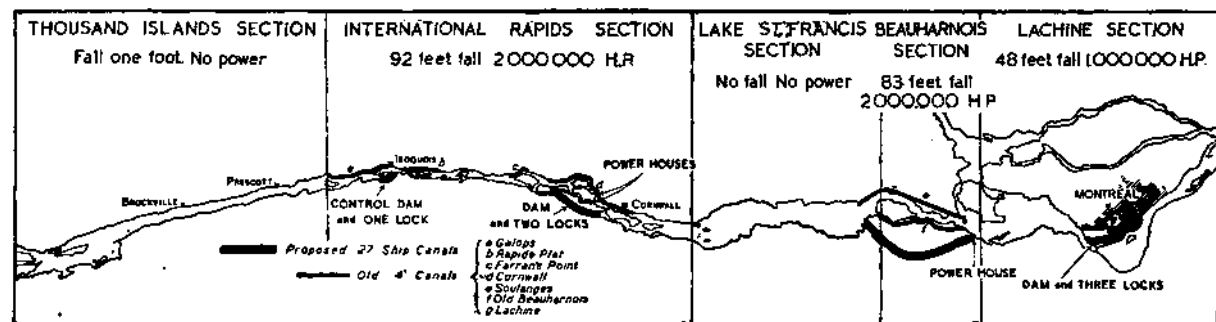
FIG. 106A.—Plan of St. Lawrence Deep Waterway Scheme.
