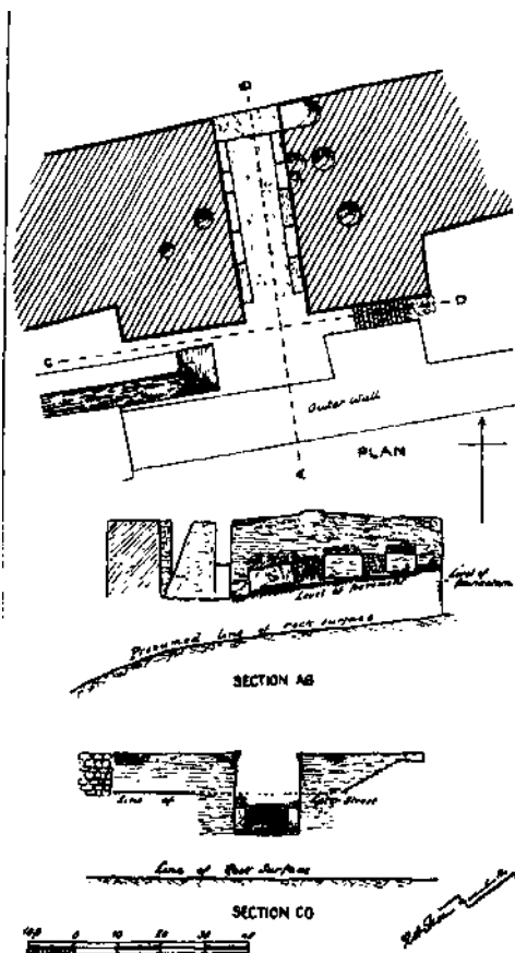
FIG. 125.—SOUTHERN GATE, INNER CITY WALL PLAN AND ELEVATIONS
