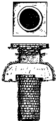
FIG. 148.—PLAN AND SECTION OF THE MACCABAEON WELL
