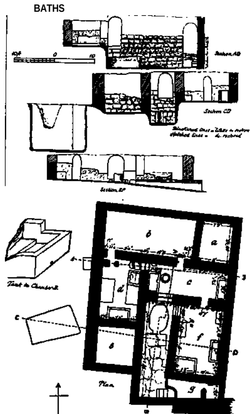
FIG. 110.—PLAN OF THE SYRIAN BATH-HOUSE
