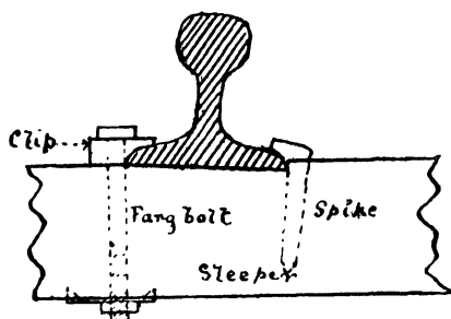
FLAT-FOOTED RAIL.
