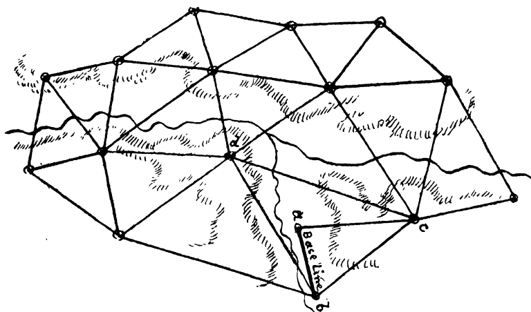
FIG. 3.—NETWORK SYSTEM.
