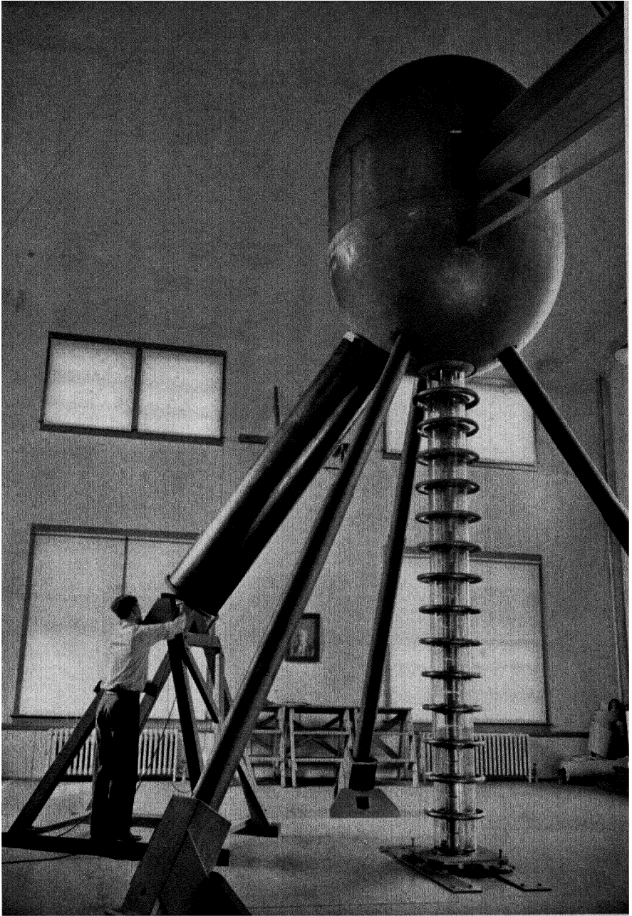
THE ELECTROSTATIC GENERATOR AT THE CARNEGIE INSTITUTE, WASHINGTON, WITH A CASCADE TUBE IN POSITION
