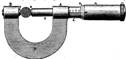
FIG. 11.—Screw-gauge.
