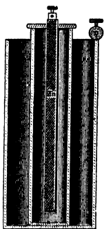
FIG. 324.—A Daniell cell.
