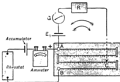
FIG 382 —The potentiometer.
