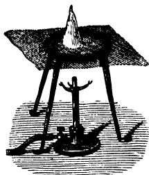
FIG. 143.—Principle of the Davy safety lamp.
