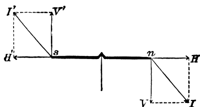
FIG. 273.—A compass-needle acted upon by magnetic forces inclined to the horizontal.
