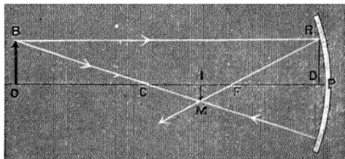
FIG. 192.—Real image, by means of a concave mirror.
