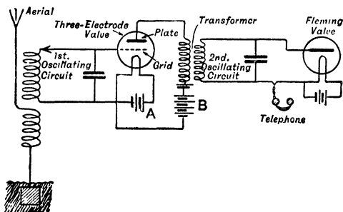
FIG. 413.—A WIRELESS RECEIVING-SET, in which the high-frequency oscillations are amplified by a 'triode valve,' then transmitted through a transformer to a second oscillating circuit, and rectified by a Fleming valve.
