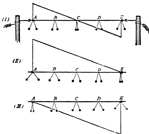
FIG. 319.—Difference of potential along an electrified string.
