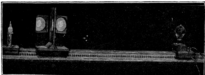
FIG. 162.—Bunsen's grease-spot photometer.
