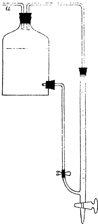
Fig. 1. Reservoir in direct communication with burette. The tube a may be placed in direct connexion with an apparatus for generating hydrogen.
