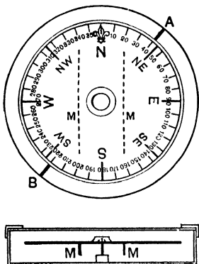
FIG. 13. —Magnetic compass.
