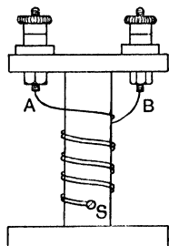
FIG. 53.—Resistance coil.
