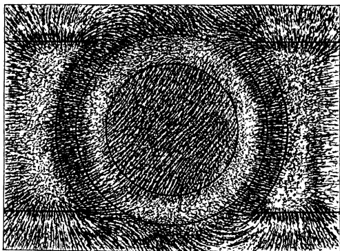
FIG. 138.—Field due to magnets and armature together.
