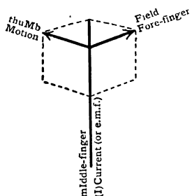
FIG. 105.—Right-hand rule for induced e.m.f.
