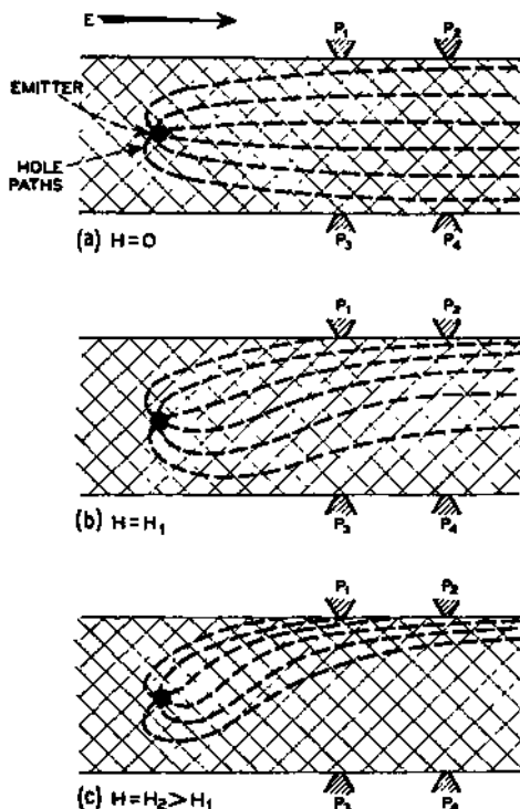
FIG. 3-11—Paths of Holes Injected into n-Type Filament Showing Concentration by Magnetic Field.
