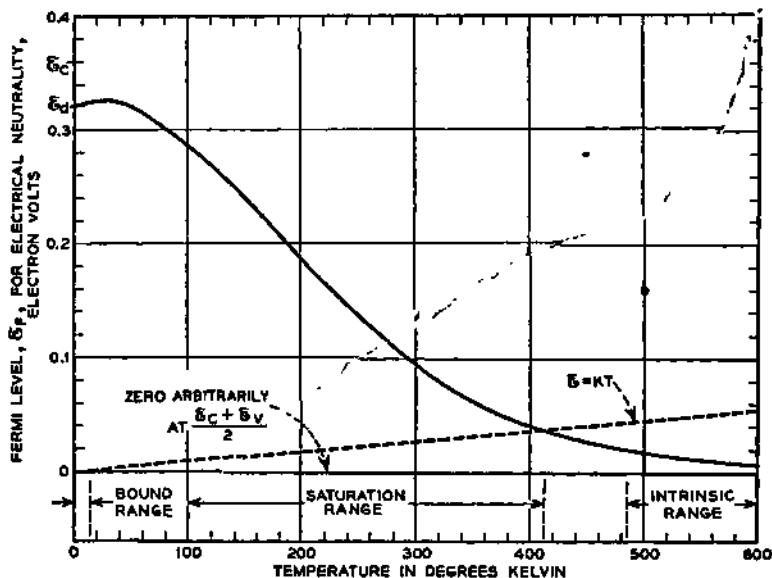
FIG. 10-6—The Fermi Level for Electrical Neutrality Plotted Against Temperature, for Germanium with N_d = 10^{15} \text{ cm}^{-3} and N = 10^{14} \text{ cm}^{-3} and \mathcal{E}_c - \mathcal{E}_d = 0.04 \text{ ev} .
