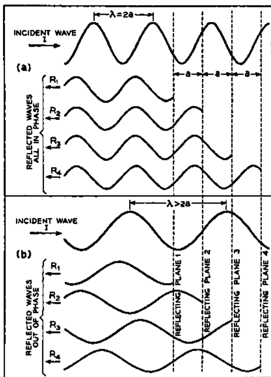
FIG. 5.8—Phase Relations between Reflected Waves, Showing Critical Condition for n = 2a .
