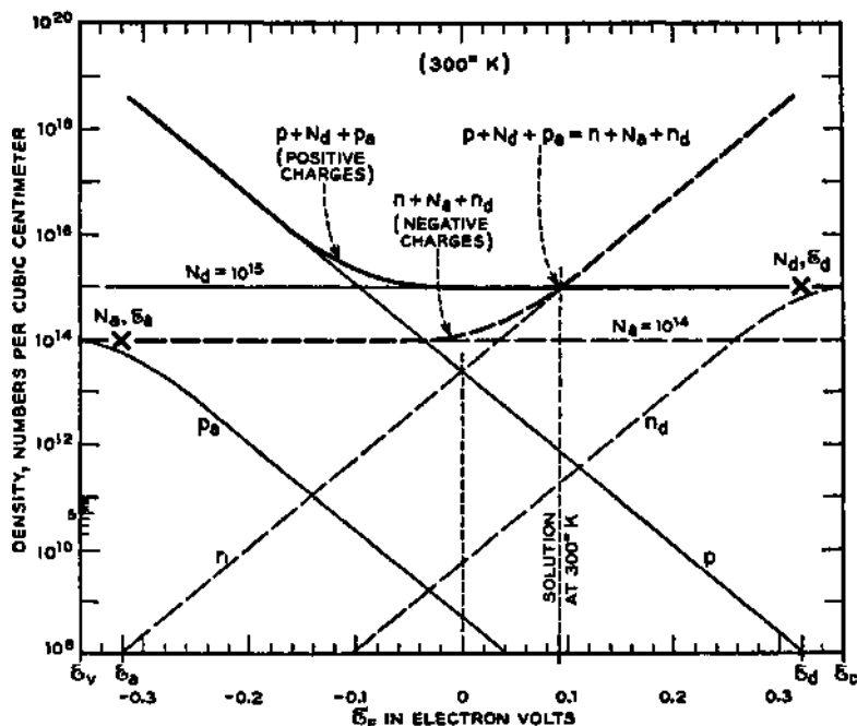
FIG. 16-2—Solution for \mathcal{E}_F with Density of Acceptors, N_a = 10^{14} \text{ cm}^{-3} , Density of Donors, N_d = 10^{15} \text{ cm}^{-3} and T \cong 300^\circ\text{K} .
