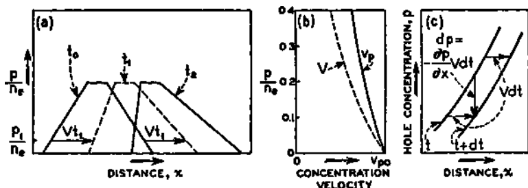
FIG. 12-8—Deformation of a Pulse of Holes Due to Conductivity Modulation. (Drawn for b = 2 .)
