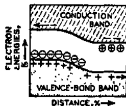
FIG. 4-5—Unsymmetrical p-n Junction Showing How More Current (Forward is Shown) is Carried by More Abundant Type of Carrier (Holes).
