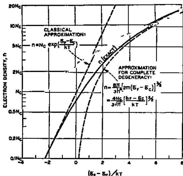
FIG. 10-5—Exact Dependence of n Upon (\mathcal{E}_F - \mathcal{E}_c) and T Compared to Limiting Forms.
