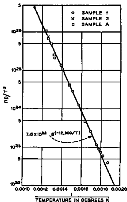
FIG. 16-9—Plot of Experimental Data for Several Silicon Samples for Comparison with Equations (10) and (11) of Section 16-4.
