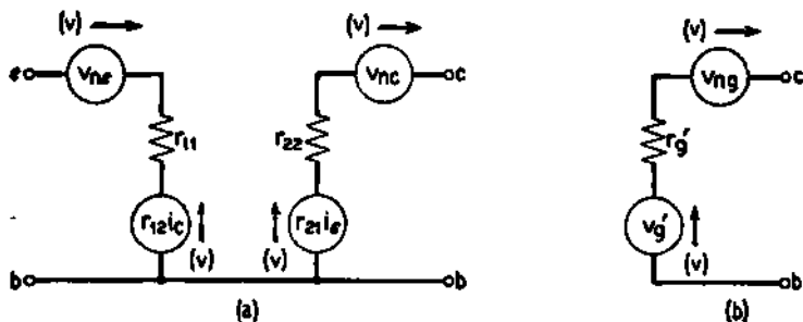
FIG. 2-9—Noise in Transistors.
