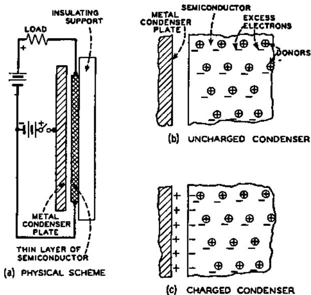
FIG. 2-2—Modulation of Conductance by Surface Charges.
