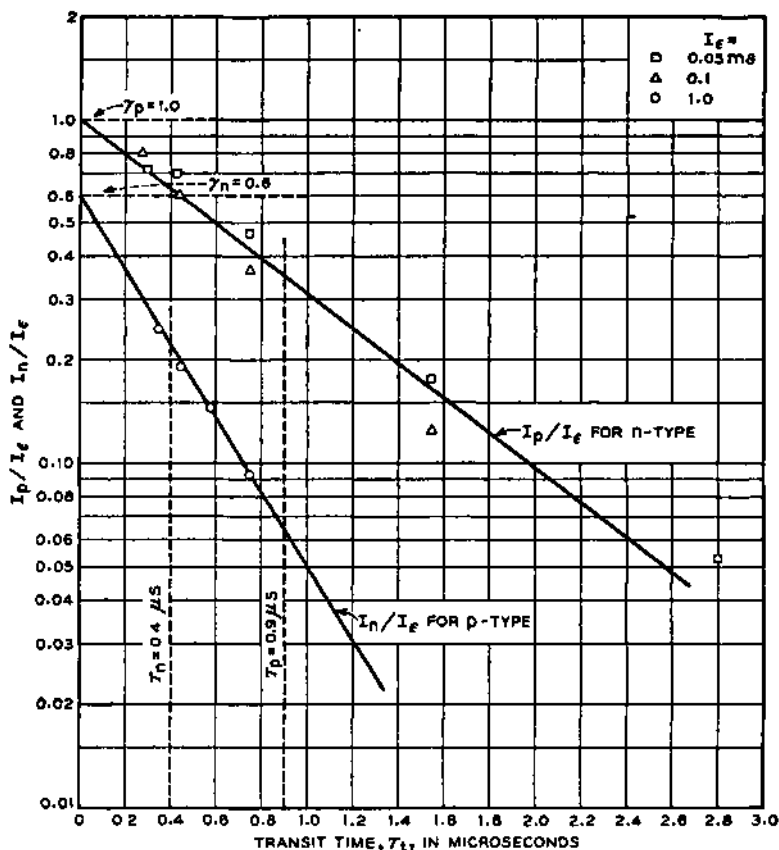
FIG. 3-5—Extrapolation of Measured Hole and Electron Currents to Zero Transit Time in Order to Determine y .
