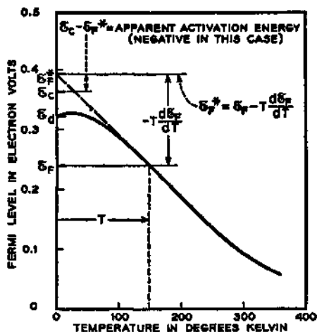
FIG. 16-8—Apparent Activation Energy for N_a = 10^{14} .
