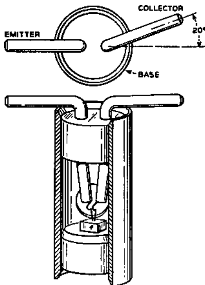
FIG. 2-4—Cut-away View of the Type-A Transistor.
