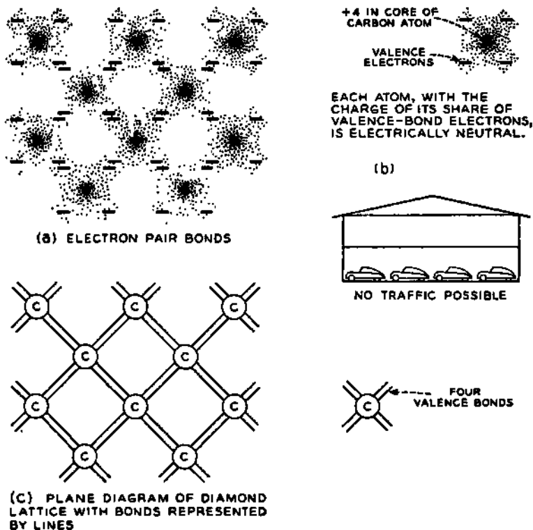
FIG. 1-4—Electrons in the Diamond Structure.
