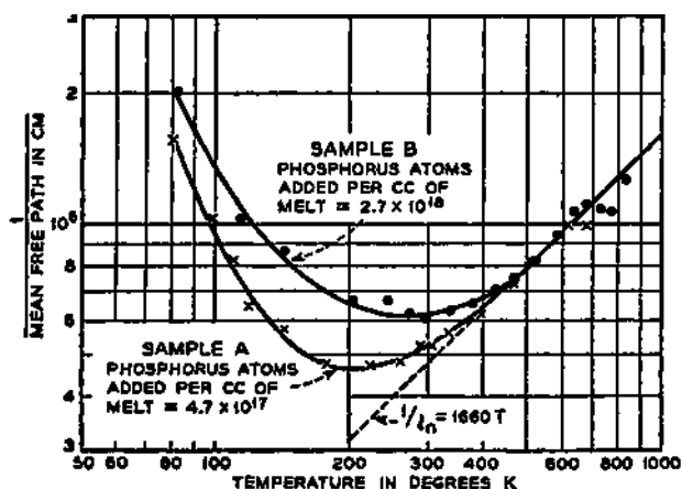
FIG. 11-12—Mean Free Path in Silicon-phosphorous Alloys versus Temperature.
