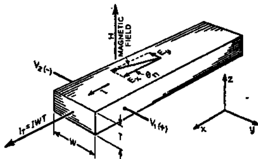
(3) VOLTAGE COMPONENTS FOR CONDUCTION BY ELECTRONS IN A MAGNETIC FIELD
