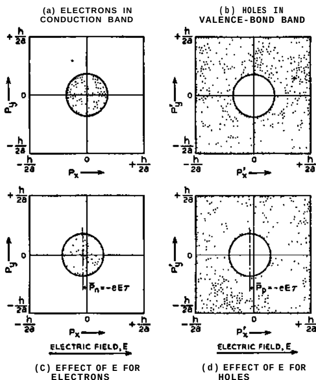
FIG. 8-4—Effect of Electric Field, E_x , on the Distribution of Electrons and Holes in the Brillouin Zone.
