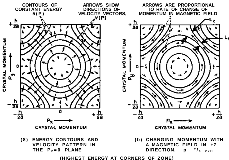
FIG. 7-3—Energy, Velocity and Effect of a Magnetic Field in a Brillouin Zone.
