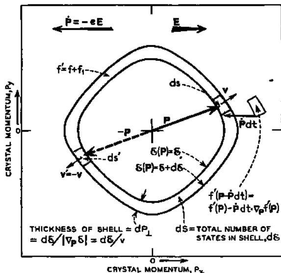
FIG. 11-6—Disturbance of Equilibrium by Electric Field.
