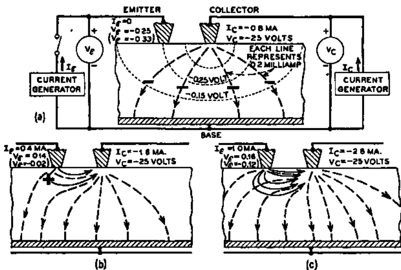
FIG. 4-10—Transistor Currents Diagram.
