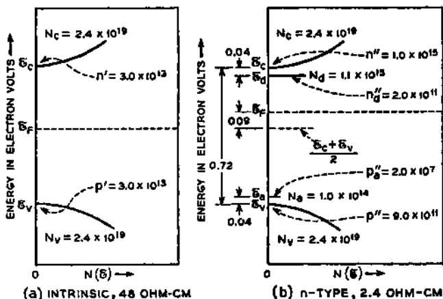
FIG. 10-7—Theoretical Distributions of Quantum States in Energy, Effective Densities, and Densities of Electrons and Holes for Germanium. (The values shown are illustrative and not exact.)
