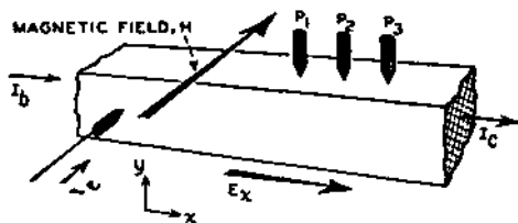
(a) EXPERIMENTAL ARRANGEMENT
