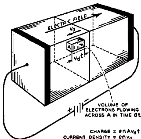
FIG. 8-6—Relationship Between Drift Velocity and Current.
