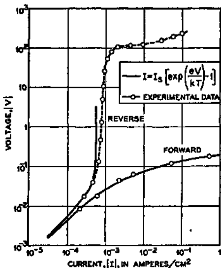
FIG. 4-6—Theoretical Rectification Curve and Experimental Data for a p-n Junction.
