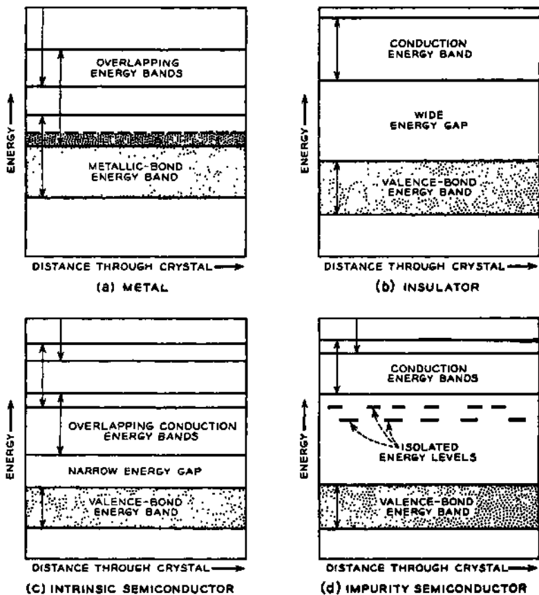
FIG. 5-13—Energy Band Diagrams for Several Crystal Types.
