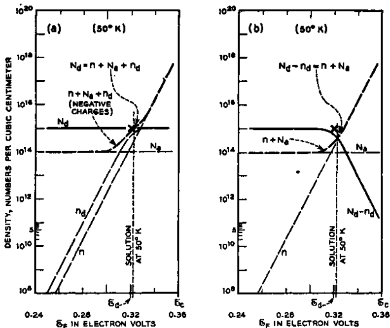
FIG. 16-5—Solution for \mathcal{E}_F with Density of Acceptors, N_a = 10^{14} \text{ cm}^{-3} , Density of Donors, N_d = 10^{15} \text{ cm}^{-3} and T \cong 50^\circ \text{K} .
