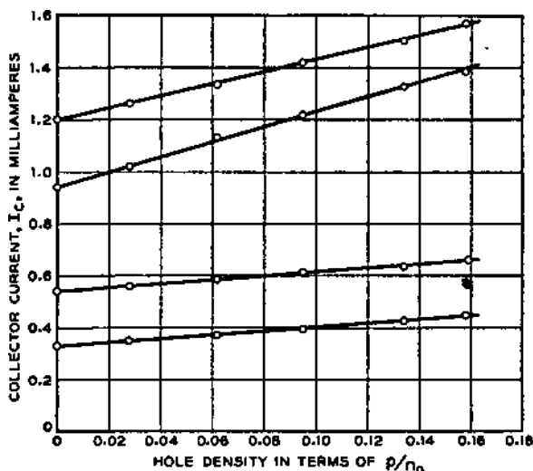
FIG. 3-6—Dependence of Collector I_c Upon Average Hole Density Being Swept by Collector Point. Collector Biased 20 Volts Reverse.
