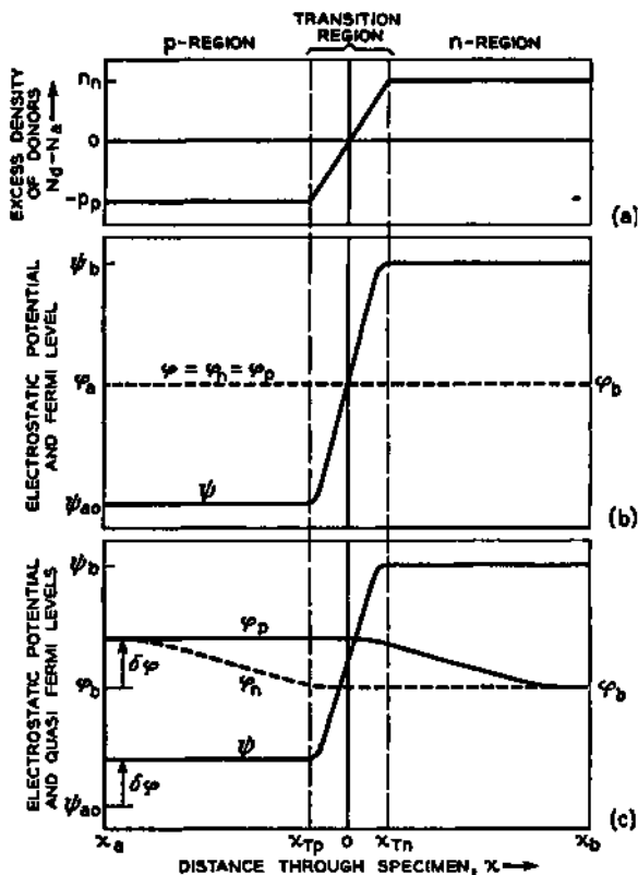
FIG. 12-3—Simplified Model of a p - n Junction.
