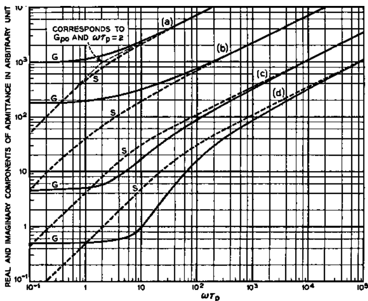
FIG. 12-4—Real and Imaginary Parts, G and S , of the Admittance for Hole Flow into the w -Region.
