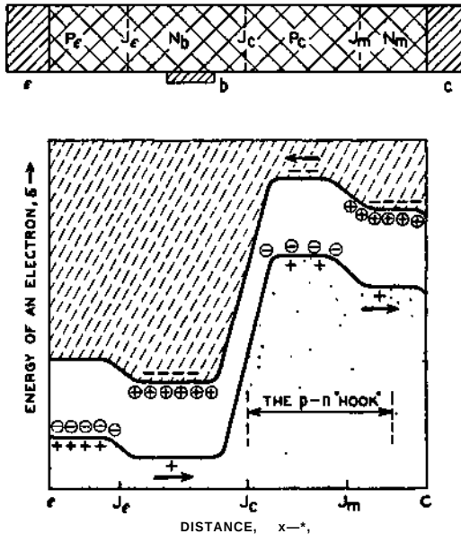
FIG. 4-13—The "p-n Hook" as a Current Multiplier.
