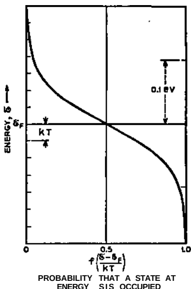
FIG. 10-1—Fermi-Dirac Distribution Function.
