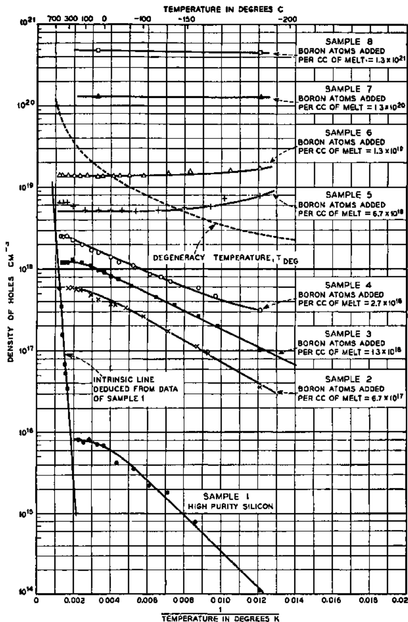
FIG. 11-8—Density of Holes in Silicon-boron Alloys versus Temperature.
