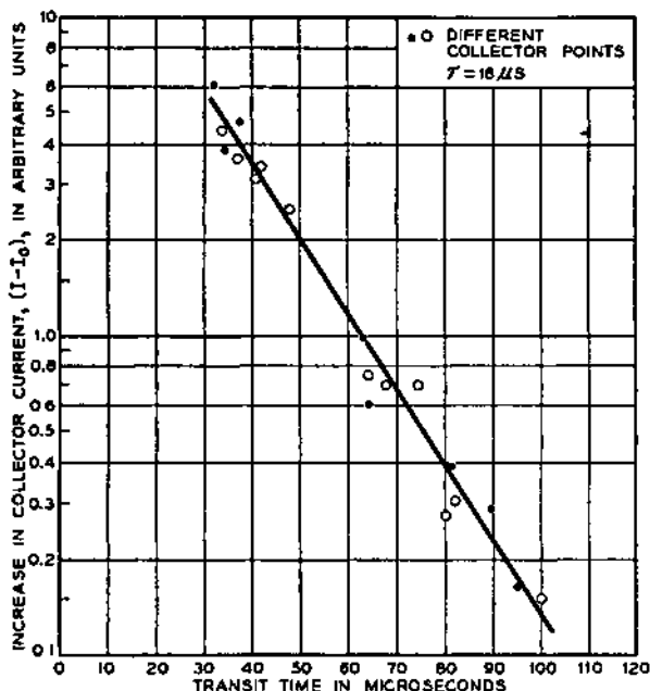
FIG. 3-8—The Decay of Injected Holes in a Sample of w-Type Germanium.
