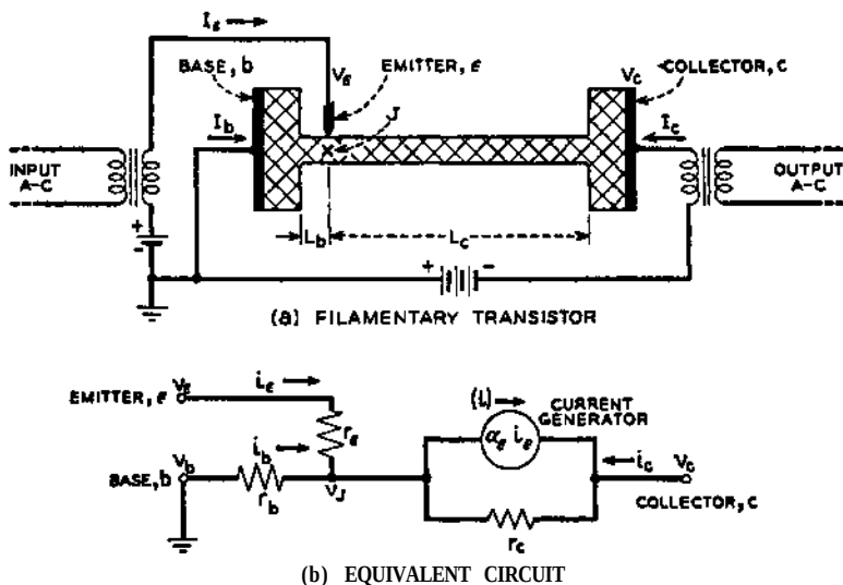
FIG. 4-1—Filamentary Transistor and Equivalent Circuit.
