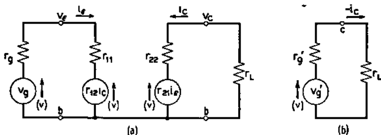
FIG. 2-8—The Transistor as a Grounded Base Amplifier.
