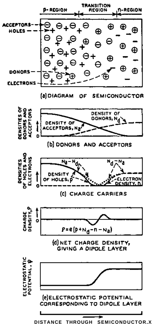
FIG. 4-3—The p-n Junction.
