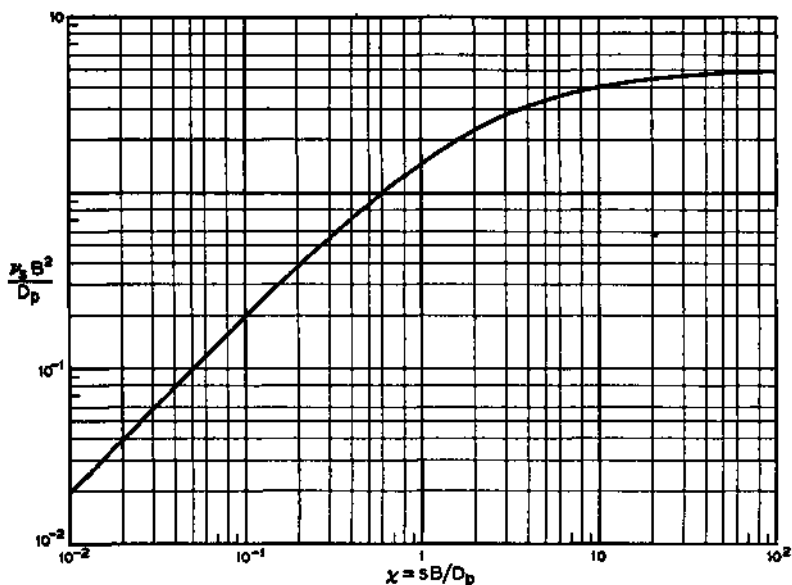
FIG. 12-6—The Dependence of the Surface Decay Constant v_0 upon the Surface Recombination Velocity s .
