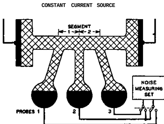
FIG. 12-12—Montgomery's Noise Transmission Effect.
