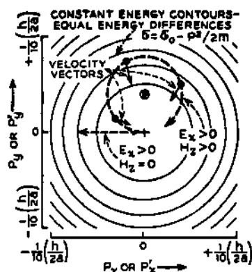
(b) CHANGE IN QUANTUM STATE OF AN ELECTRON INITIALLY AT THE STATE OF HIGHEST ENERGY
