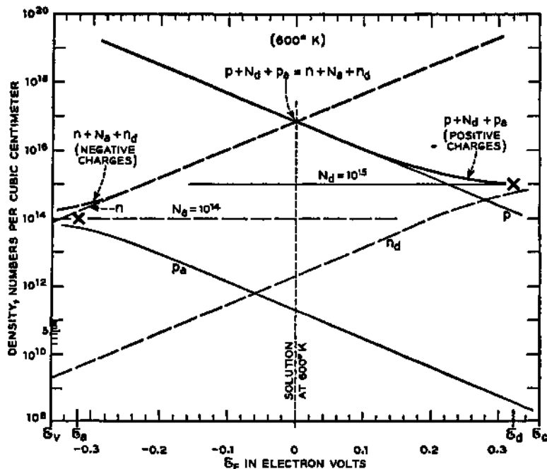
FIG. 16-3—Solution for E_F with Density Acceptors, N_a = 10^{14} \text{ cm}^{-3} , Density of Donors, N_d = 10^{15} \text{ cm}^{-3} and T \cong 600^\circ \text{K} .
