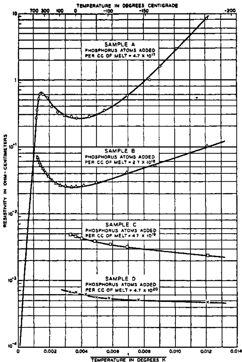
FIG. 1—10—Resistivity of Silicon-Phosphorous Alloys Versus Temperature.
