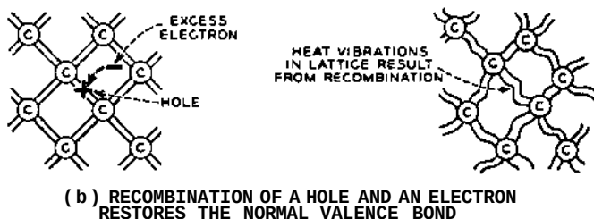
FIG. 1-6—Photo-conductivity in Diamond.
