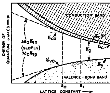
FIG. 17-5—Variation of Energy with Lattice Constant.
