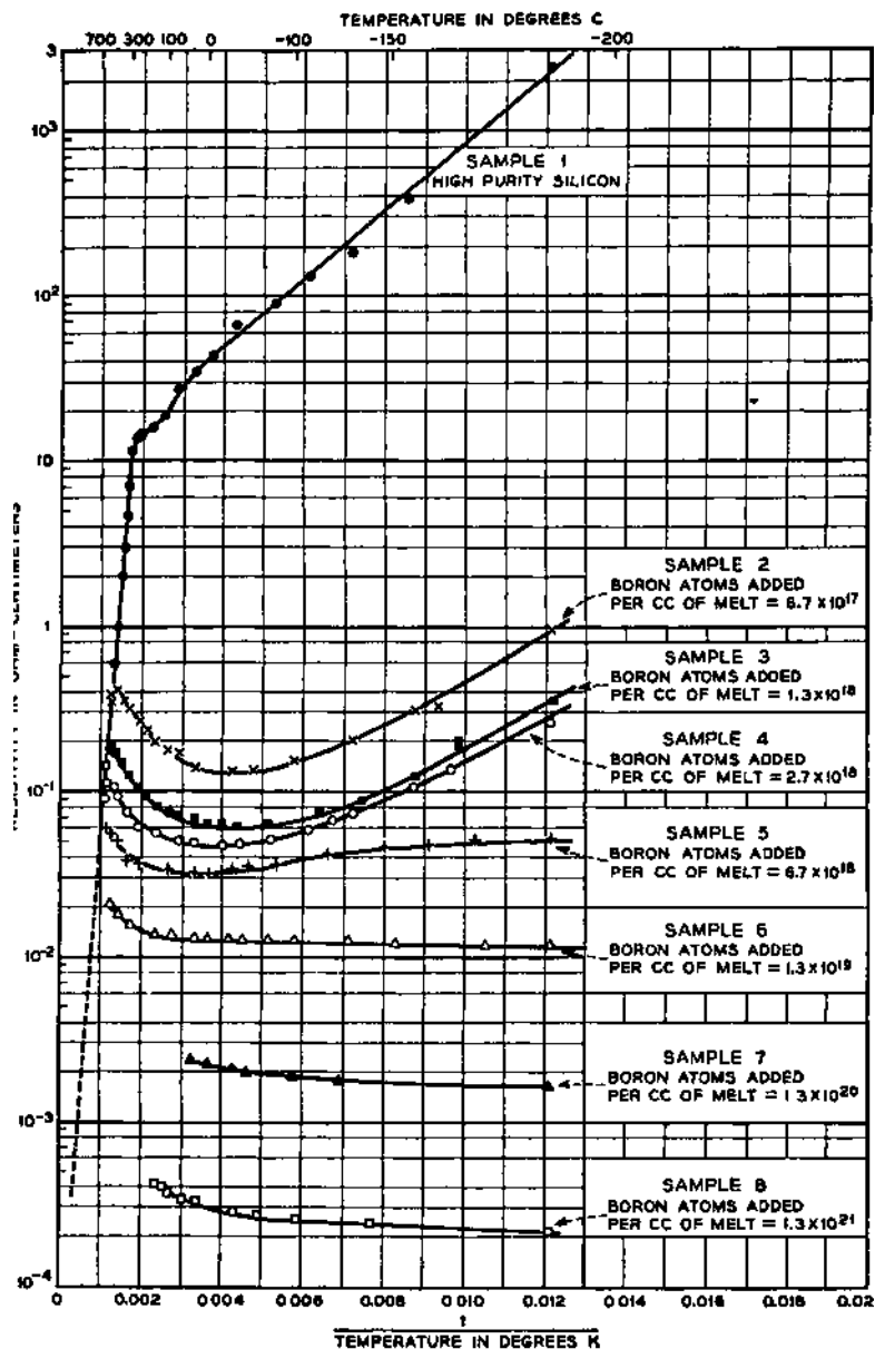
FIG. 11-7—Resistivity of Silicon-boron Alloys versus Temperature.
