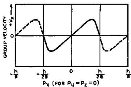
(b) GROUP VELOCITY FOR THE UPPER ENERGY BAND
