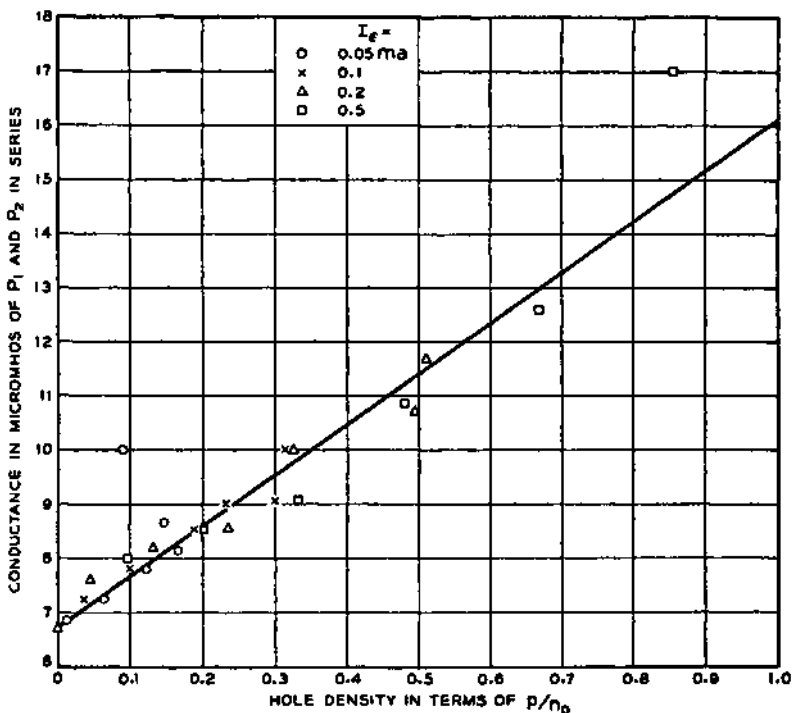
FIG. 3-7—Conductance of P_1 and P_2 of Figure 3-3 in Series as Function of p/n_0 Showing that Conductance Depends on Hole Concentration but Not on Currents in Filament. For Each Value of I_c the Hole Density Was Varied by Varying I_b + I_c from .038 to .078 ma.
