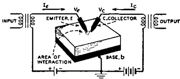
(a) TYPE-A TRANSISTOR
