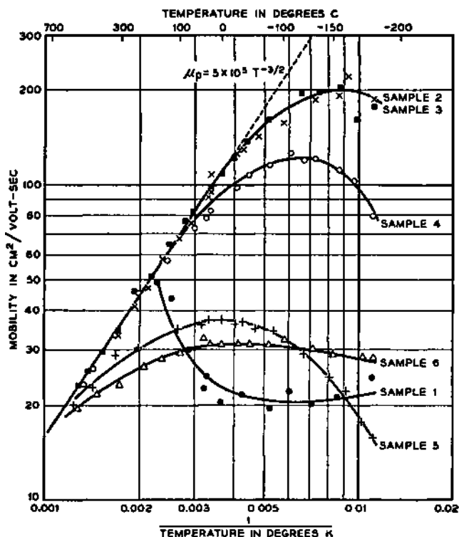
FIG. 11-10—Hole Mobility in Silicon-boron Alloys versus Temperature.
