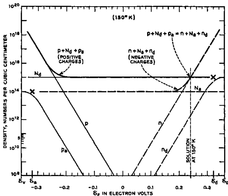
FIG. 16-4—Solution for \mathcal{E}_F with Density of Acceptors, N_a = 10^{14} \text{ cm}^{-3} , Density of Donors, N_d = 10^{16} \text{ cm}^{-3} and T \approx 150^\circ\text{K} .
