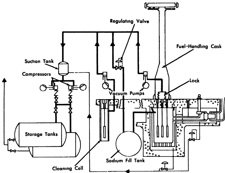
FIG. 6-27. Gaseous-waste system.
