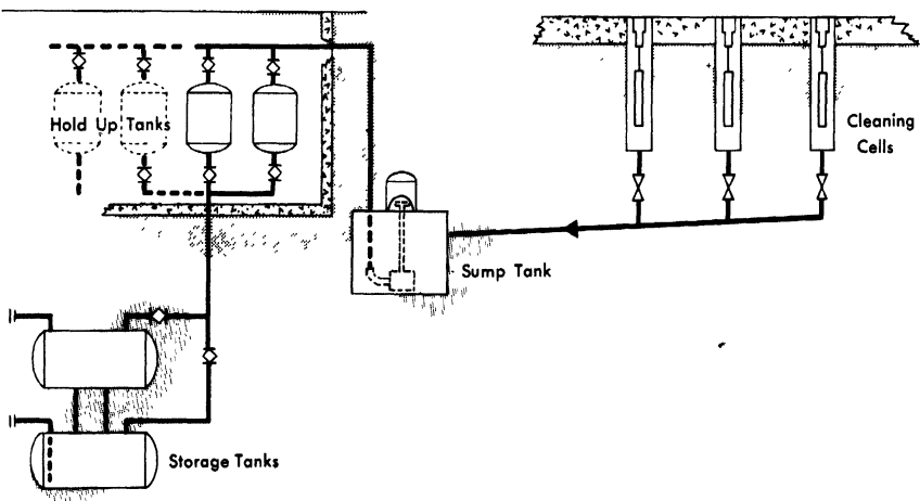
FIG. 6-26. Liquid-waste system.
