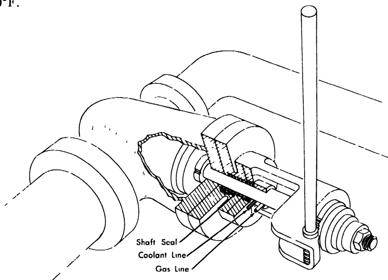
FIG. 6-12. SRE valve.
