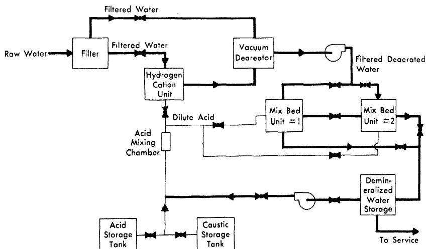
FIG. 7-3. SRE water-conditioning system flow diagram.
