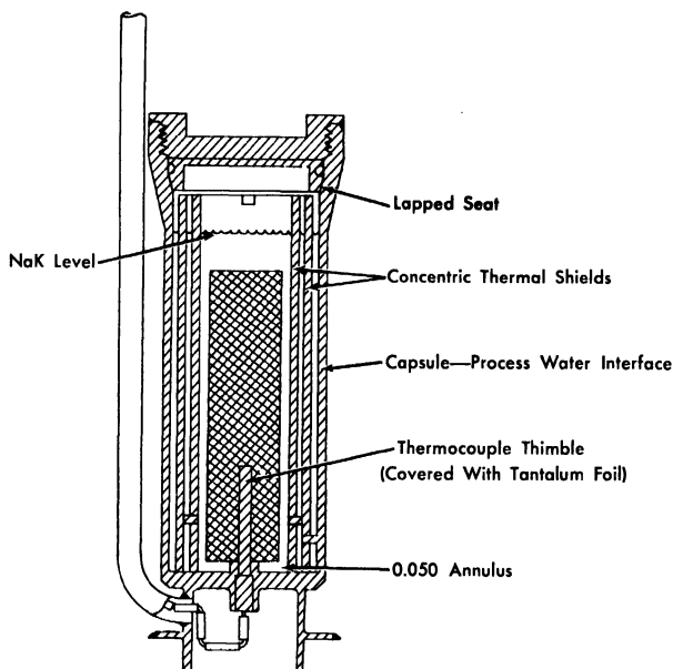
FIG. 5-8. Fuel slug irradiation capsule.
