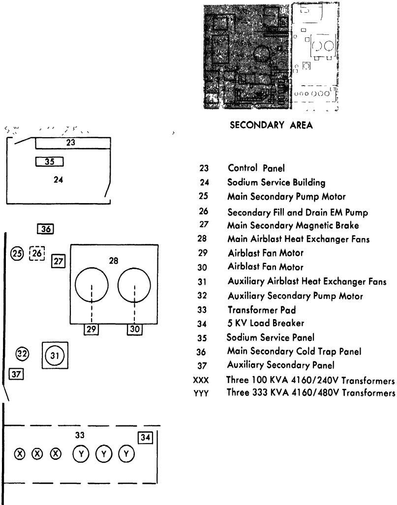
FIG. 6-37(c). Secondary area.
