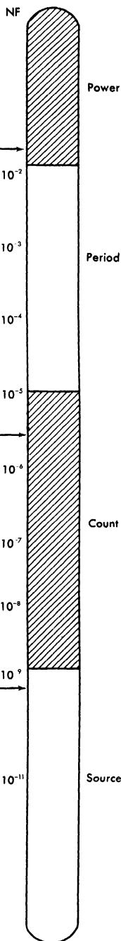
FIG. 6-32. Relation of neutron flux level to instrumentation and control.
