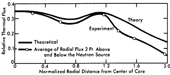
FIG. 3-10. Radial thermal flux plot of dry SRE.
