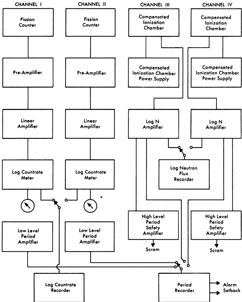
FIG. 6-29. SRE nuclear instrumentation, channel I-IV.
