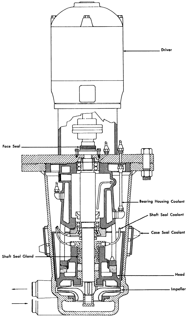
FIG. 6-13. SRE secondary sodium pump.
