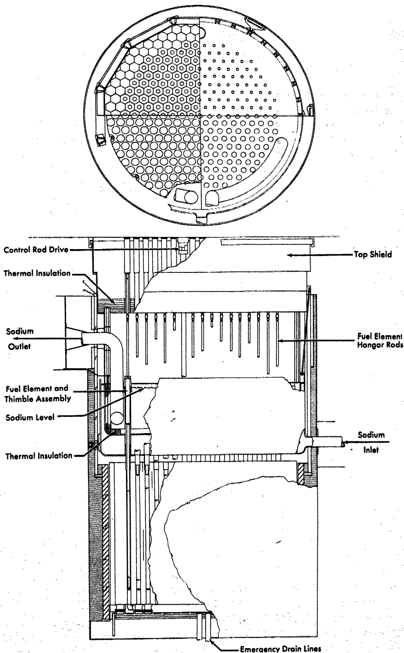
FIG. 8-10. Thimble core.
