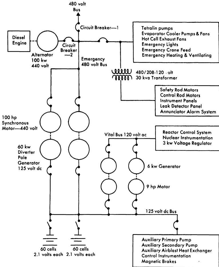
FIG. 6-35. Emergency electrical power system diagram.
