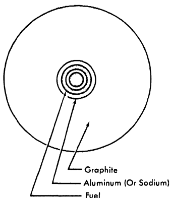
FIG. 3-2. Five-region model of the lattice cell.
