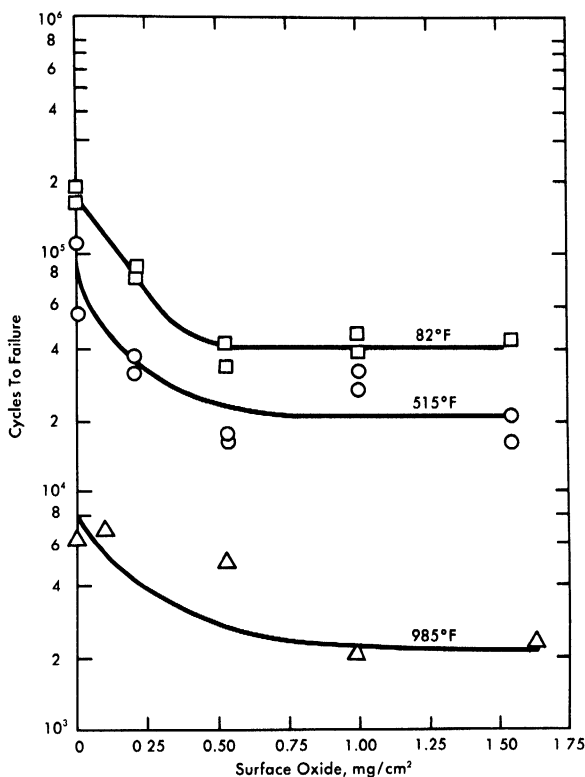
FIG. 4-3. Fatigue cycles to failure.
