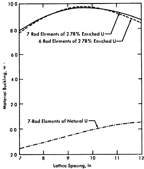
FIG. 3-4. Lattice bucklings measured in the sodium graphite exponential experiment.
