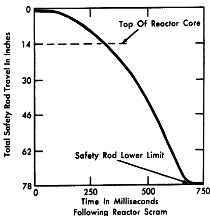
FIG. 6-31. Safety-rod response time following release from holding magnet.
