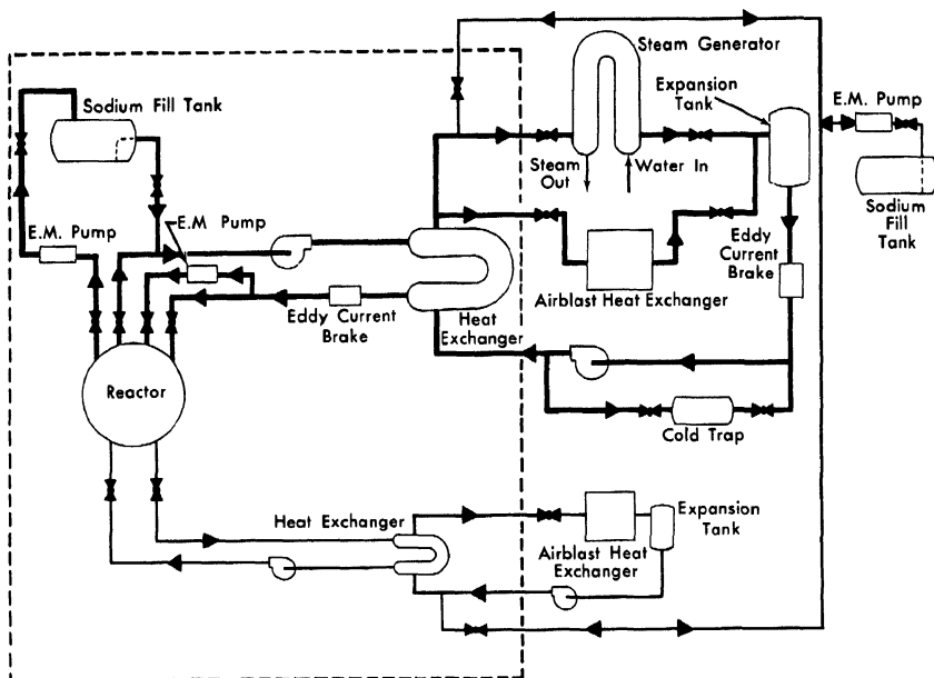
FIG. 6-11. SRE coolant system schematic (the area to the left enclosed by the dotted line represents the radioactive portion of the sodium system).
