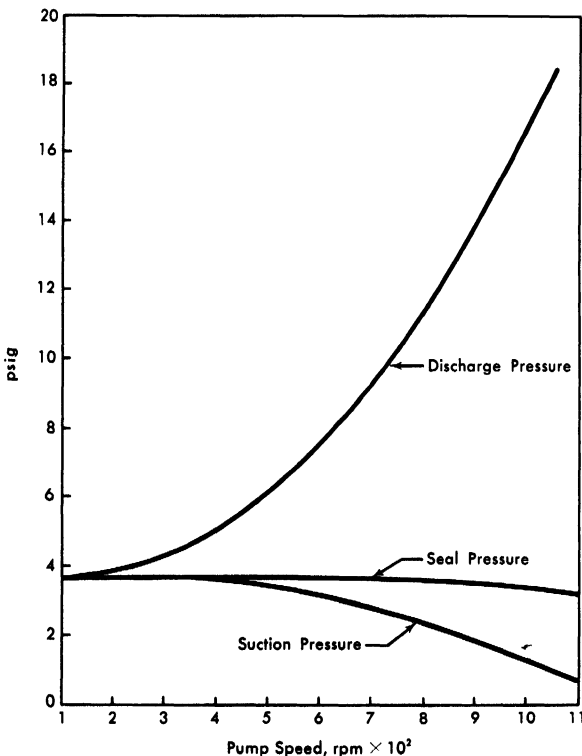
FIG. 7-4. Main primary pump pressure versus rpm.
