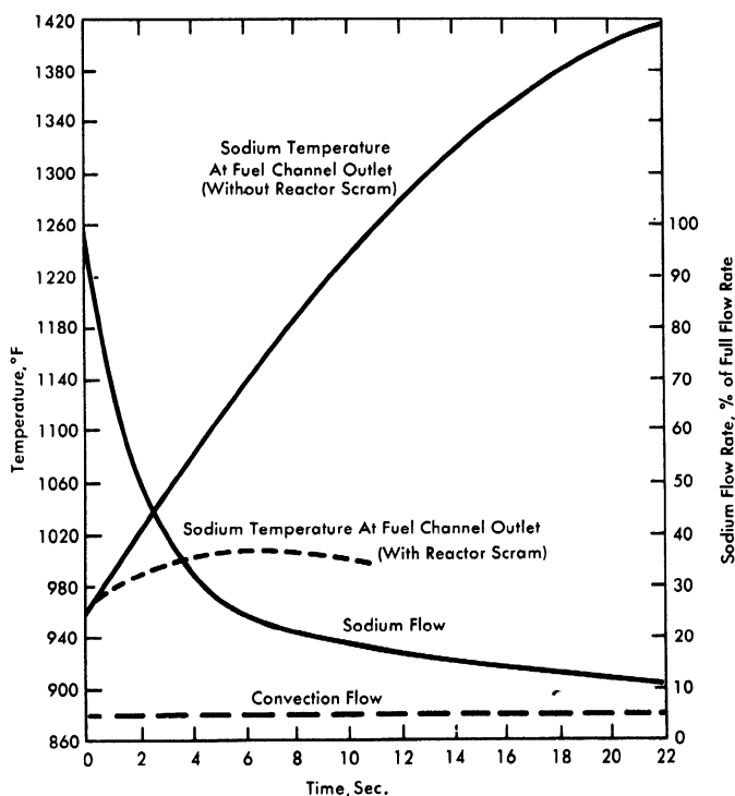
FIG. 3-20. SRE loss of sodium flow accident (with and without corrective action).
