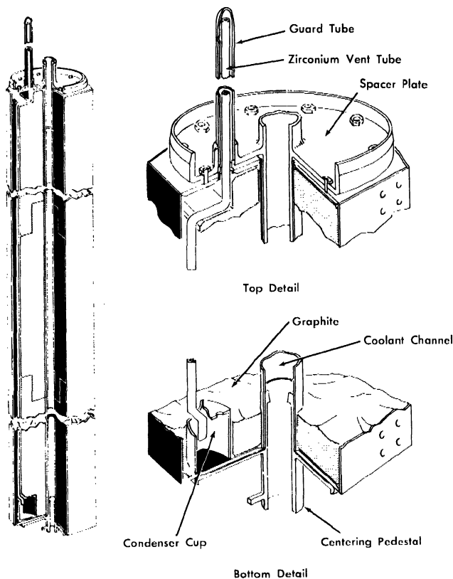
FIG. 6-6. Moderator can details.
