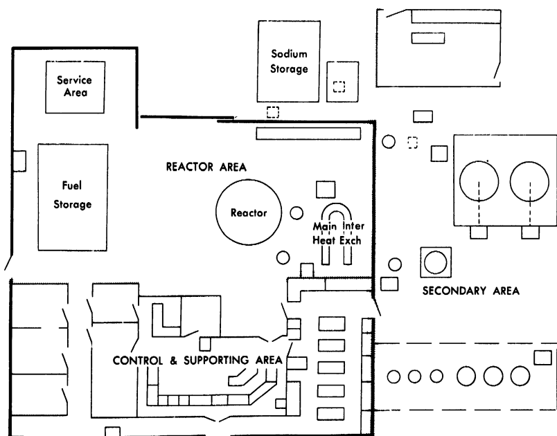
FIG. 6-37. Floor plan of reactor building.
