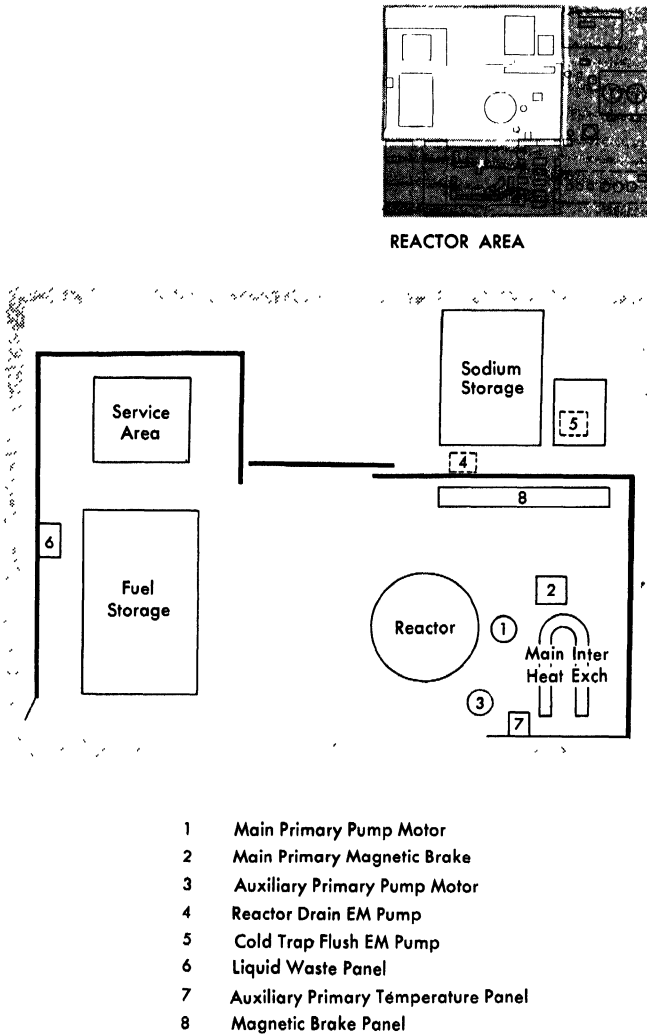
FIG. 6-37(a). Reactor area.
