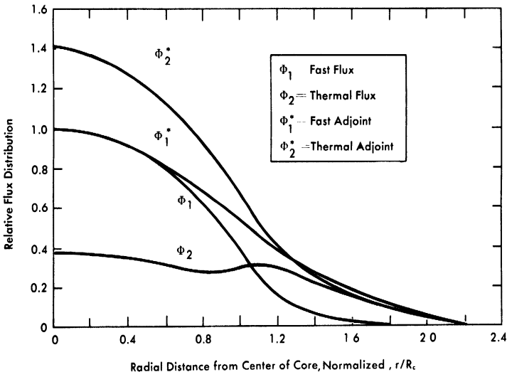
FIG. 3-12. Neutron flux for SRE, wet case.
