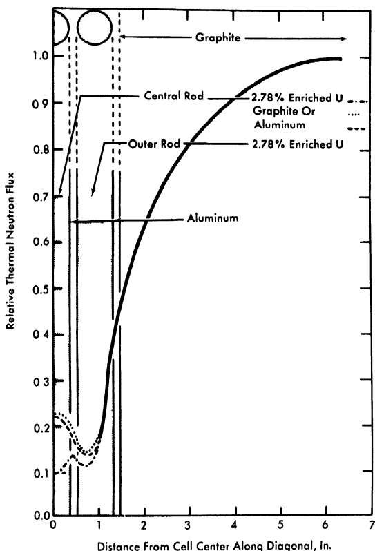
FIG. 3-5. Flux distribution measurements.
