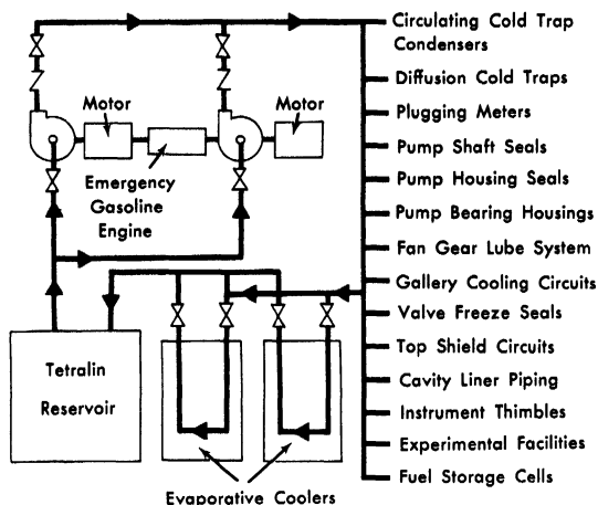
FIG. 6-25. Organic cooling system.
