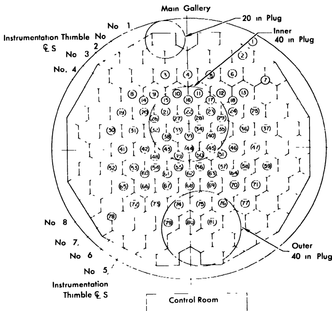
FIG. 6-5. Loading face top surface.
