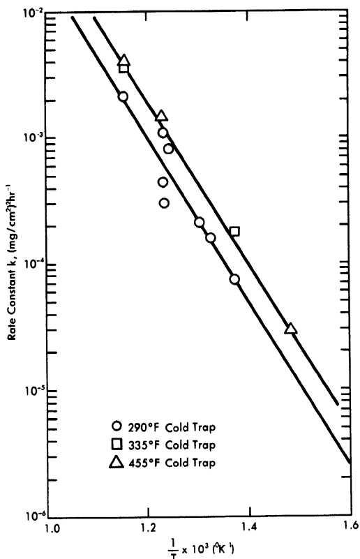
FIG. 4-2. Weight-gain rate data for reactor-grade zirconium in liquid sodium.
