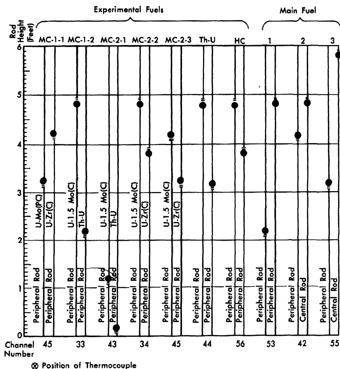
Fig. 5-5. Thermocouple distribution in the SRE.
