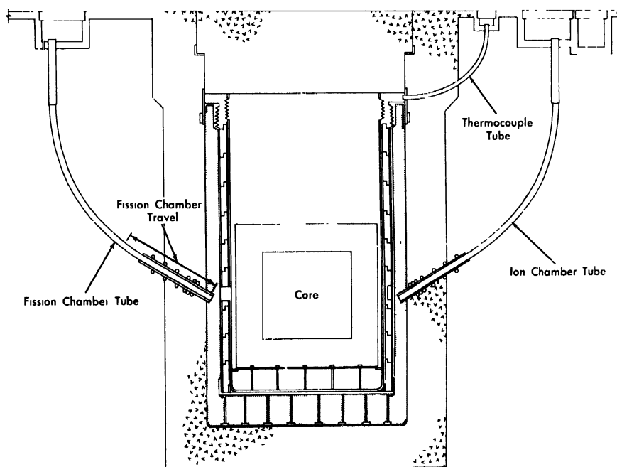
FIG. 6-28. Instrumentation tubes providing access to the reactor core.
