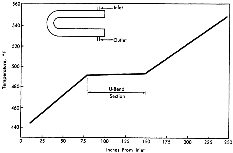
FIG. 7-9. Main intermediate heat-exchanger temperatures during steady-state operations.
