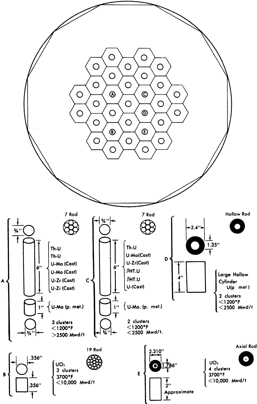
FIG. 5-3. SRE experimental program.
