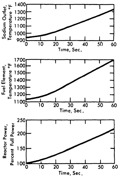
FIG. 3-18. SRE rod withdrawal transient (simultaneous withdrawal of all shim rods with no corrective action).
