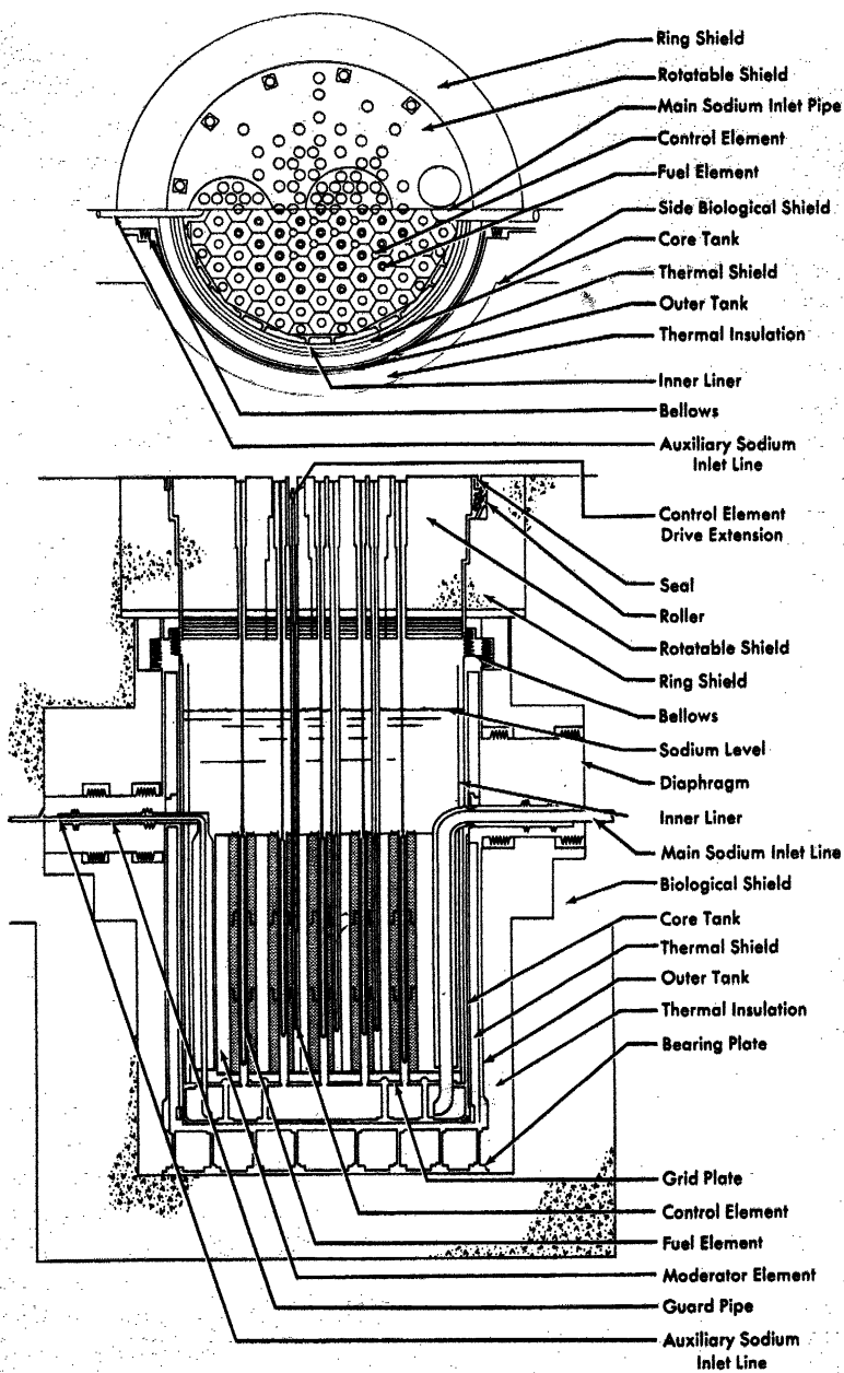
FIG. 2-2. SRE core section and top shield layout with cutaway.
