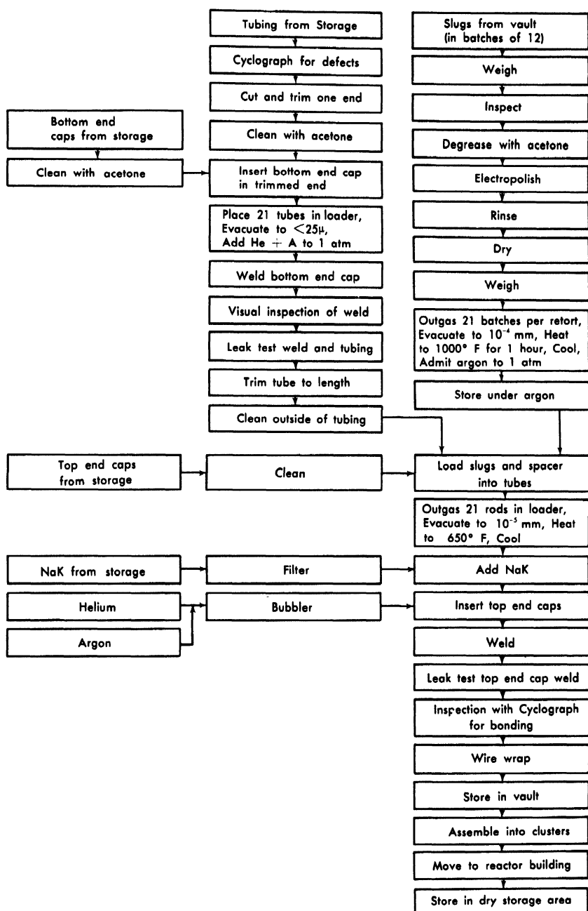
FIG. 5-11. Flow chart of SRE fuel-rod fabrication.
