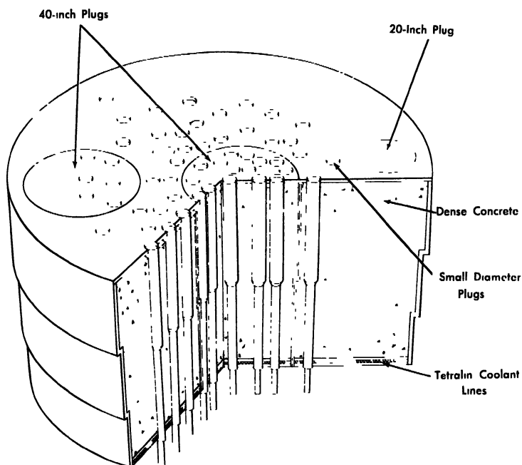
FIG. 6-4. Loading face shield.
