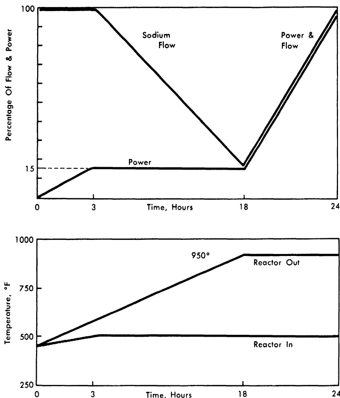
Fig. 7-6. Typical cold-start procedure for the SRE.
