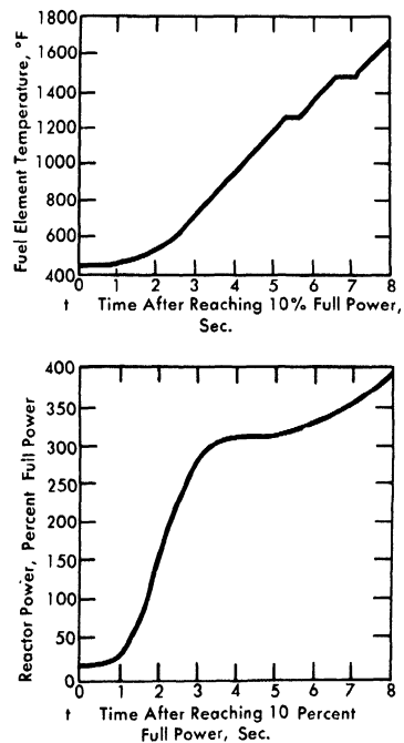
FIG. 3-19. SRE startup accident (simultaneous withdrawal of all shim rods from shutdown condition with no corrective action).
