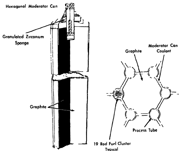
FIG. 8-6. Proposed HINPF moderator and reflector cans.
