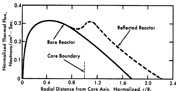
FIG. 3-13. Radial flux (wet) with black control rod on axis.
