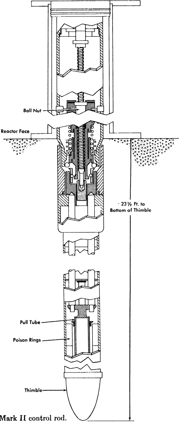
FIG. 6-8. Mark II control rod.
