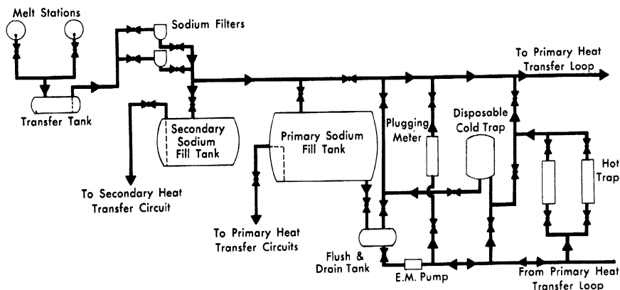
FIG. 6-19. Schematic of sodium service system.
