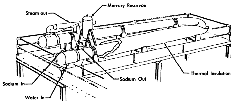
FIG. 7-1. SRE steam generator.
