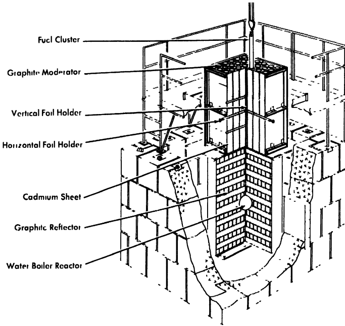
FIG. 3-3. Sodium graphite exponential experiment.
