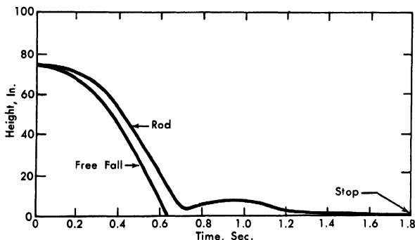
FIG. 6-10. Safety-rod drop, position versus time.
