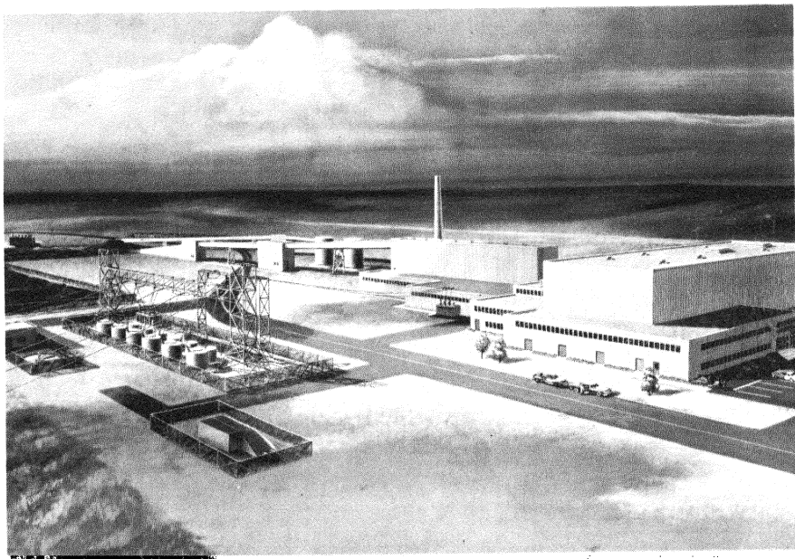
FIG. 8-2. A preliminary study of the proposed HNPf site arrangement looking toward the northeast. In the right foreground is the nuclear facility housing the reactor, steam generators, and the sodium heat-transfer system and services. The building to the left of the nuclear facility houses a coal-fired steam boiler and its turbine-generator unit.
