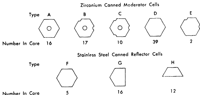
FIG. 6-7. Variations of the hexagonal shape used on moderator/reflector cans.
