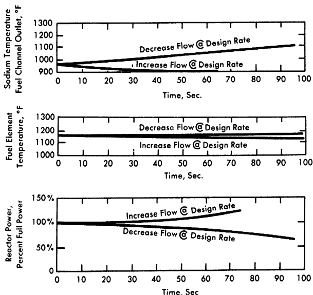
FIG. 3-21. SRE sodium flow transients (no corrective action).
