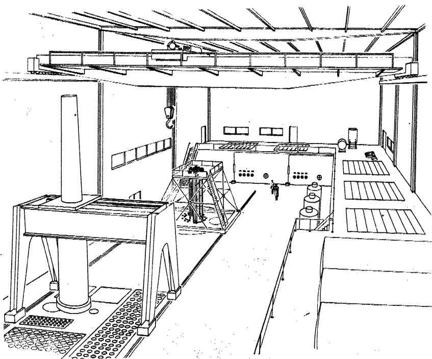
FIG. 8-3. A preliminary study of the reactor room. Visible on the second level are the removable shield blocks over the three intermediate heat exchangers. In the center foreground, at floor level, can be seen the outline of the top shield or loading face of the reactor. Above the loading face is a supporting structure for the control and safety-rod drives. This structure unitizes the removal and handling of the drives when the face is cleared for refueling.
