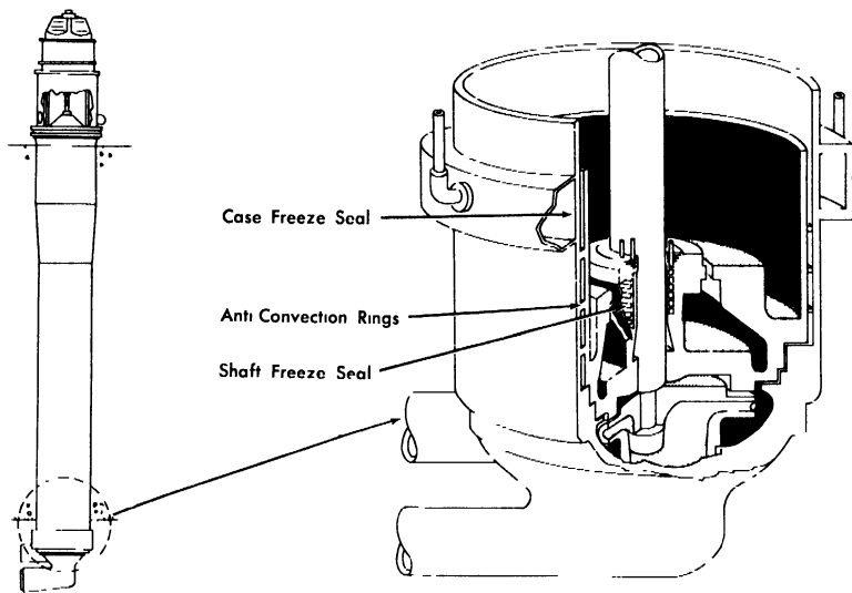
FIG. 6-14. SRE main sodium pump (cutaway of lower portion of pump, showing freeze seals).
