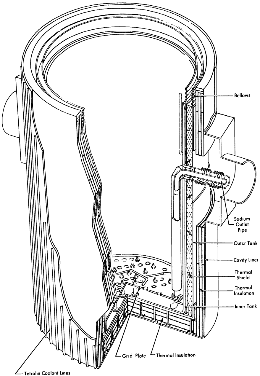
FIG. 6-2. Core containment cutaway.
