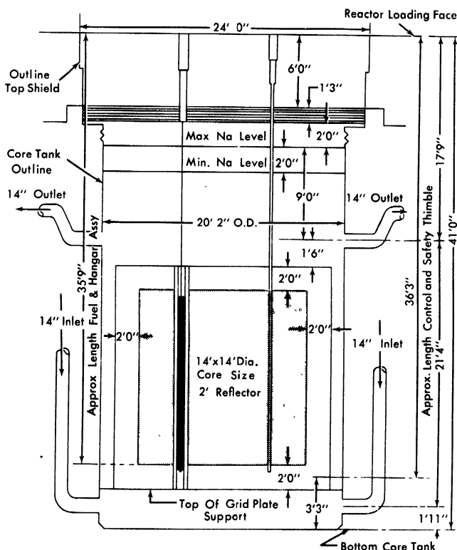
FIG. 8-5. Tentative reactor outline dimensions.
