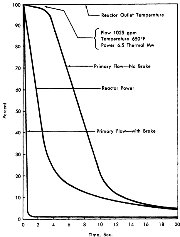
FIG. 7-7. Post-scam sodium flow from 150°F \Delta T .
