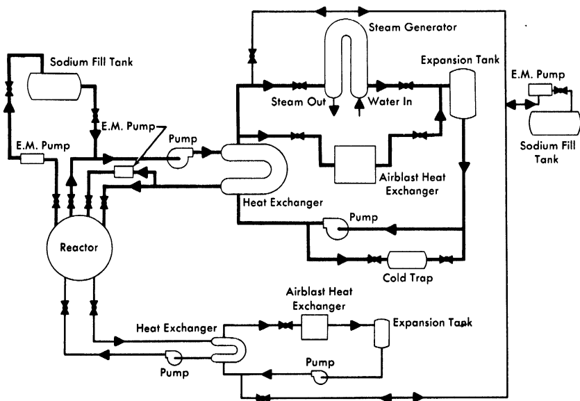
Fig. 2-3. SRE coolant flow diagram.
