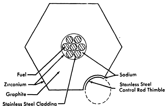
FIG. 3-7. SRE lattice cell.
