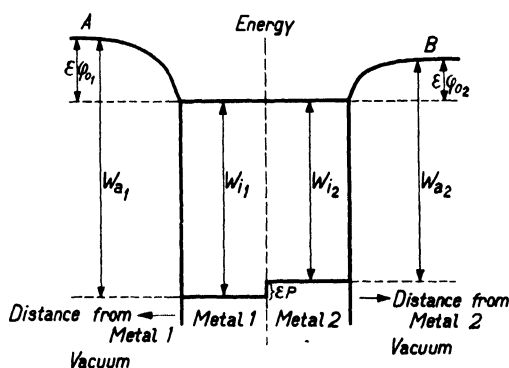
Fig. 9. Relative height of energy levels, when two metals are in contact with each other.
