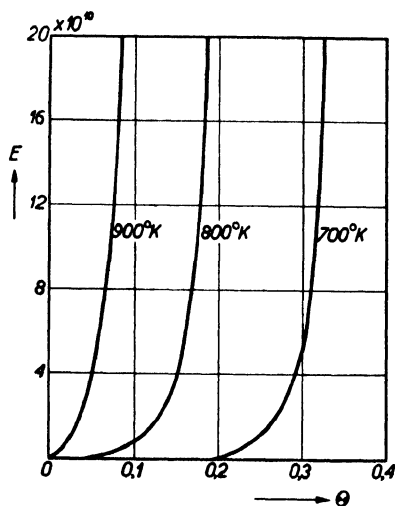
Fig. 28. Rate of evaporation of Cs atoms per cm. 2 per sec., E_a , from a tungsten filament as a function of \theta .
