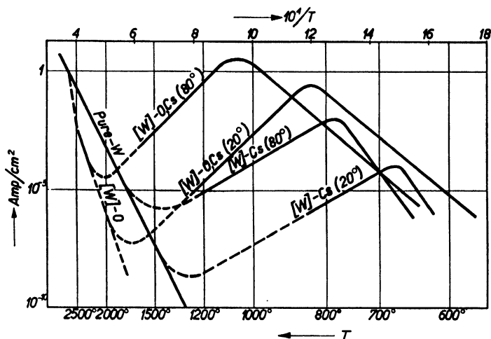
Fig. 62. Electron emission as a function of temperature for [W]-O,Cs and [W]-Cs cathodes at Cs vapour pressures corresponding to a bulb temperature of 20 and 80° C. Figure taken from I. Langmuir, Industr. Engng Chem. 22 , 390 (1930).
