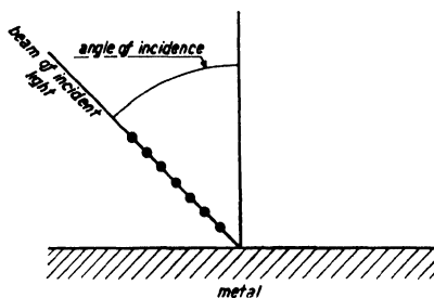
Fig. 48b. Electric vector of the incident light perpendicular to the plane of incidence. \perp .
