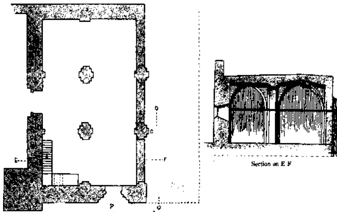
PLAN AND SECTION OF MEDIEVAL CHURCH AT YEBNA, Scale \frac{1}{200} . Hearing 109°.
