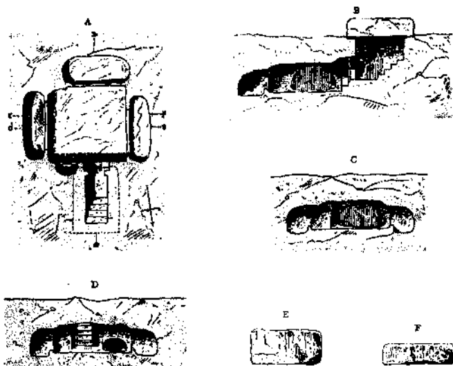
DETAILS OF ROCK-HEWN TOMBS AT K'BUR EL YAHUD. Scale \frac{1}{100} .
