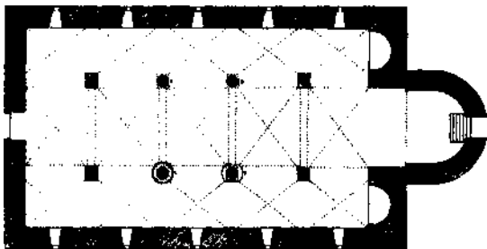
PLAN OF JAMEH EN NASIR, NABLUS. Scale \frac{1}{300} .
