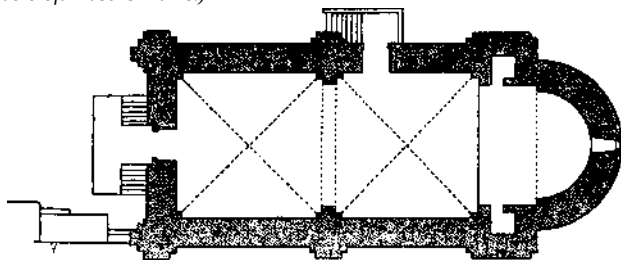
PLAN OF SMALL MEDIAEVAL CHURCH AT GAZA. Scale \frac{1}{16} .
