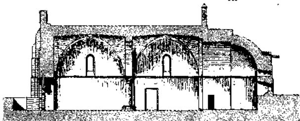
LONGITUDINAL SECTION. Scale \frac{1}{16} .
