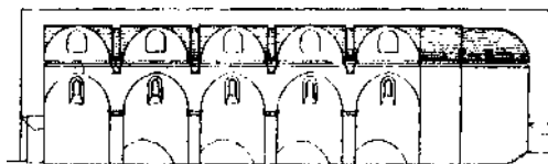
LONGTUDINAL SECTION OF JAME' EN NASER. Scale \frac{1}{300} .
