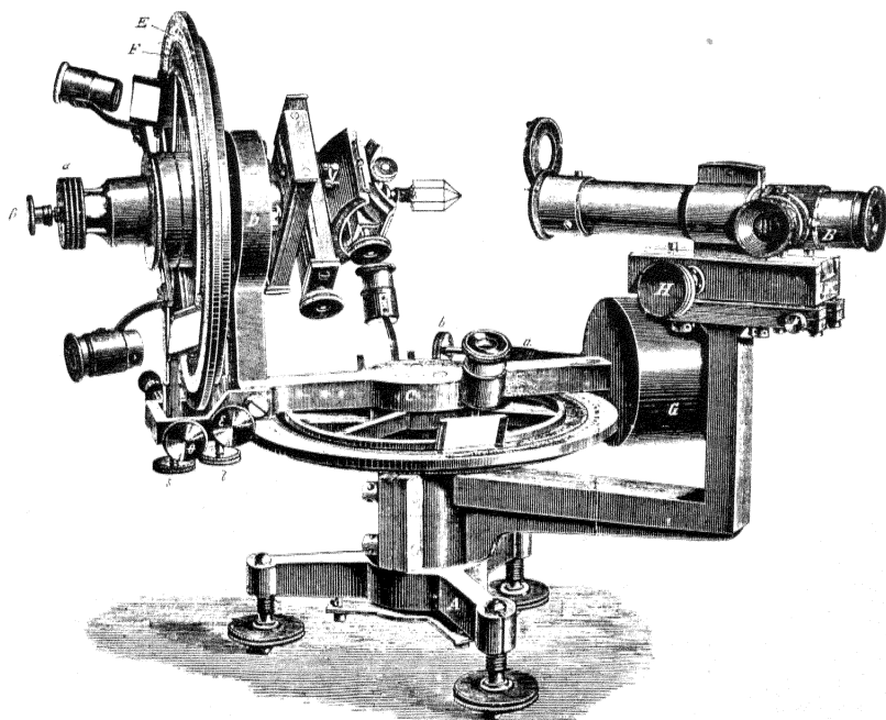
FIG. 45.—THE ORIGINAL FEDOROV TWO-CIRCLE GONIOMETER.
