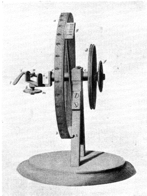
FIG. 41.—WOLLASTON REFLECTING GONIOMETER.
