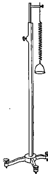
FIG. 25. — Variation of period of vibration with load.
