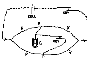
FIG. 107. — Diagram of Wheatstone's bridge in its completed form.
