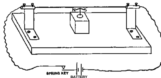
FIG. 87. — Oersted's experiment.
