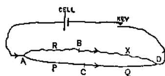
FIG. 106.—Showing how the battery is connected in a Wheatstone bridge, and how the current divides.
