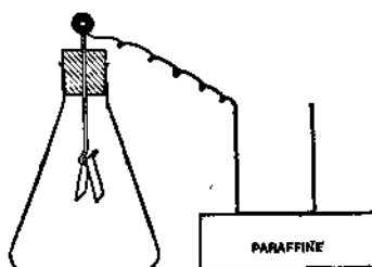
FIG. 83. — Faraday's ice pail experiment.
