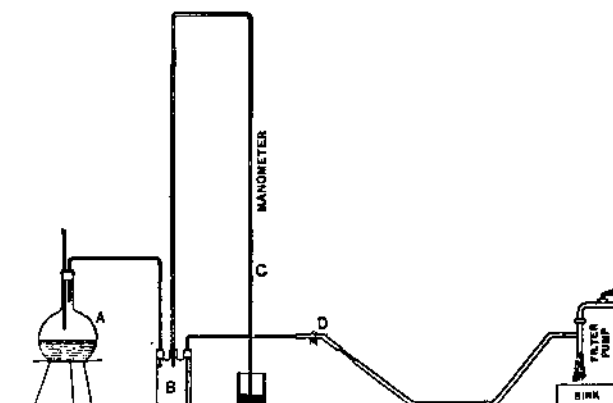
FIG. 74. — Apparatus for showing how the temperature of boiling water varies with the pressure.
