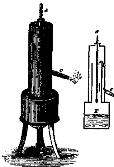
FIG. 67.—Hypsometer, an instrument for heating thermometers to the temperature of boiling water.
