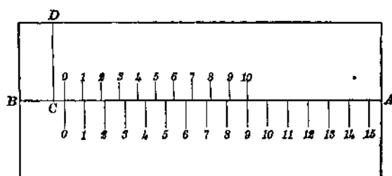
FIG. 6. —Method of making vernier caliper.
