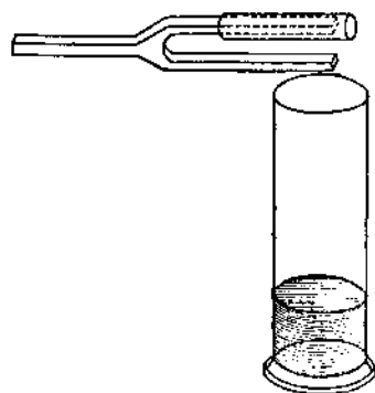
FIG. 60, — Illustrating the fact that two trains of waves are necessary to produce interference.
