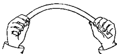
FIG. 80. — Magnetizing a piece of "tin" by bending it in the earth's field.
