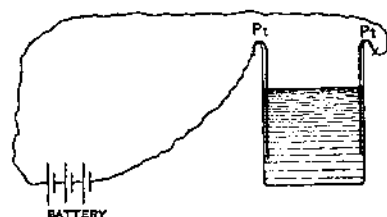
FIG. 96.—Circuit arranged for studying the chemical effects of an electric current.
