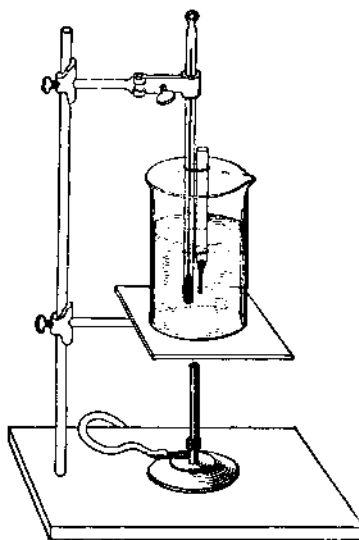
FIG 73-Melting-point of paraffin,
