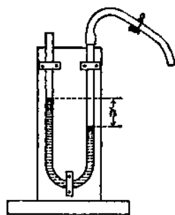
FIG. 39. — A simple form of pressure gauge.
