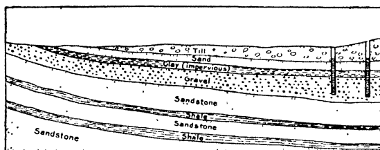
FIG. 153. — Section in water-bearing gravel with intake too low to cause water to rise to the surface. (After Ellis.)
