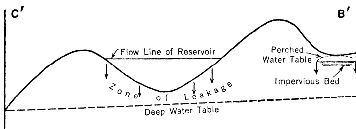
Fig. 196c. — Section showing relation of reservoir level to low water table. (After Bryan, U. S. Geol. Surv., Wat. Sup. Pap. 597.)
