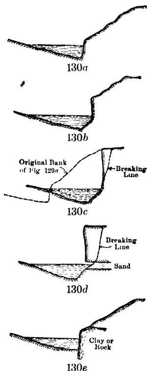
FIG. 130. — Sections showing successive stages of bank erosion. (a) Initial condition of bank; (b) erosion in progress; (c) bank cut back to vertical; (d) saturated basal sand layer, whose outflow leaves bank unsupported; (e) profile developed with hard rock or tough clay. (From Thomas and Watt, Improvement of Rivers. )
