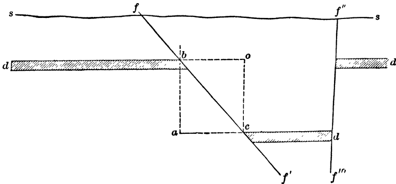
Fig. 90. — Normal fault in horizontal beds. ss , surface; ff' , fault plane; db , up-throw side; dc , downthrow side; cba , angle of hade or slope; cbo , angle of dip; ab , throw (also stratigraphic throw in this case); ac , heave (horizontal throw); left side of ff'' , foot wall; right side of ff'' , hanging wall; fbc , fault scarp; f''f''' , fault plane (vertical).
