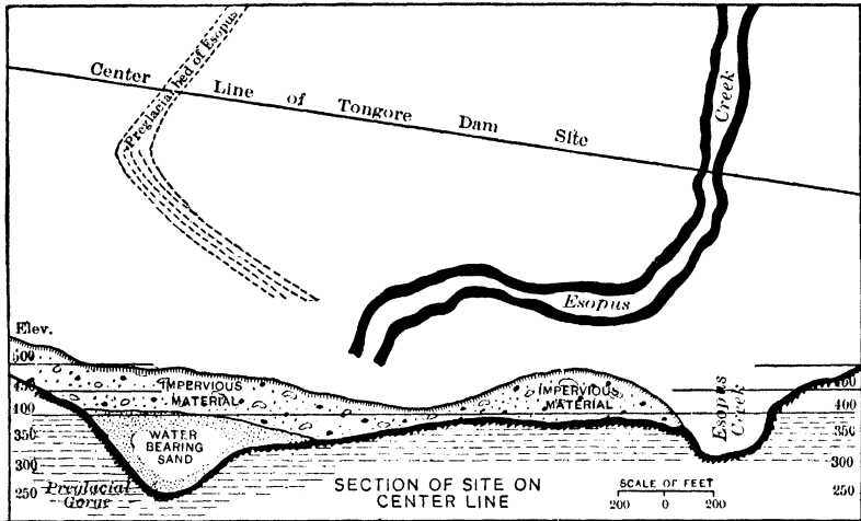
FIG. 195. — Section through Tongore dam site, tested for Catskill, N. Y., aqueduct. (After Berkey, N. Y. State Museum, Bull. 146.)
