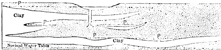
FIG. 148. — Conditions encountered by wells sunk through perched water tables. (After Fuller, U. S. Geol. Survey, Water Sup. Pap. 258, 1911.)
