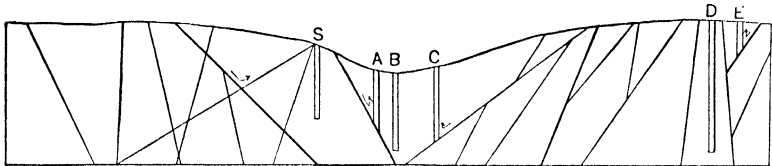
FIG. 157. — Section illustrating artesian conditions in jointed crystalline rocks without surface covering. A, C, flowing wells fed by joints; B, intermediate well of greater depth between A and C, but with no water; D, deep well not encountering joints; E, pump well adjacent to D, obtaining water at shallow depths; S, dry hole adjacent to a spring, showing why wells near springs may fail to obtain water. (From Fuller, U. S. Geol. Survey, Bull. 319.)
