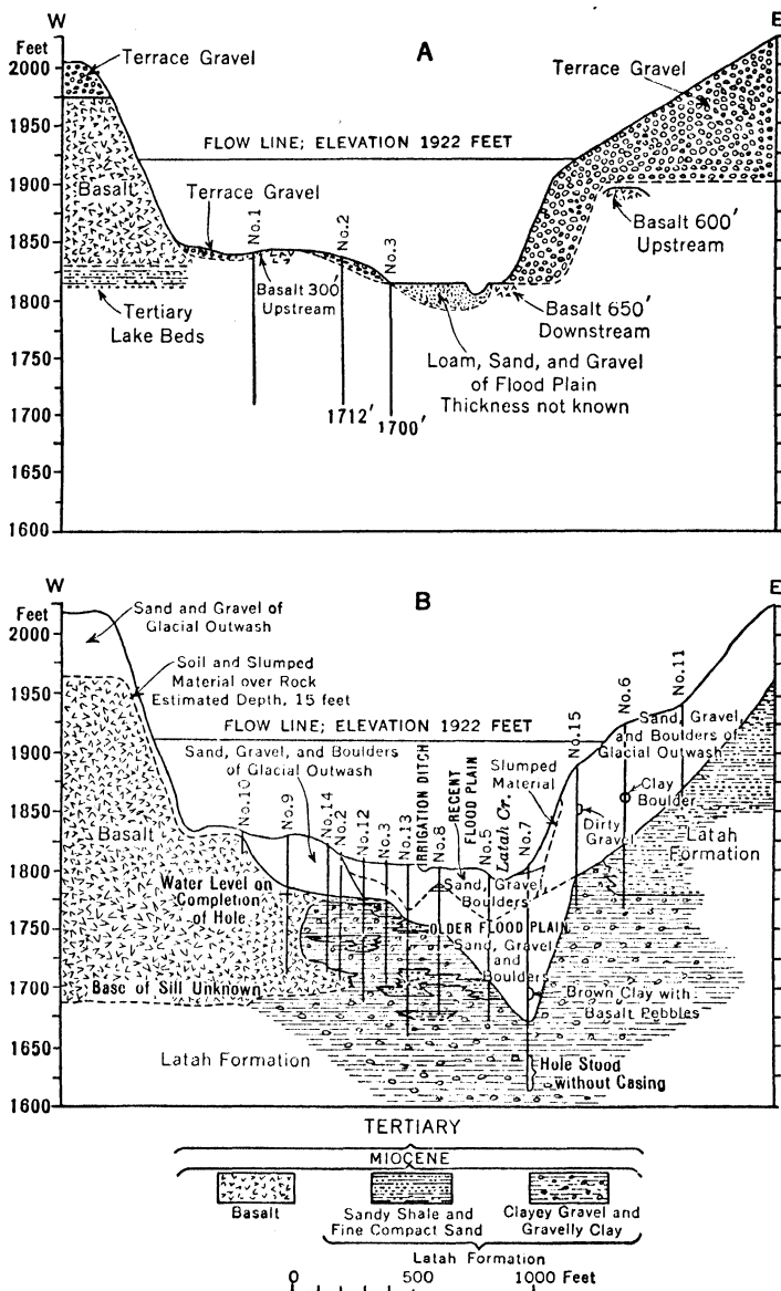
FIG. 196i. — Geologic section of Latah Creek dam site, Columbia basin irrigation project, Washington. A , showing known and inferred relations; B , based on completed examination and results of test drill holes. (After Bryan, U. S. Geol. Surv., Wat. Sup. Pap. 597-A, 1929.)
