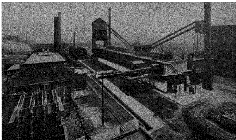
PLATE LXXXII, FIG. 2. — By-product coke ovens.
