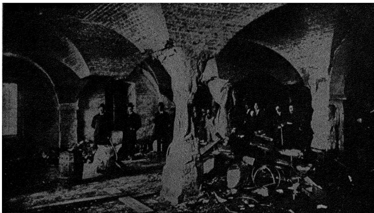
FIG. 198.—Effect of fire on granite columns, U. S. Public Storehouse, Baltimore, Md.
