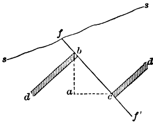
FIG. 91. — Normal fault having against dip of beds. ab , throw (vertical); bc , stratigraphic throw; others same as Fig. 90.
