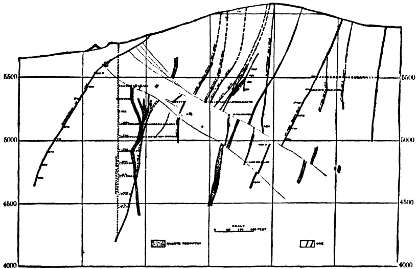
FIG. 220. — Section across veins of Pennsylvania, Rarus, Mountain View, and West Colusa mines, Butte, Mont. A series of steeply dipping veins, broken by faults. (After Weed.)
