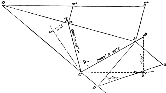
FIG. 104. — Diagram illustrating determination of dip of fault plane. (After Hayes.)
