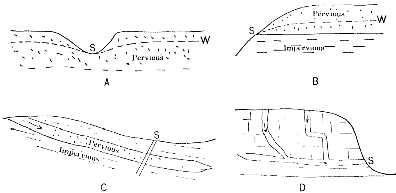
Fig. 146. - Sections illustrating: A , depression spring; B , contact spring; C , artesian spring; and D , tubular spring. S = spring; W = water table.
