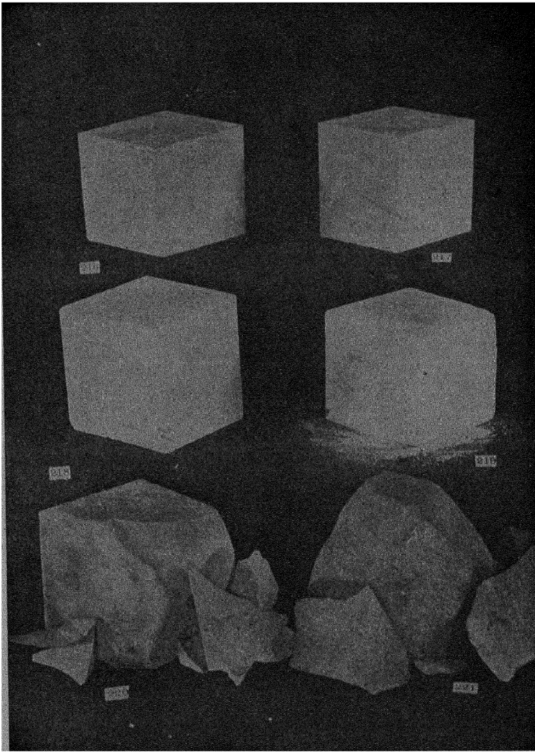
PLATE LXI. — Fire Tests on 3-inch cubes of limestone, Newton, N. J. (After W. E. McCourt.)
