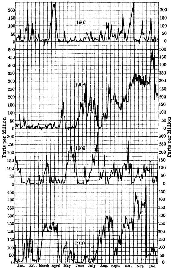
FIG. 135. — Chart showing variation in acidity of Monongahela River water during different years (Pittsburgh Flood Commission report).
