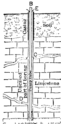
FIG. 163. — Conditions governing freezing in limestone wells. (From Fuller, Domestic Water Supplies.)
