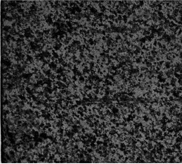
PLATE LXII, FIG. 1. — Moderately fine-grained granite, Hallowell, Me.
