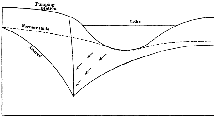
FIG. 142. — Section showing lowering of water table by pumping. (After Veatch, U. S. Geol. Survey, Prof. Pap. 44, p. 72, 1906.)
