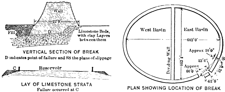
FIG. 168. — Plan and section of Nashville reservoir, showing cause of break. (After Purdue, Eng. Rec., LXVI, p. 539.)
