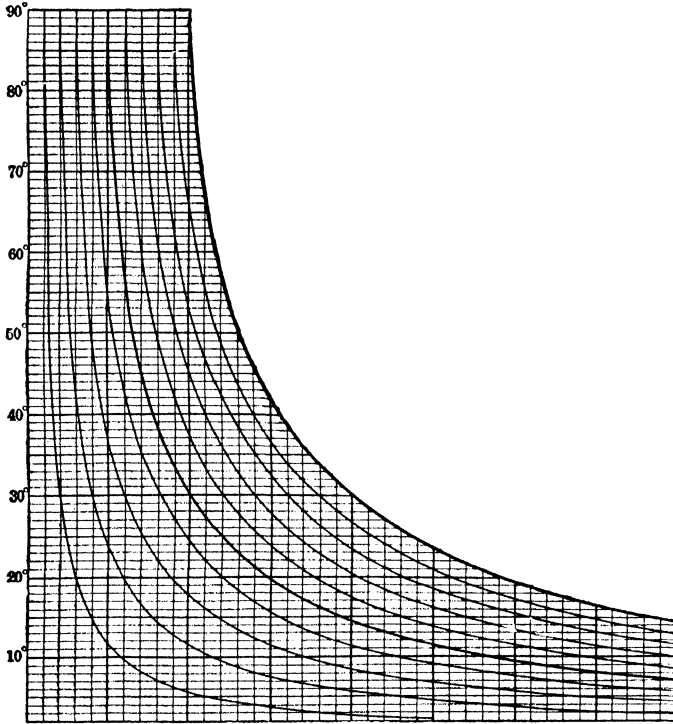
FIG. 83. — Diagram for use in determination of thickness of beds by graphic method. (After Hayes.)
