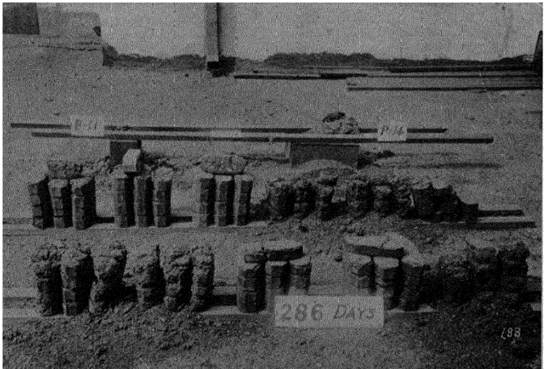
Fig. 2. — The same after 286 days' weathering. (Wright, U. S. Bur. Mines, Bull. 14, 1911.)
