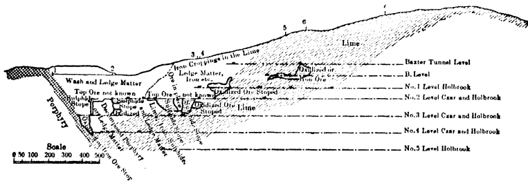
FIG. 222. — Section through Copper Queen mine, Bisbee, Ariz., showing variable depth of weathering. (After Douglas, Amer. Inst. Min. Engrs., Trans., XXIX.)
