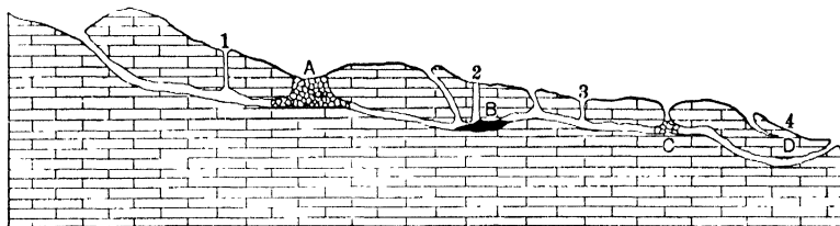
FIG. 154. — Section illustrating conditions of flow from solution passages in limestone. A, brecciated zone (due to caving of roof), serving as confining agent to waters reached by well 1; B, silt deposit filling passage and acting as confining agent to waters reached by well 2; C, surface debris clogging channel and confining waters reached by well 3; D, pinching out of solution crevice resulting in confinement of waters reached by well 4. (After Fuller, U. S. Geol. Survey, Bull. 319, 1908.)
