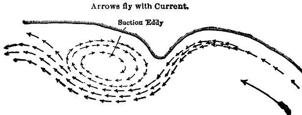
FIG. 128. — Sketch of a suction eddy. (After Thomas and Watt.)
