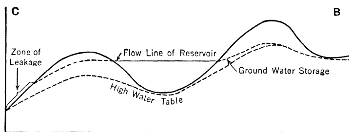
FIG. 196b. — Diagram showing relation of reservoir level to high water table. (After Bryan, U. S. Geol. Surv., Wat. Sup. Pap. 597.)
