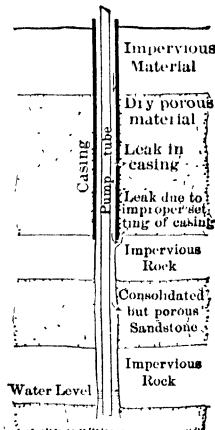
FIG. 162. — Conditions governing freezing in wells with leaky casings and porous walls. (Fuller.)
