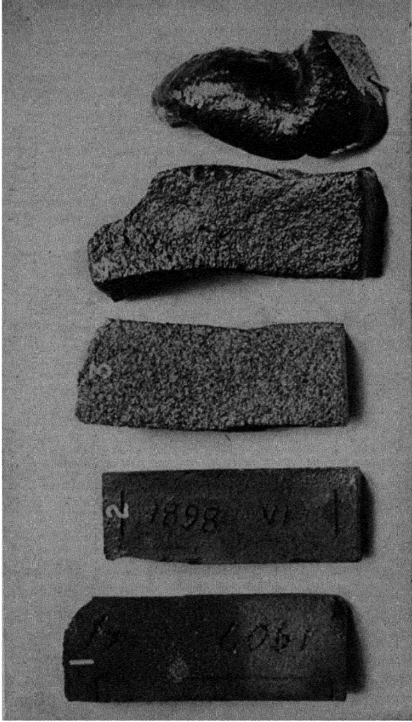
PLATE LXXVI. — Bricklets of different clays, all fired at the same temperature to show their different fusibilities. (529)
