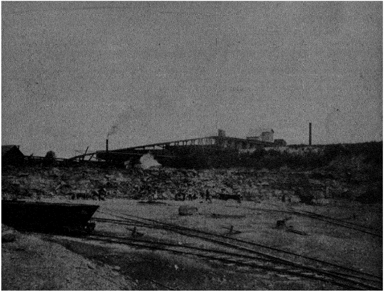
PLATE LXXIV, FIG. 1. — Quarry in natural cement rock, Milwaukee, Wis. (H. Ries, photo.)
