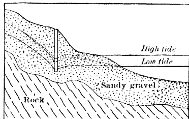
FIG. 152. — Section showing relation of tide to level of water table. (After Ellis.)
