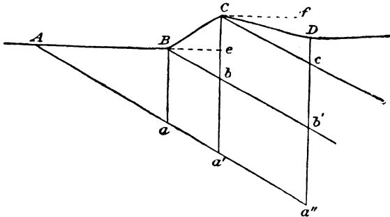
FIG. 85.—Diagram illustrating determination of depth of beds by trigonometric method. (After Hayes.)
