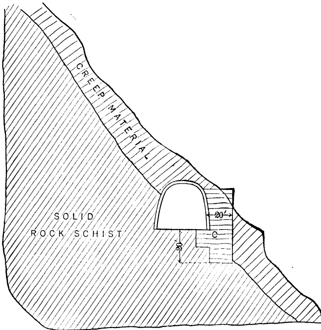
FIG. 169. — Section showing position of Mühlthal tunnel and creep material on Brenner Railroad. (After Drinker, Tunneling.)
