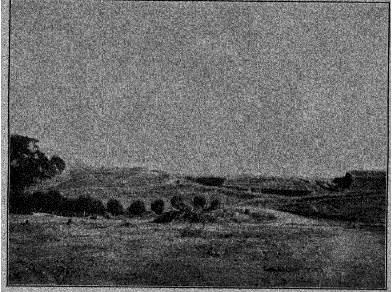
FIG. 196e. — View of Lafayette dam east of Berkeley, Calif. The notch on right shows cut formed by settling of dam due to low bearing power of underlying sediments. (H. Ries, photo.)
