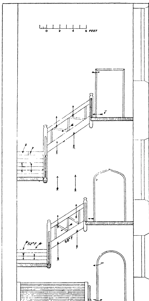
Fig. 15. Diagram showing air currents on the well-staircase of the Cavendish Laboratory. The main features are a warm upward current from a coil of pipes at the foot of the staircase, and a cold stream flowing, from the top story, down the stairs to the basement and thus conducted by the staircase twice round the rising column of warm air.
