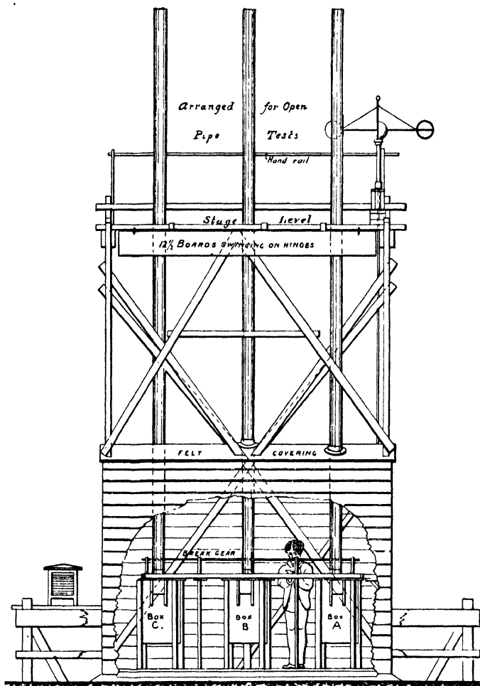
Fig. 4. General view of arrangements by the Cowl Committee of the Sanitary Institute for experiments upon the upcast flow of air caused by wind.
