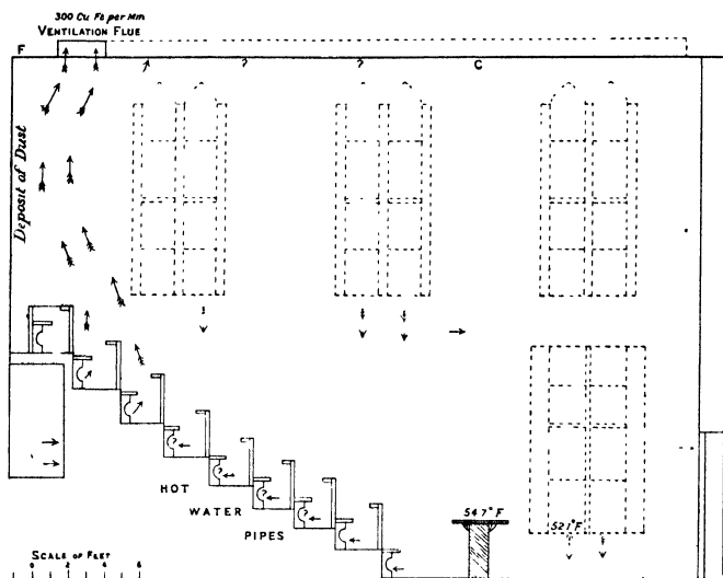
Fig. 14. Diagram showing air currents in the Lecture Room of the Cavendish Laboratory. The strong current shown on the left is a direct convective flow between the hot water pipes under the tiers of seats and the ventilation pipes in the ceiling. The air which supplies this current is derived partly from openings at the back, marked A , and partly by an inflow of air through openings under the lower seats, which were intended to supply the room with air from the warmed space occupied by the pipes. The warming produces a particularly vigorous current through the openings under the two top rows of seats over the hot pipes. Downward convection currents of cold air are also shown by arrows drawn downward from the window-sills. Hardly any indication of flow into the long ventilation flue, which has openings throughout its lower face, was shown, except where the air rose from the heated pipes.
