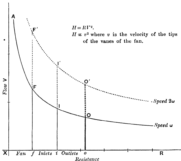
Fig. 34. Ventilation by fan.
