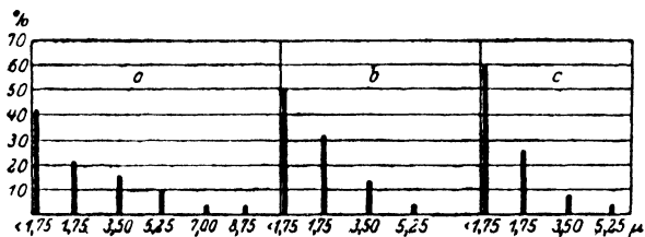
(Standard Nebuliser without condenser, Glycerine water.) a = 1 atmosphere. b = 2\frac{1}{2} atmospheres. c = 5 atmospheres. Ordinate = number of particles per cent. Abscissa = Diameter of particles.
