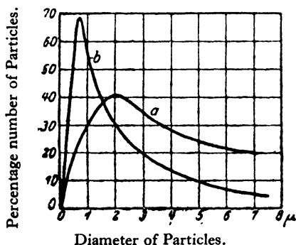
“ Frequency - Curves after Heusser and Strobl. a = Low pressure. b = High.”
