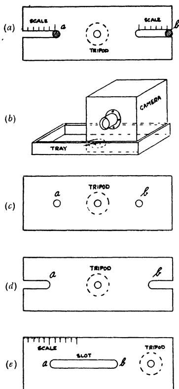
FIG. 24 — ILLUSTRATING SEVERAL ALTERNATIVE METHODS OF STEREO-SCOPY WITH A SINGLE LENS CAMERA.
