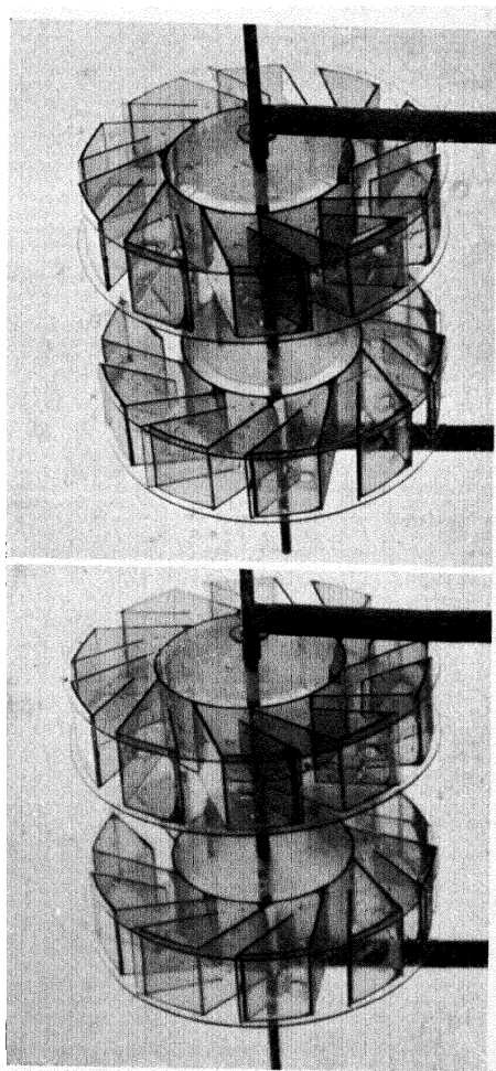
STEREOSCOPIC PAIR OF PHOTOGRAPHS OF CELLULOID WATER WHEEL FOR THERMOSTAT.
