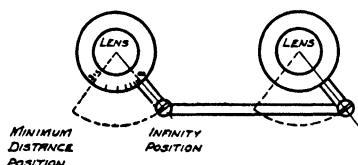
FIG. 35.—SLIDING MOUNT FOCUSING ARRANGEMENT.
