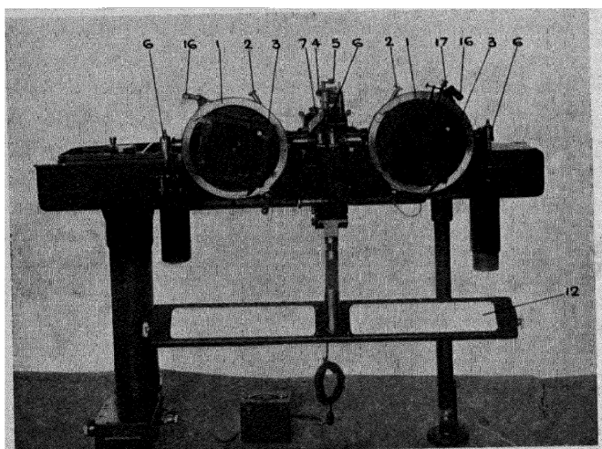
FIG. 199.—THE FOURCADE STEREOGONIOMETER (REAR VIEW).
