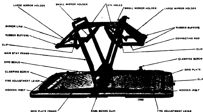
SMALL PORTABLE STEREOSCOPE, TYPE 2 D. 1
