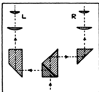
FIG. 164.—OPTICAL ARRANGEMENT OF LEITZ BINOCULAR MICROSCOPE.
