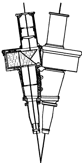
FIG. 152.—SHOWING PATH OF RAYS IN CORNEAL MICROSCOPE.
