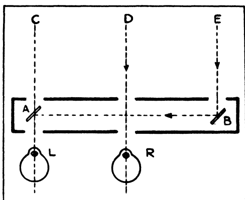
FIG. 108 —STRATTON'S PSEUDOSCOPE
