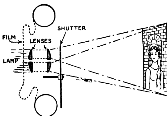
FIG 217.—THE BURKHARDT SYSTEM.
