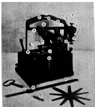
DR. MÜLLER'S UNIVERSAL X-RAY SPECTROSCOPE AS SET UP FOR THE BRAGG METHOD.
