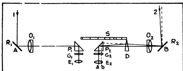
FIG. 116.—PRINCIPLE OF BARR AND STROUDE RANGE-FINDER.
