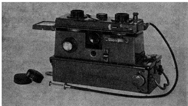
FIG. 45.—THE VÉRASCOPE "NORMAL" CAMERA FOR 45 \times 107 MM. PLATES.
