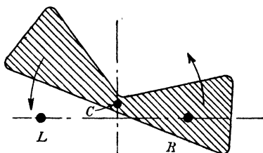
FIG. 220.—THE ROCKING SHUTTER FOR SYNCHRONIZING THE PICTURES.
