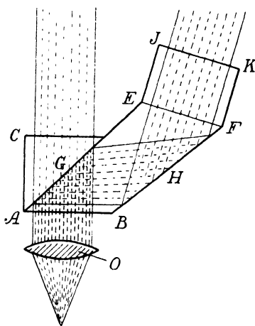
FIG. 160.—THE BECK OPTICAL ARRANGEMENT.
