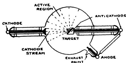
FIG. 182.—A TYPICAL X-RAY TUBE.
