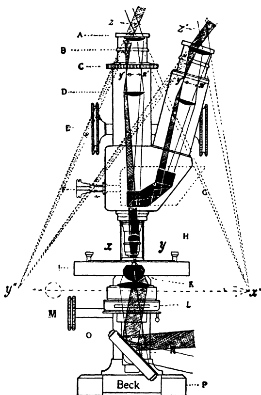
FIG. 161.—THE BECK BINOCULAR MICROSCOPE IN SECTION.
