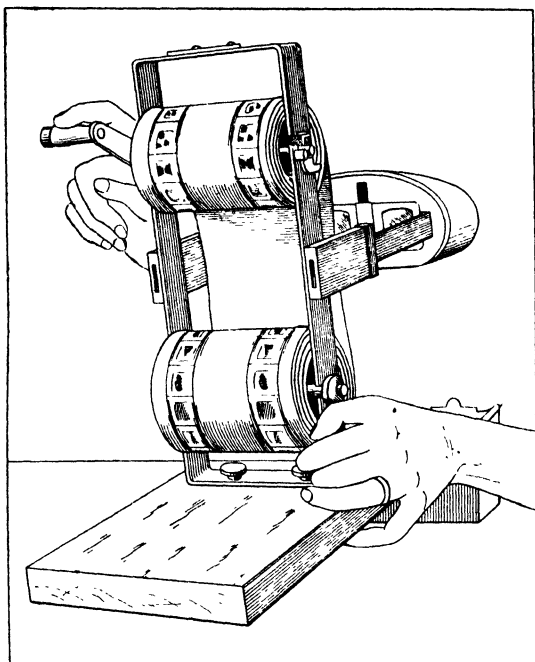
FIG. 134.—THE MAGSTER MOTION STUDY APPARATUS.
