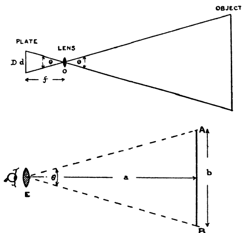
FIG. 18.—ILLUSTRATING PRINCIPLE OF VIEWING LENS OF STEREOSCOPE.
