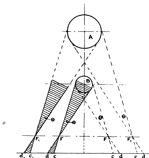
FIG. 19 --ILLUSTRATING THE PRINCIPLE OF HYPER-STEREOSCOPY.
