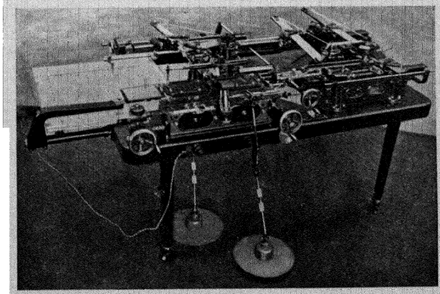
FIG. 198.—THE STEREOAUTOGRAPH (PERSPECTIVE VIEW).
