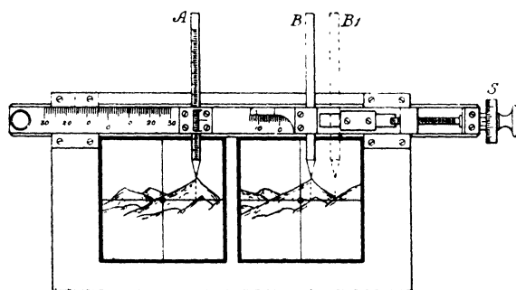
FIG. 119.—THE STEREO-MICROMETER.
