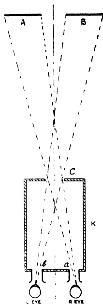
FIG. 61.—ELLIOTT'S STEREOSCOPE.
