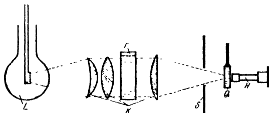
FIG. 25. L = half-watt lamp with vertical filament (15 volt, 11 amp.); K = condenser; F = heat filter (20% acid solution of ferrous sulphate, 3 cm.); Q = quartz vessel with capillary stopper containing the cell suspension; H = hand spectroscope.
