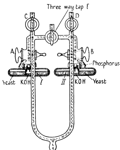
FIG. 24. Differential manometer for the determination of very small gas absorptions.
