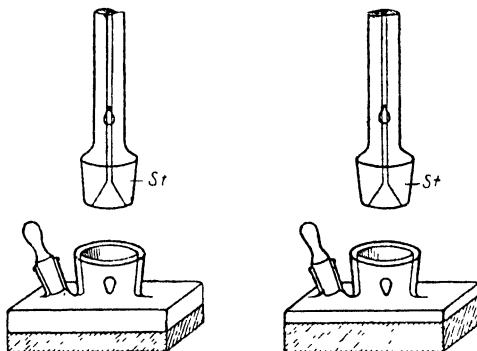
FIG. 49. Manometer vessel for the determination of \gamma . The figure shows the different fillings of the vessels by which the ratio gas space: liquid volume was altered.
