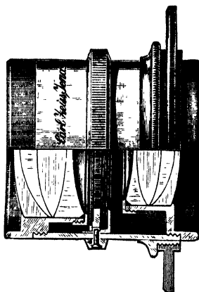
FIG. 26.—Zeiss's Anastigmat Series VIIa. (convertible).
