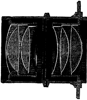
FIG. 22A.—Goerz's Double Anastigmat , Series IIa.
