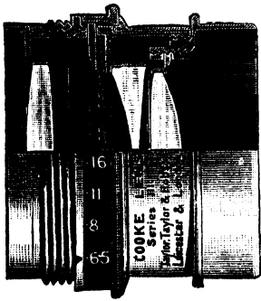
FIG. 38.—Cooke-Taylor Lens (Series III.).
