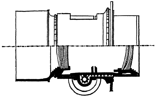
FIG. 13.—Petzval's Portrait-Objective.
