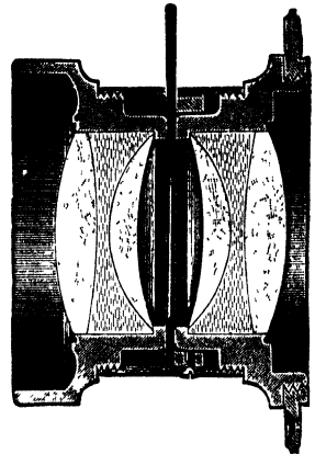
FIG. 22.—Goerz's Double Anastigmat .
