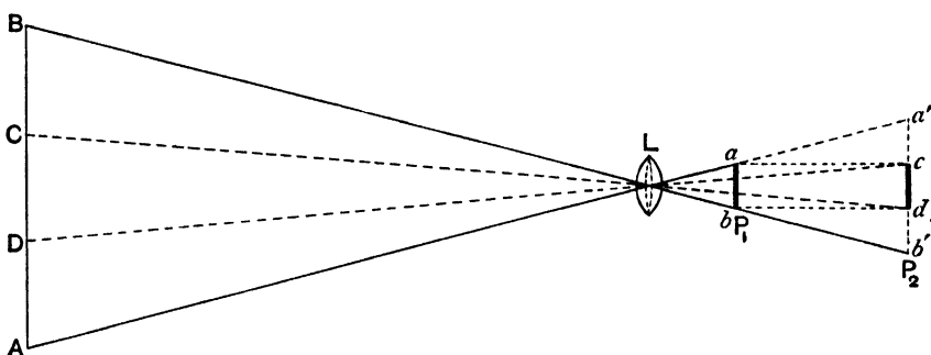
FIG. 41.—Diagram illustrating Relation between Focal Length and Size of Image.
