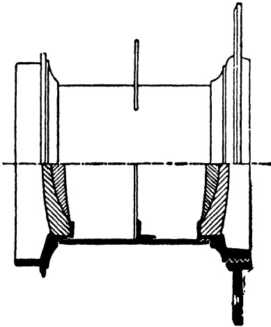
FIG. 21.—Steinheil's Aplanat .
