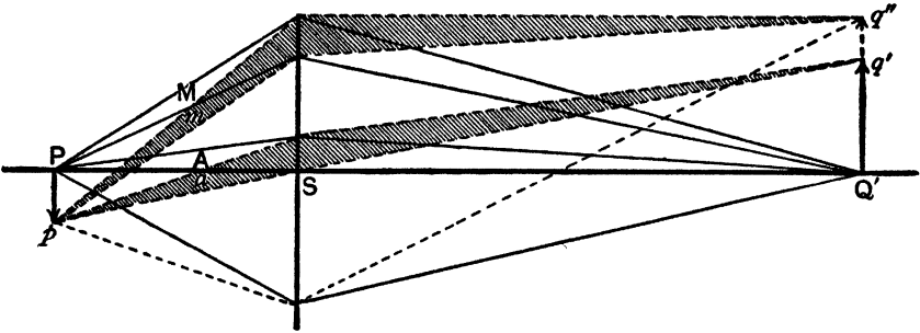
FIG. 49.—Diagram illustrating Formation of Image by Central and by Marginal Rays.
