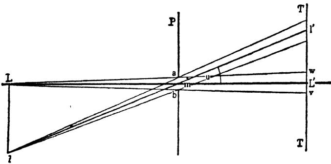
FIG. 1.—Formation of an Image in the Pin-hole Camera.
