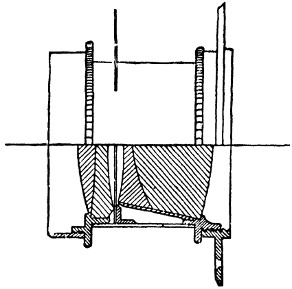
FIG. 14.—Steinheil's Antiplanet .
