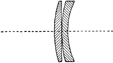
FIG. 27.—Gauss's Achromatic Objective .
