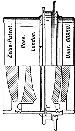
FIG. 29.—Zeiss's Unar .
