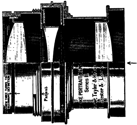
FIG. 39.—Cooke-Taylor Portrait Lens.
