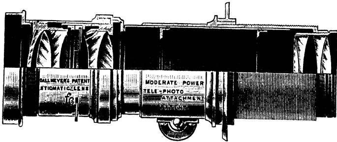
FIG. 47.—Dallmeyer's Tele-objective.
