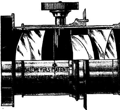
FIG. 33.—Dallmeyer's Stigmatic Lens, Series I.
