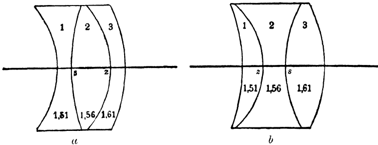
FIG. 18.—Triple cemented Anastigmatic Lenses.
