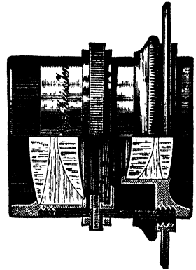
FIG. 23.—Zeiss's Anastigmat , Series VIa. (or Convertible Anastigmat ).
