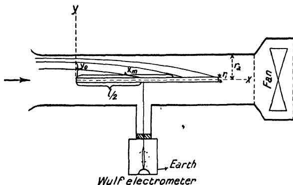
FIG. 3.—Gerdien's aspirator.
