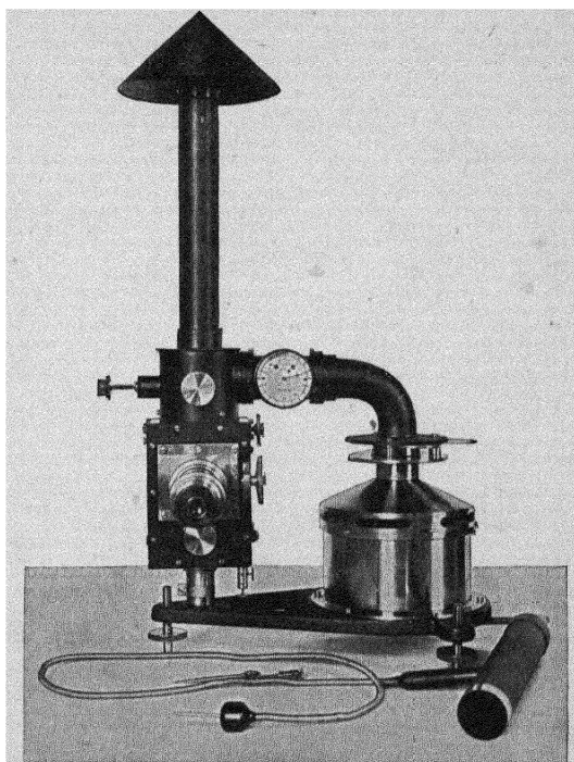
FIG. 6.—Ebert's ion counter with Wulf electrometer. (Günther and Tegetmeyer, Brunswick.)
