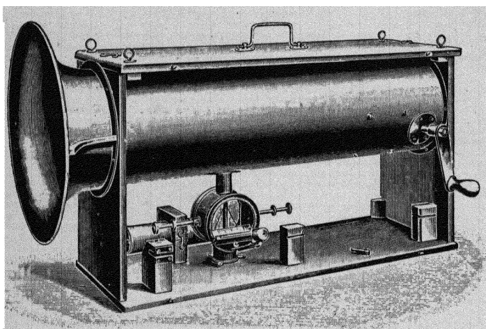
FIG. 4.—Gerdien's aspirator.
