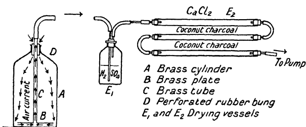
FIG. 8.—Apparatus for determining the quantity of emanation emitted by the soil. (Joly and Smyth.)
