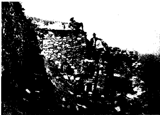
FIG. 138. Detail showing pirca construction. Photographs by courtesy of W. V. Alford, Esq.
