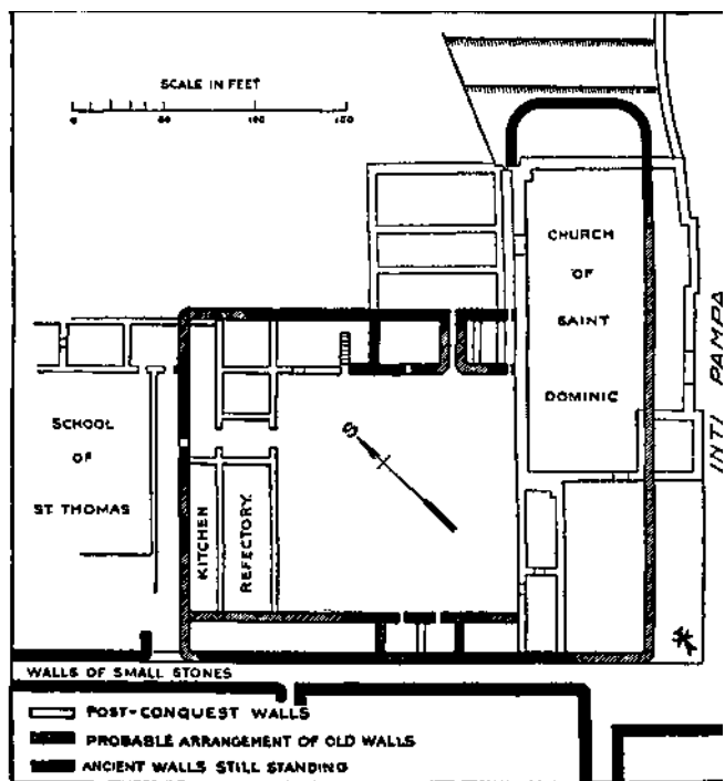
FIG. 165. Plan of Coricancha and of the monastery of St. Dominic.
