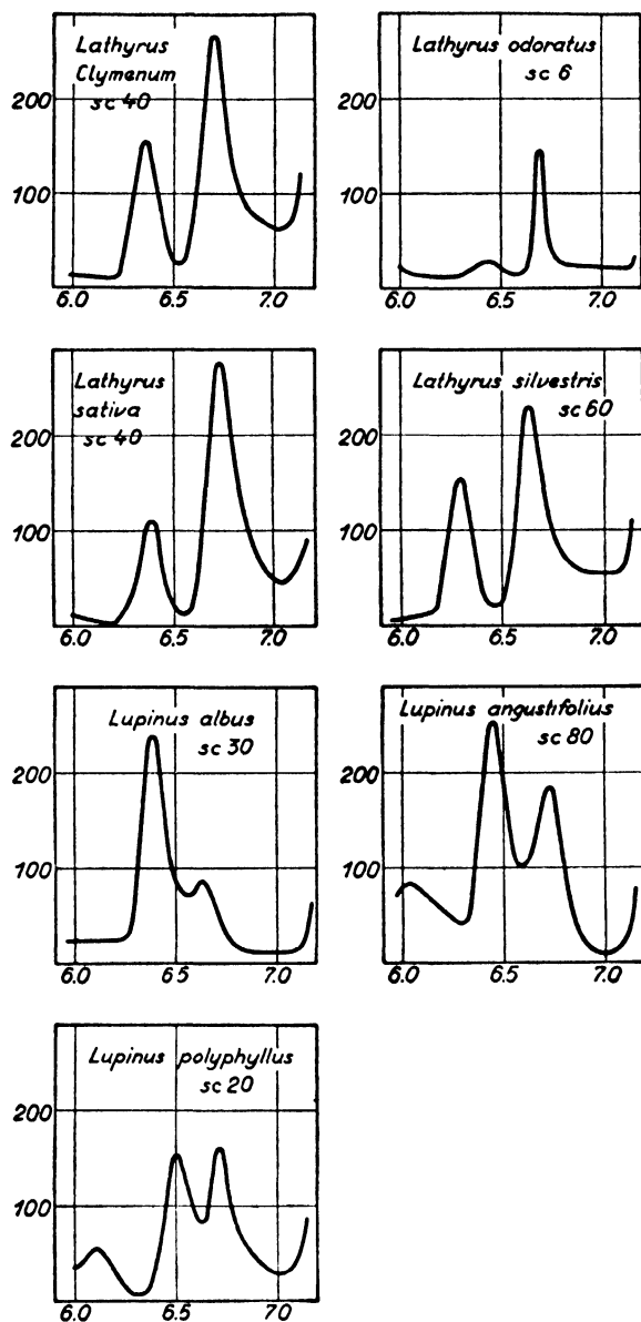
FIG. 7. Sedimentation diagrams showing the composition of globulin solutions prepared by extraction of seeds from different species of the family Leguminosae. (Danielsson, 1949.)
