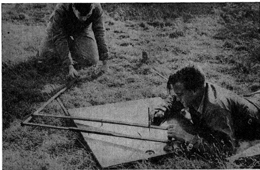
FIG. 2. (Above) A pantograph set to reduce to \frac{1}{6} . To the left is a drawing board on pegs, firmly set up the proper distance from the area to be charted. On it is fastened the pivot A of the pantograph and the drawing paper. At B is the lead which marks on the chart; at C the pointer, now at the lower left corner of the area
