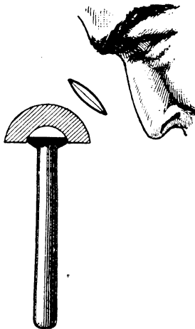
FIG. 72. Test plate examination of a small lens
