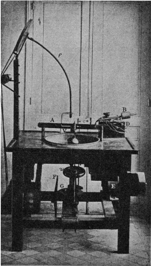
FIG. 54. Lathe with adjustable relative rotations.
