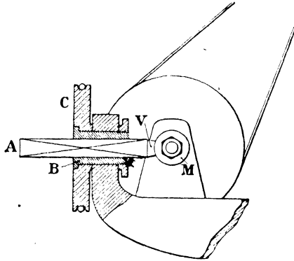
FIG. 12. Truing by milling.
