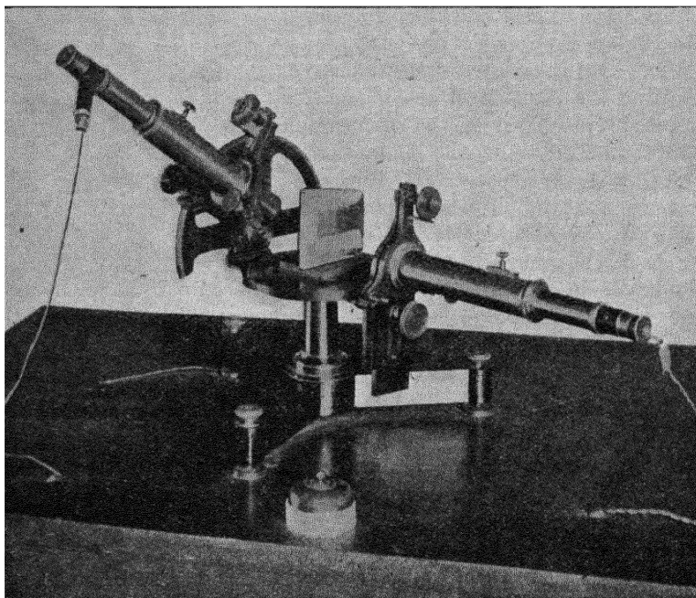
FIG. 89. Workshop goniometer.
