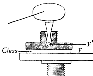
Fig 15. Ball-and-socket handle.
