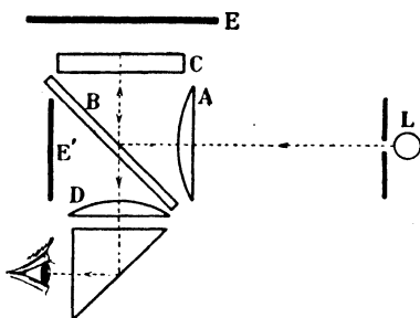
FIG. 79. Diagram of interference apparatus for testing parallel plates by observing fringes at a finite distance.
