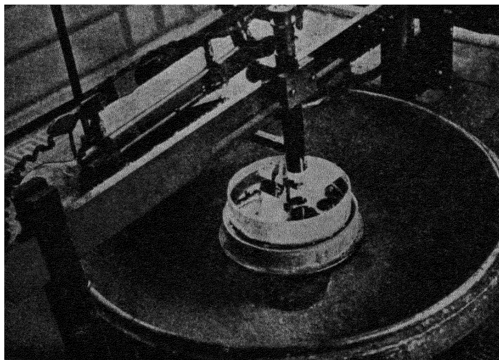
FIG. 15. Fringe viewer mounted on the bridge bar of a lathe with adjustable relative rotations.
