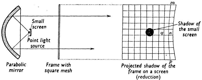
FIG. 78. Testing device for a searchlight mirror.
