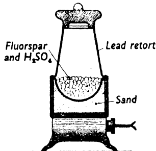
FIG. 117. Retort for acid etching.
