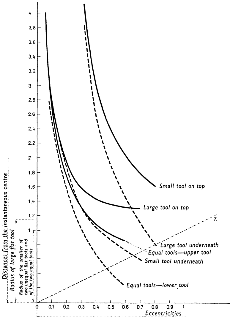
FIG. 45. Distances from the instantaneous centre as functions of the eccentricity of the two tools.
