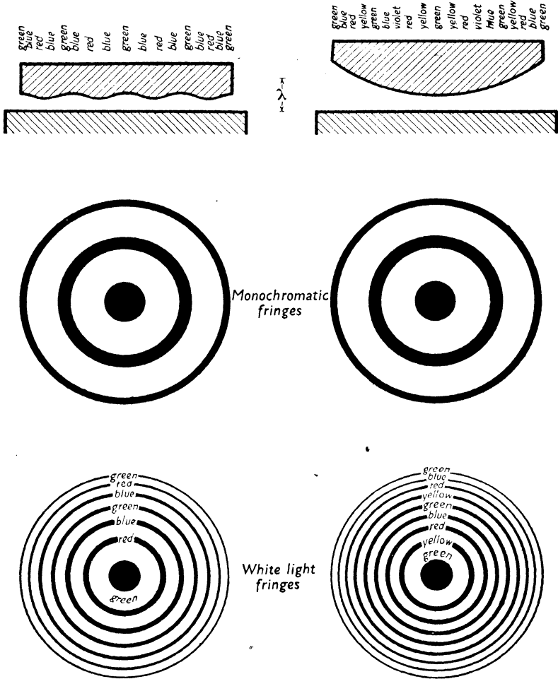
FIG. 64. Difference of contours which cannot be discerned by means of monochromatic fringes.
