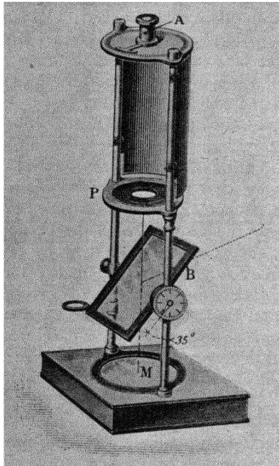
FIG. 93. Norremberg's apparatus.
