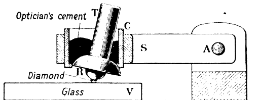
FIG. 113. Apparatus for adjusting diamonds.
