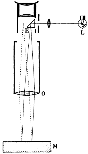
FIG. 87. Autocollimating telescope
