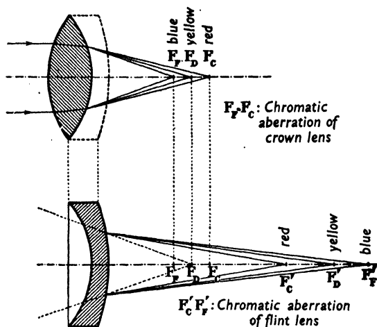
FIG. 5. Achromatic objective.
