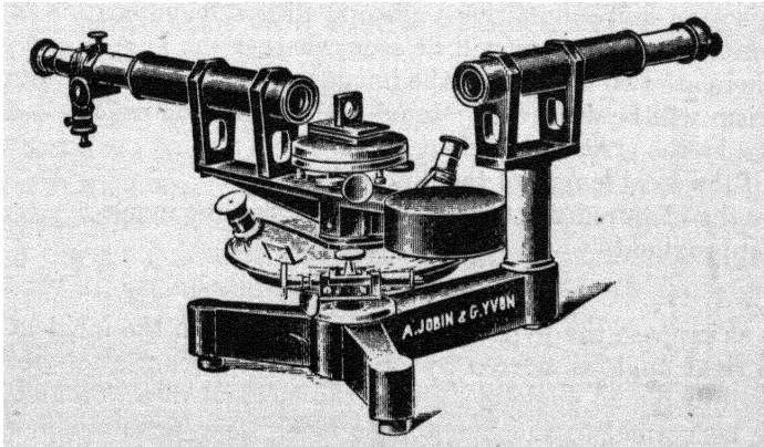
FIG. 90. Laboratory goniometer.
