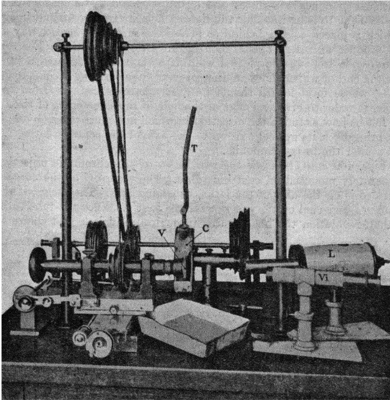
FIG. 108. Machine for centring with a light and for edging.
