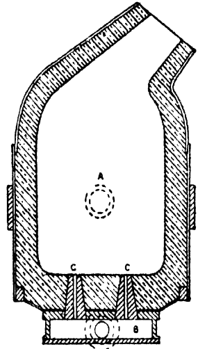
Fig. 11. VERTICAL SECTION.
