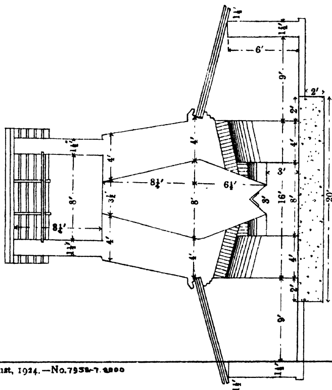
Fig. 1. SECTION.
