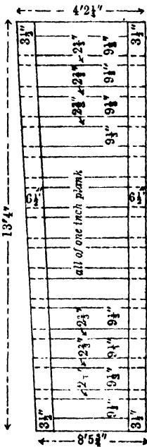
Fig. 17. TEMPLET for setting bottom brick in a Circular kiln.
