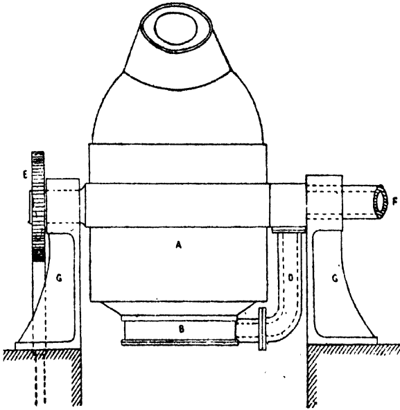
Fig. 10. FRONT ELEVATION.
