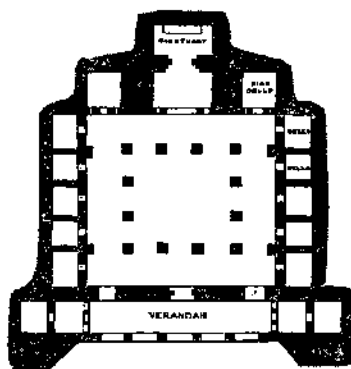
Vihara at Ajuntah. Scale W feet to 1 inch )
