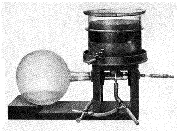
(a) The apparatus in which the tracks are produced. The chamber in which the expansion of the moist air takes place is seen at the top on the right, the tracks being photographed through the glass top.
