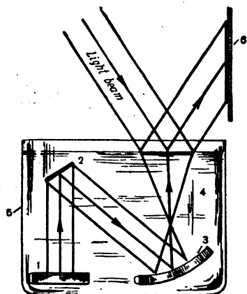
Fig. 61. Diagram of new design of supersonic microscope
