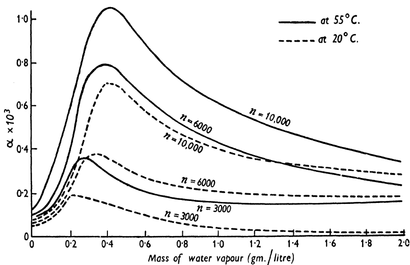
FIG. 112.—Absorption of sound in Air containing Water Vapour ( Knudsen ).
