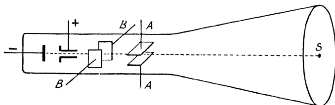
FIG. 75.—The Cathode Ray Oscillograph.
