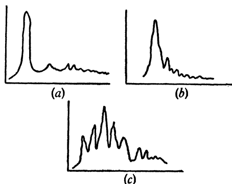
FIG. 107.—Decay of Sound in Auditorium.
