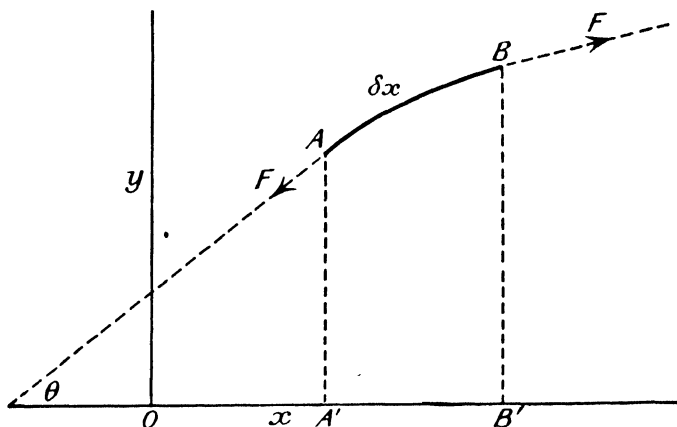
FIG. 27.—Velocity of Transverse Waves in a String.
