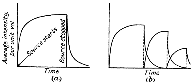
FIG. 105.—Rise and Fall of Average Intensity in a Room.
