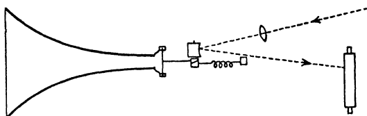
FIG. 74.—The Phonodeik ( Miller ).
