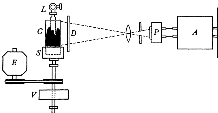
FIG. 77.—Optical Analysis of Sound Film ( Richardson ).
