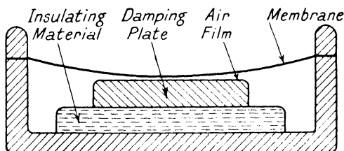
FIG. 51.—Condenser Microphone.
