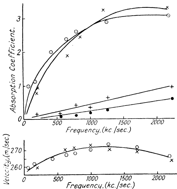
FIG. 94.—Ultrasonic Dispersion in Gases ( \bullet O 2 , + SO 2 , \times N 2 O, \circ CO 2 ).
