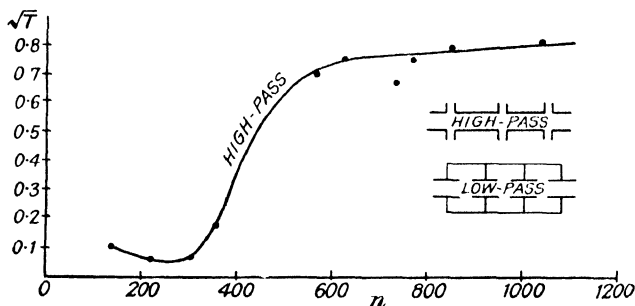
FIG. 83.—Energy transmitted by High-Pass Filter.
