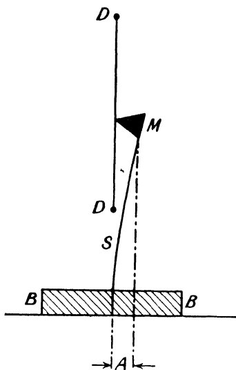
FIG. 32.—Chattering Method.
