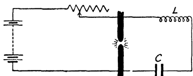
Fig. 91.—Singing Arc.
