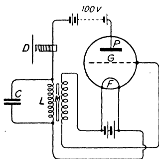
FIG. 50.—Valve-Maintained Oscillations.
