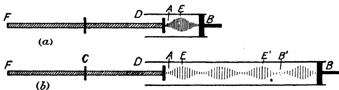
FIG. 11.—Kundt's Tube.
