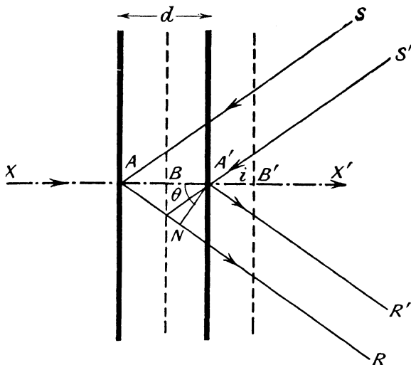
FIG. 98.—Diffraction of Light by Ultrasonic Waves.
