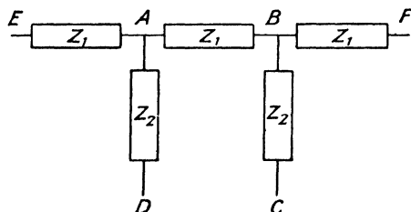
FIG. 82.—Conduit with Branches.
