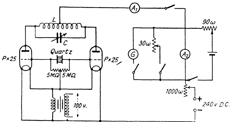
FIG. 92.—Ultrasonic Oscillator.
