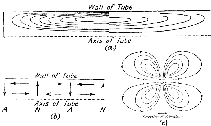
FIG. 81.—Circulations in Kundt's Tube (Andrade).
