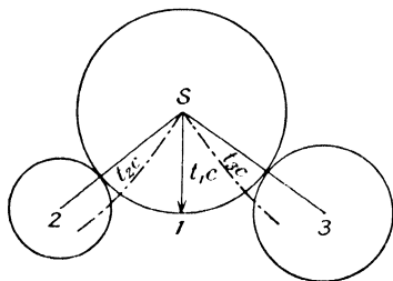
FIG. 110.—Sound Ranging.
