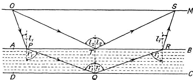
FIG. 119.—Echo-Prospecting.
