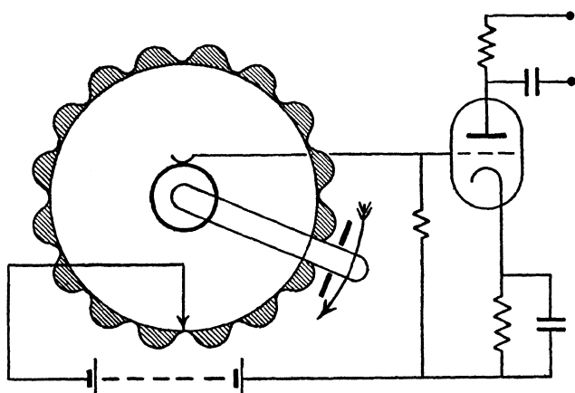
FIG. 121.—Principle of Electrostatic Tone Generator.
