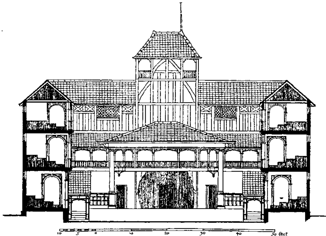
THE FORTUNE THEATRE: SECTION
