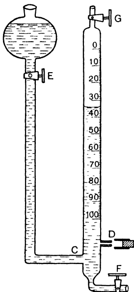
FIG. 18.—WATER-SUPPLY FOR THE MODIFIED POTOMETER.
