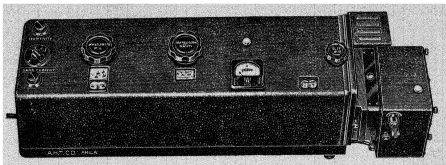
Fig. 17-11. Beckman quartz prism absorption spectrophotometer, model DU. Percentage transmission and optical density scales read with galvanometer at null. (Photo courtesy Arthur Thomas Co., Philadelphia, Pa., and Scientific Instruments Division, Beckman Instruments, Inc., Fullerton, Calif.)
