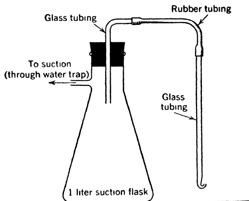
Fig. 11-3. Suction apparatus for removal of supernatant liquid.
