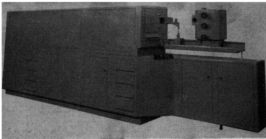
Fig. 18-6. Baird 3-meter grating spectrograph equipped with Eagle mounting (stands against wall, needing no access to back) and photographic plate recording. (Photo courtesy Baird Associates, Cambridge, Mass.)
