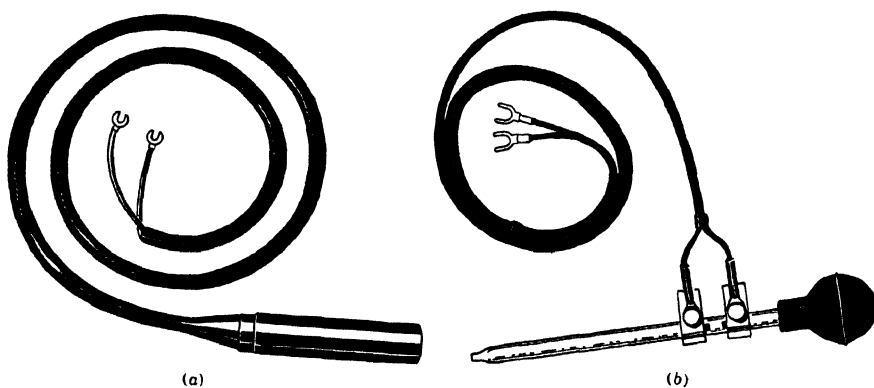
Fig. 10-4. Conductance cells suitable for soils solutions: (a), large size, requiring about 35 ml of solution; (b), small size, requiring only a few ml of solution. (Both available with a cell constant range of 0.1 to 2.0, from Industrial Instruments, Inc., Jersey City 5, N.J.)
