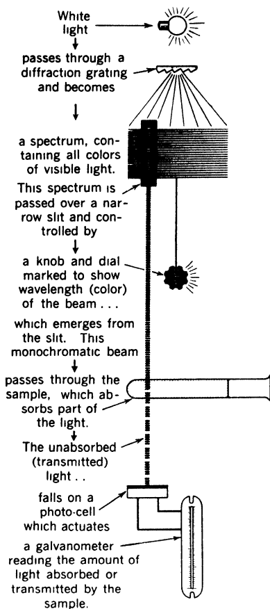
Fig. 17-14. Operating principles of the Coleman replica grating absorption spectrophotometer. (After Waco Catalyst , 9:10, 1952, Wilkins-Anderson Co., Chicago, Ill.)
