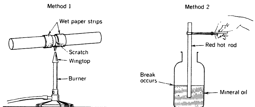
Fig. 1-2. Cutting large glass cylinders and bottles.
