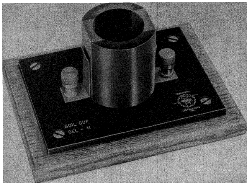
Fig. 10-1. Standard Bureau of Soils soil resistance cup. (Photo courtesy Industrial Instruments, Inc., Jersey City 5, N.J.)
