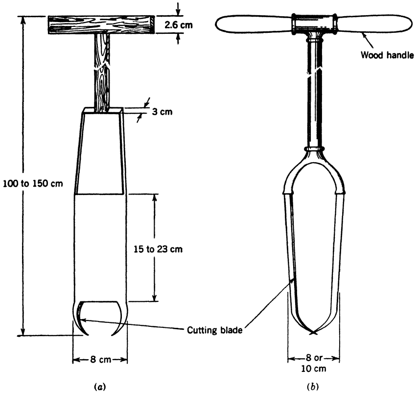
Fig. 2-2. Post-hole type soil sampling augers: (a), closed cylinder auger suitable for dry soils (after Cole and Retzer, S.S.S.A. Proc. , 1:305, 1937); (b), conventional post-hole auger.
