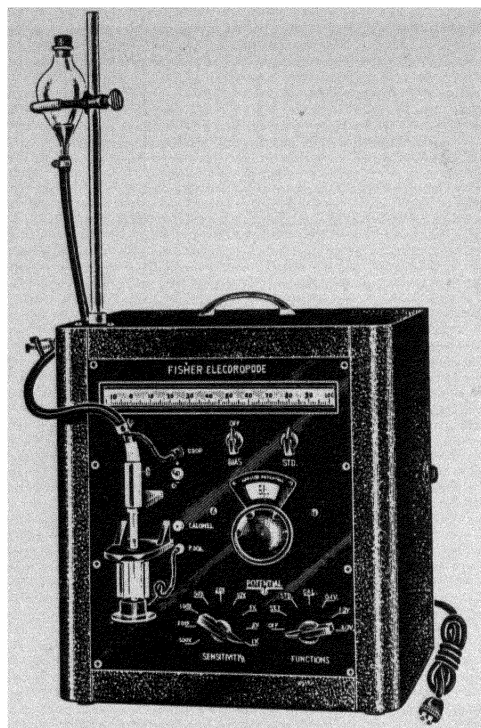
Fig. 16-5. Fisher's manually operated Electropode. (Photo courtesy Fisher Scientific Co., Pittsburgh, Pa.)
