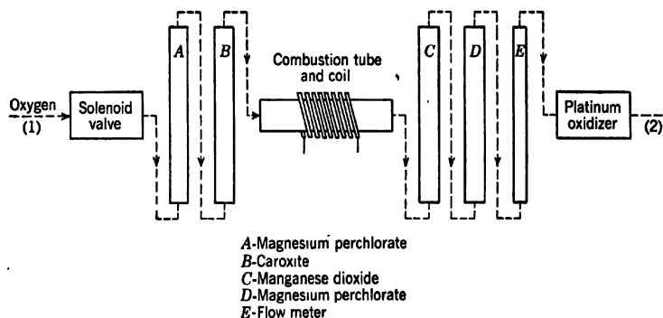
Fig. 9-2. Schematic diagram of gas train of Fisher Induction Carbon Apparatus. Letters and numbers also refer to Fig. 9-1.
