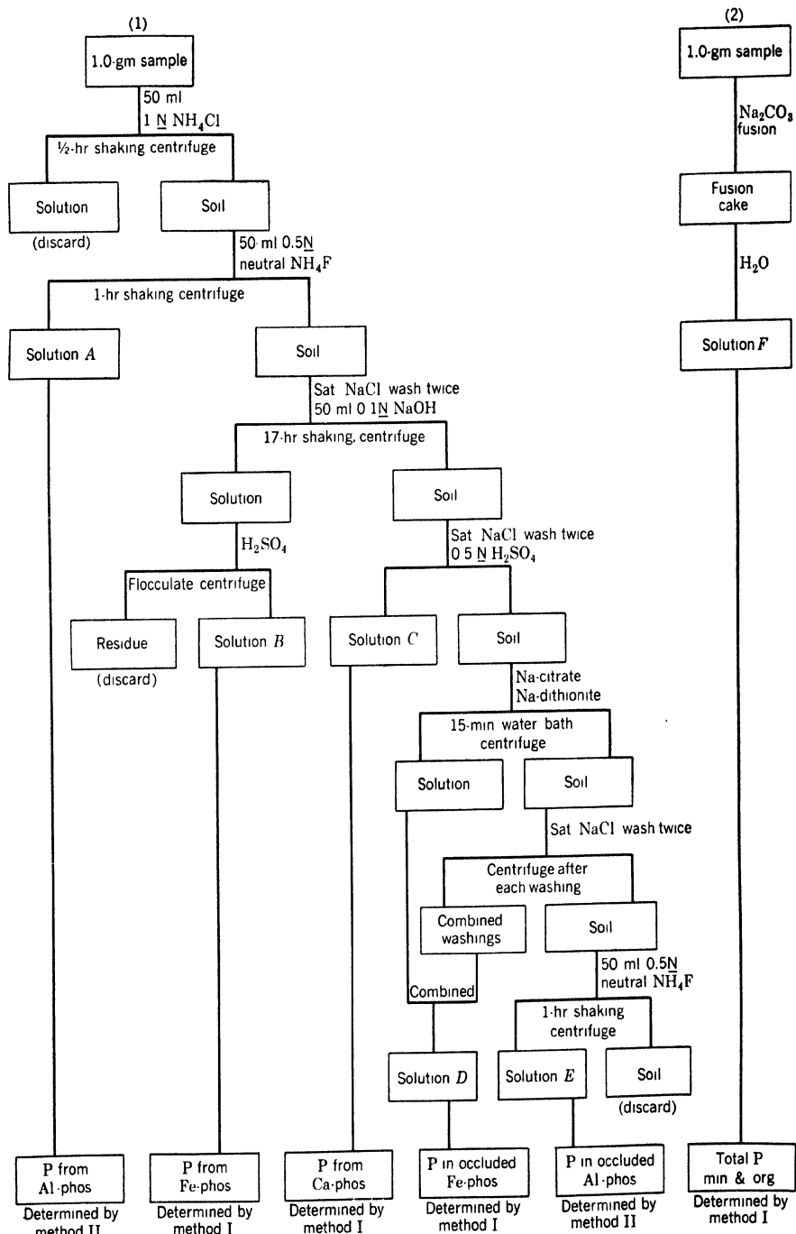
Fig. 7-2. Flow sheet for soil phosphorus fractionation system. Organic phosphorus is not included in this fractionation, but is determined separately (see Fig. 7-3).
