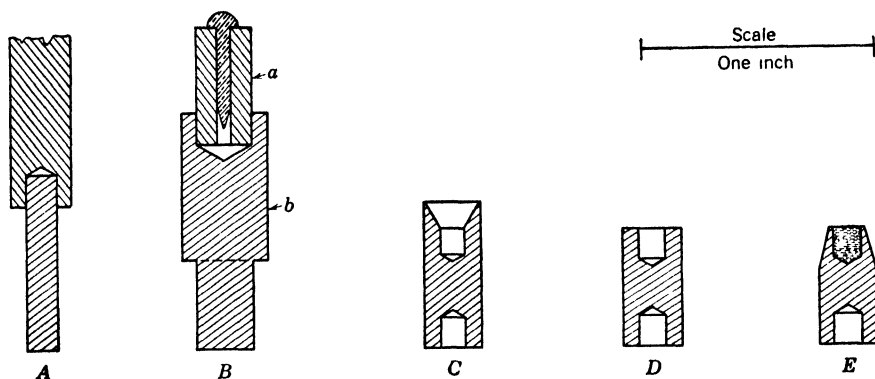
Fig. 18-9. Graphite electrodes for arc excitation of test elements in samples. A , upper, DC negative; B , lower, for iron spectra; C , sample crater, empty; D , crater for sulfide precipitates; E , sample crater filled, with excess graphite filed off. (From Vanselow and Liebig, Spectrochemical Methods , Berkeley, Calif.: University of California, 1948, p. 39.)
