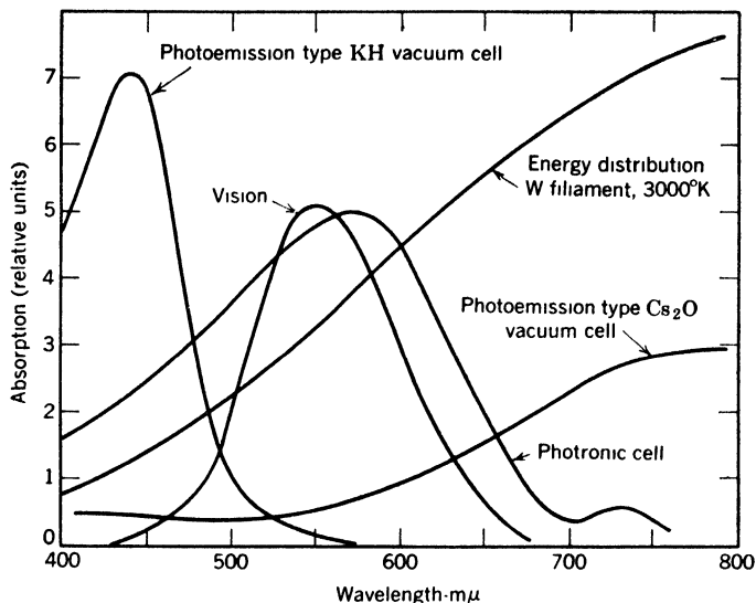
Fig. 17-1. Relative response of photoelectric cells and the human eye compared to energy distribution of wolfram (W) filament emission. (After Withrow, et al. , Ind. Eng. Chem., A. E. , 8:214, 1936.)
