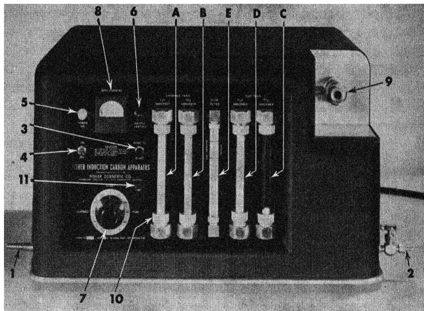
Fig. 9-1. Fisher Induction Carbon Apparatus. The sample in a combustion boat is placed in a combustion tube at 9 and oxygen is passed into 1 and out at 2, sweeping the \text{CO}_2 along. Other features are explained in Fig. 9-2 and the text.
