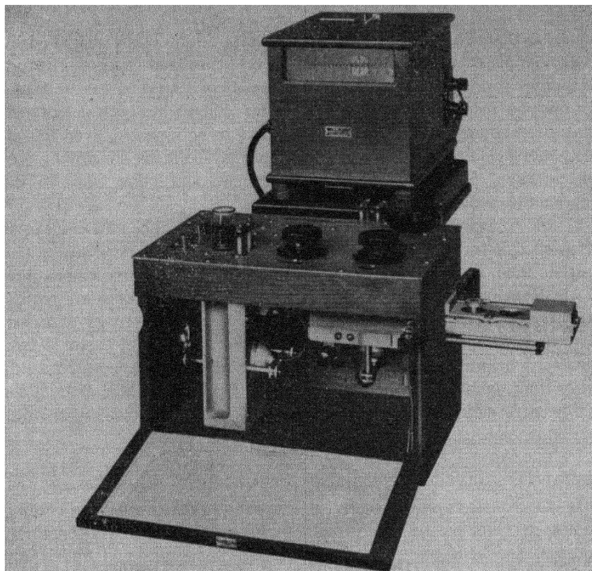
Fig. 17-8. Evelyn photoelectric colorimeter, a precision light filter absorption spectrophotometer. The galvanometer reads percentage transmission on a linear scale directly from current output of photonic cell without amplification. (Courtesy Minneapolis-Honeywell Regulator Co., Rubicon Instruments, Philadelphia, Pa.)
