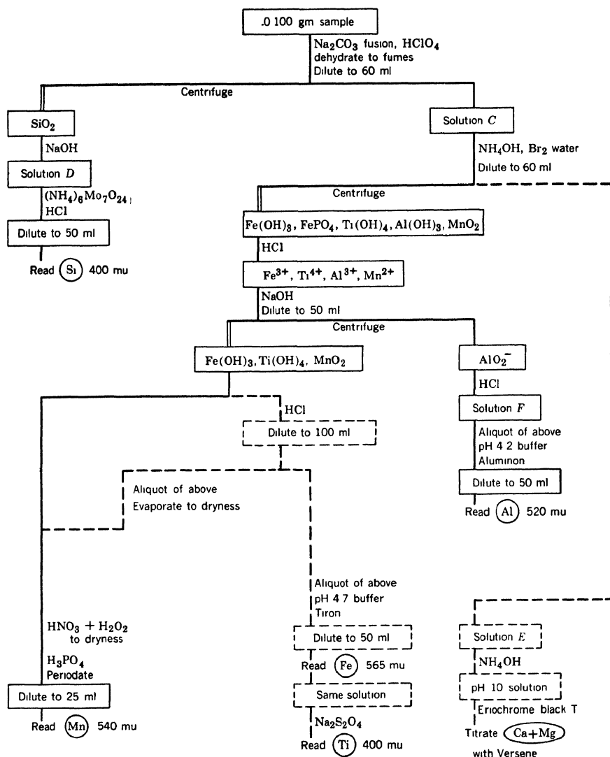
Fig. 11-2. Flow sheet for sample decomposed with \text{Na}_2\text{CO}_3 in semimicrochemical system.
