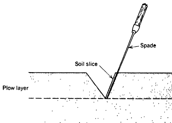
Fig. 2-8. Taking a representative thin slice of soil through the plow-layer by means of a spade. From 10 to 20 such slices are composited for one sample.
