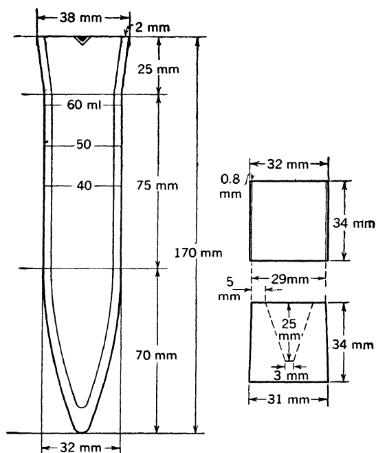
Fig. 11-4. Special 60-ml pointed centrifuge tube and special rubber cushion enclosed in brass cylinder for support during centrifugation. (After Corey and Jackson, Anal. Chem. , 25:624, 1953.)
