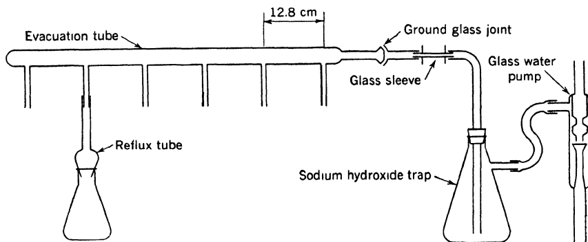
Fig. 12-1. Apparatus for wet oxidation of organic tissue in \text{HNO}_3\text{-H}_2\text{SO}_4\text{-HClO}_4 mixture. Special reflux tubes and manifold provide for evacuation of \text{HClO}_4 fumes through an \text{NaOH} trap and their discharge into the sewer line. (Apparatus developed by author and associates at the University of Wisconsin; available from Erway Glassblowing, Oregon, Wis.)
