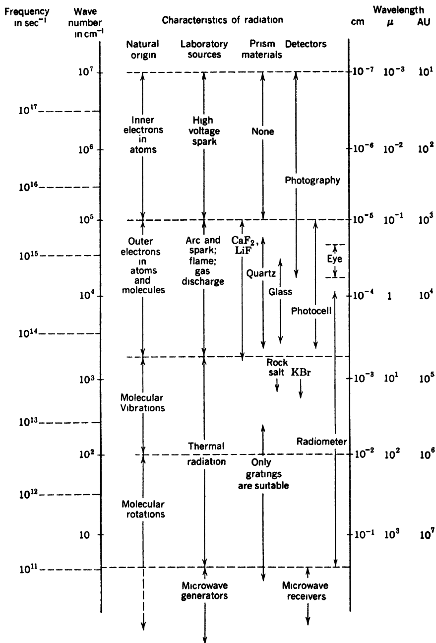
Fig. 18-1. Emission spectral regions and instrumental conditions for excitation and detection. (From Harrison et al. , Practical Spectroscopy , Englewood Cliffs, N.J.: Prentice-Hall, Inc., 1948, p. 3.)
