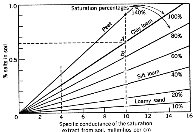
Fig. 10-6. Relationship of percentage of soluble salts to specific conductance of the saturation extract of soils of varying texture. The moderately saline limit at 4 mmho/cm falls at widely varying percentages of salts, depending on the soil texture. (After Richards, op. cit. , p. 17.)
