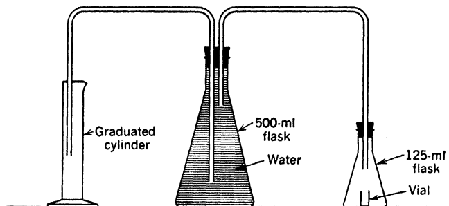
Fig. 4-4. Apparatus for gasometric determination of \text{CaCO}_3 equivalence of limestone by volume of \text{CO}_2 evolved. (After Horton and Newsom.)
