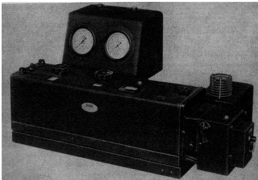
Fig. 18-2. Beckman quartz prism single-beam spectrophotometer equipped with flame emission source, model DU. Percentage transmission and optical density scales read these properties of the spectral line with the galvanometer at null. (Photo courtesy Arthur H. Thomas Co., Philadelphia, Pa., by permission of Scientific Instruments Division, Beckman Instruments, Inc., Fullerton, Calif.)
