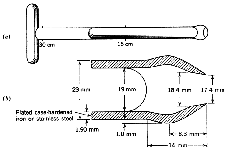
Fig. 2-4. Details of construction of cut-away soil sampling tube: (a), depth intervals grooved each 15 cm (6 inches), lengths of 33 and 93 cm are convenient; (b), details of hardened cutting edge, which should be hard enough to resist bending if thrust into gravel, but not hard enough to be brittle.
