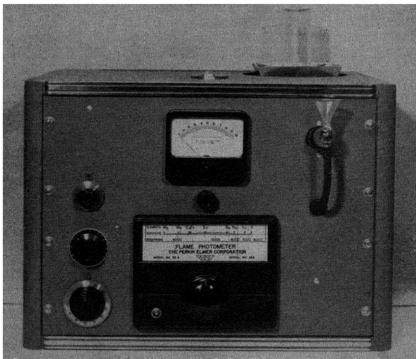
Fig. 18-3. Perkin-Elmer prism double-beam flame spectrophotometer, model 52C. (Photo courtesy Perkin-Elmer Corp., Norwalk, Conn.)
