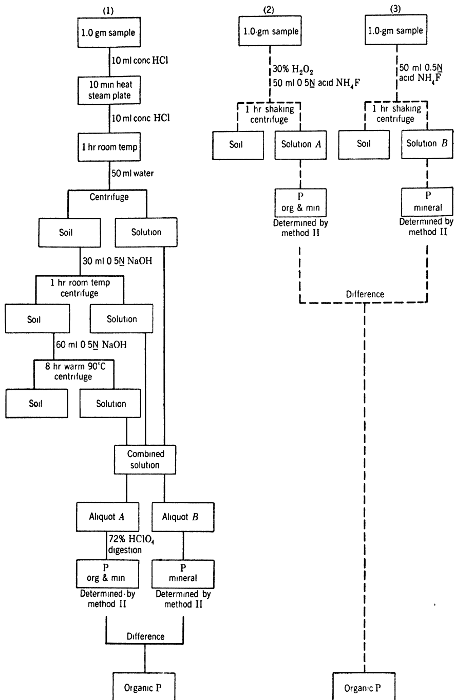
Fig. 7-3. Flow sheet for determination of soil organic phosphorus. Dotted lines indicate an alternative procedure.
