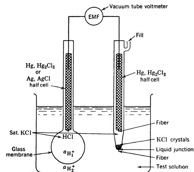
Fig. 3-2. Glass electrode system for measurement of pH.
