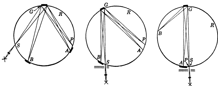
Fig. 18-4. Principle of the Rowland Circle and the optics of the grating spectrograph. R , the Rowland Circle; S , entrance slit; G , diffraction grating; P , principal focus, white light; A , B , spectral distribution of images of slit, dispersed linearly about the circumference of the circle. Left diagram, Paschen mounting in which recorders are placed at A and B . Middle and right diagrams, Eagle mounting, in which movement of the grating brings different portions of the spectrum into position near the entrance slit. (From Better Analysis , No. 2, p. 3, Cambridge, Mass.: Baird Associates, Inc., 1950.)
