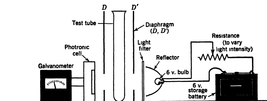
Fig. 17-9. Diagram of Evelyn colorimeter, illustrating typical components of the light filter type of absorption spectrophotometer. Special features include light filtration prior to incidence on the test solution, low energy light source, test tube comparator cell, and direct reading photonic cell, requiring no amplification.
