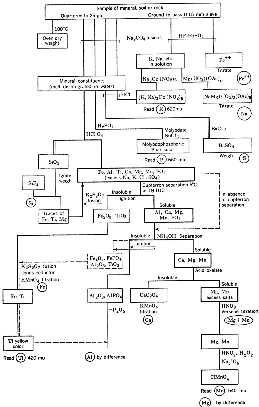
Fig. 11-5. Flow sheet for conventional system of silicate analysis.
