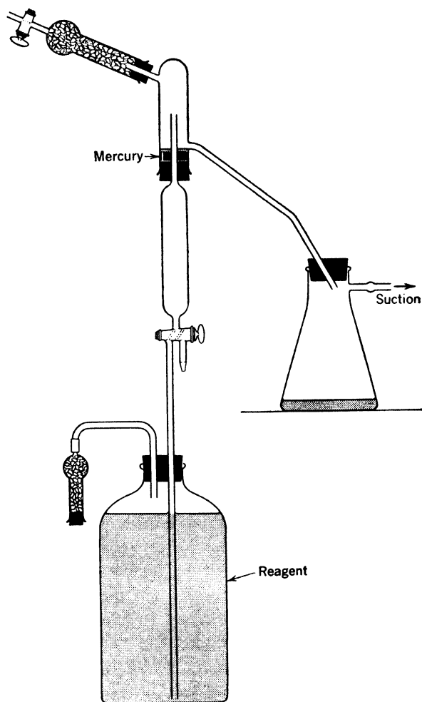
Fig. 14-1. Apparatus for dispensing quinalizarin- \text{H}_2\text{SO}_4 solution with protection from moisture of air. The volume of the reagent is exactly reproducible, though not necessarily exactly 10 ml. (After MacDougall and Biggs, Anal. Chem. , 24:566, 1952.)
