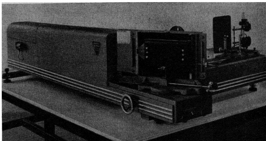
Fig. 18-7. Bausch & Lomb, Littrow prism spectrograph and illuminating unit. The usable spectrum, extending from 2100 to 8000 Å with full resolving power, is recorded photographically. (Photo courtesy Bausch & Lomb Optical Co., Rochester, N.Y.)
