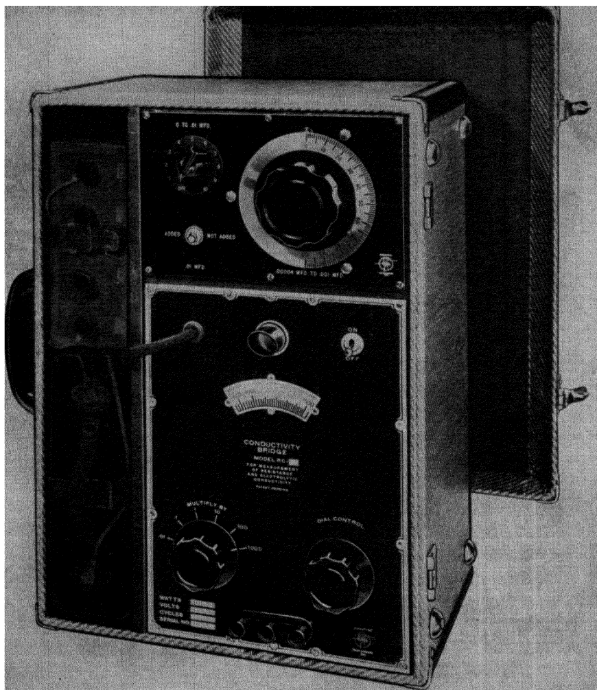
Fig. 10-2. Conductance bridge suitable for the measurement of soluble salt content of soil solutions (as well as gypsum block resistances). (Available from Industrial Instruments, Inc., Jersey City 5, N.J.)
