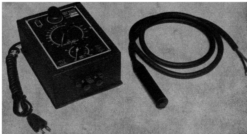
Fig. 10-3. Conductance bridge and cell suitable for measurement of electrical conductance from 0.1 to 10 millimhos/cm (nonsaline to strongly saline soil extracts). (Available from the Industrial Instruments, Inc., Jersey City 5, N.J.)
