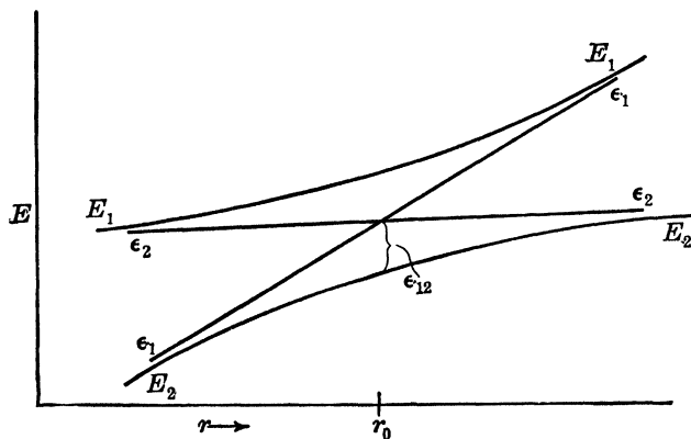
FIG. 16-11. Energy relations at point of "crossing."
