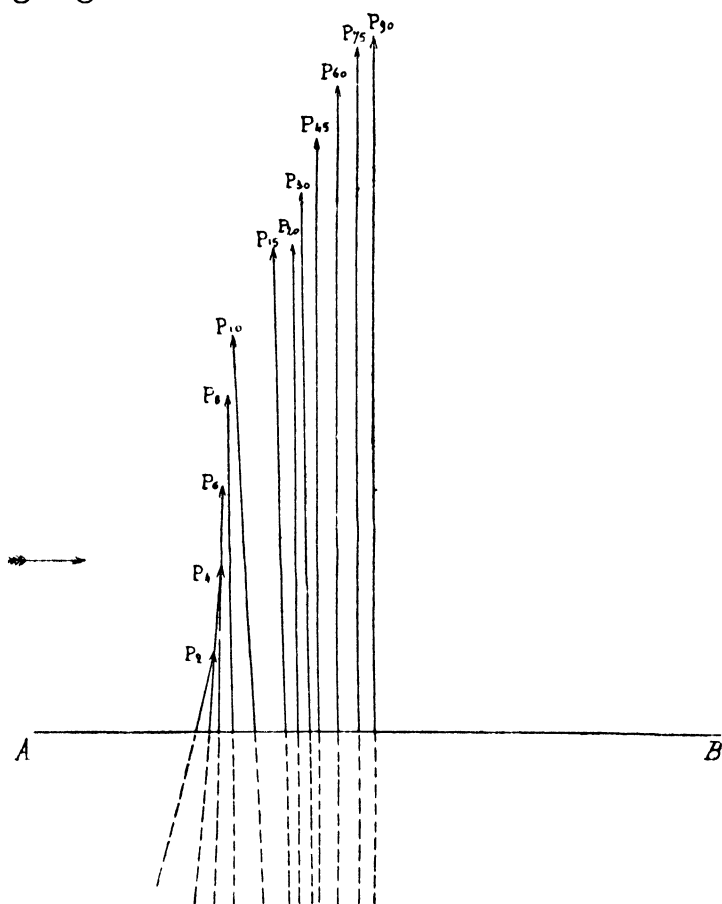
FIG. 32.—Sheaf of pressures on a flat plane.
