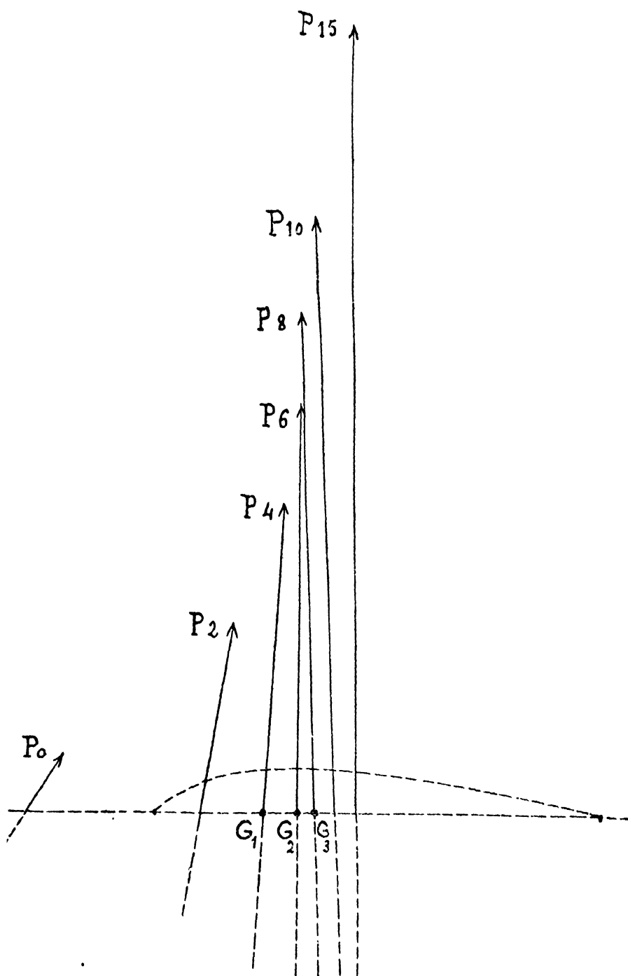
FIG. 43.—Sheaf of total pressures on a Bleriot XI. monoplane with a longitudinal V of 8^\circ .
