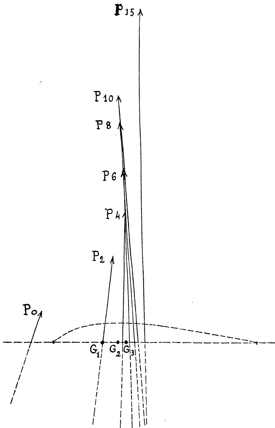
FIG. 44.—Sheaf of total pressures on a Bleriot XI. monoplane with a longitudinal V of 6^\circ .
