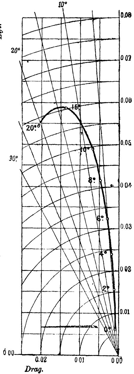
FIG. 2.—Maurice Farman plane.
