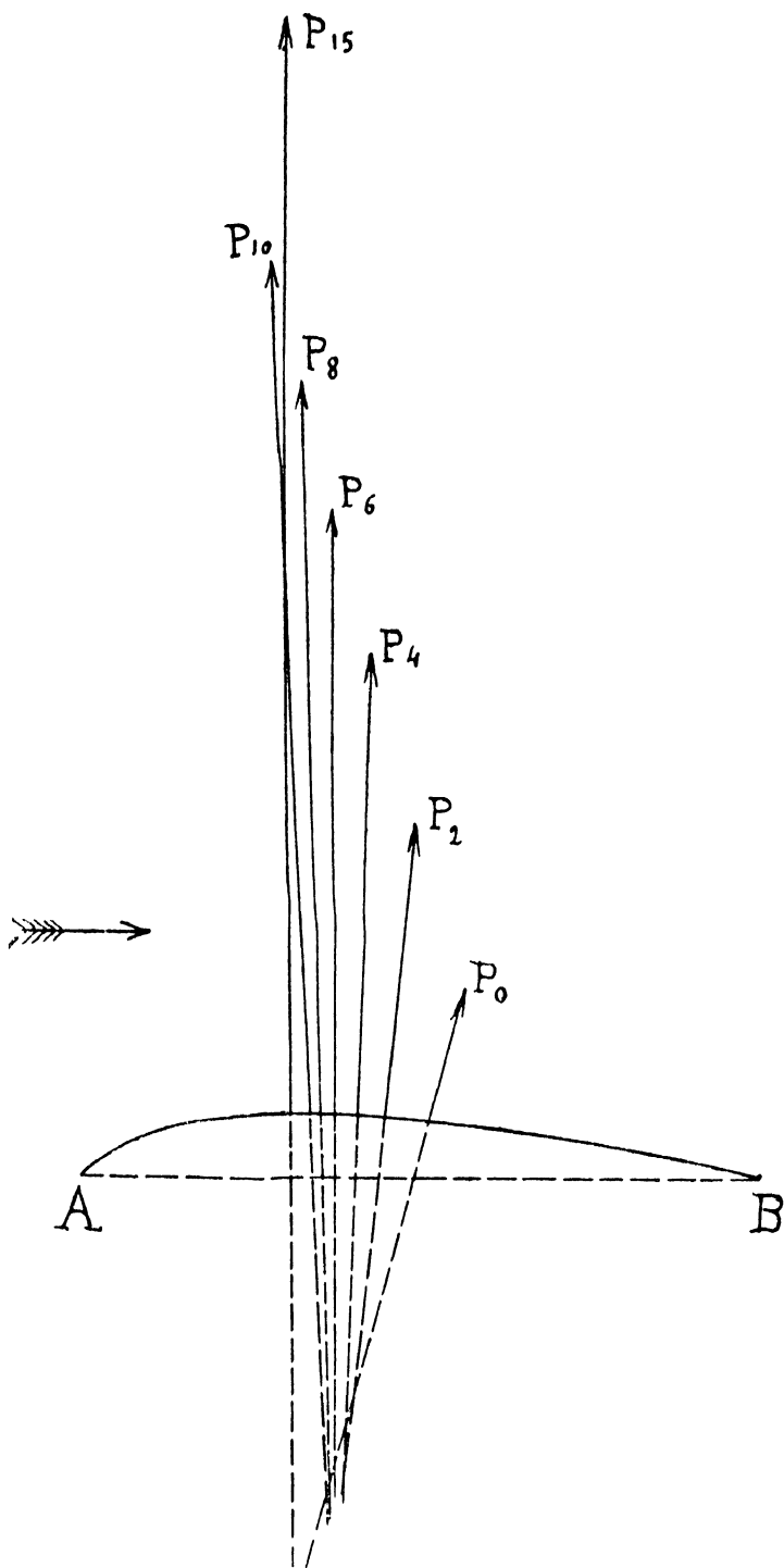
FIG. 34.—Sheaf of pressures on a Bleriot XI. plane.
