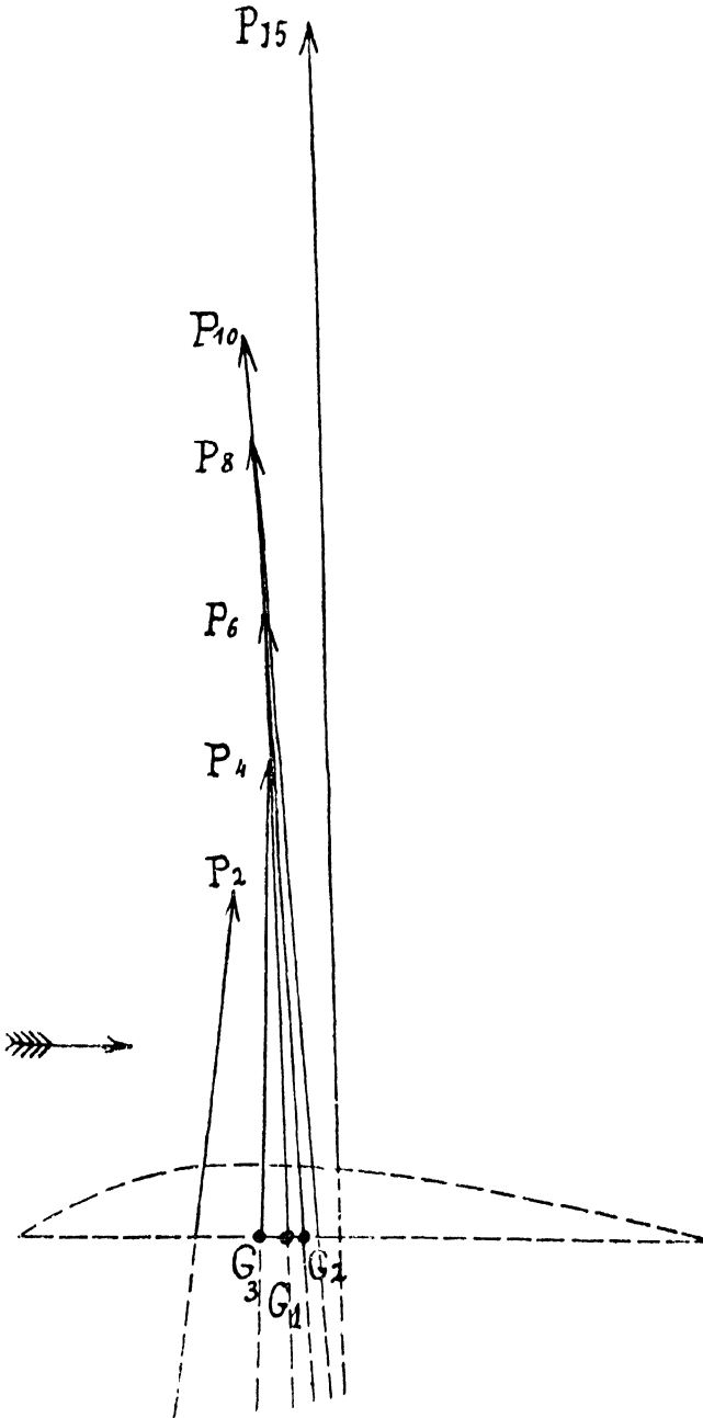
FIG. 39.—Sheaf of total pressures on a complete Bleriot XI. monoplane.
