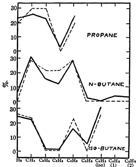
FIG. 15.—Observed (—) and calculated (---) products in the thermal decomposition of hydrocarbons.
