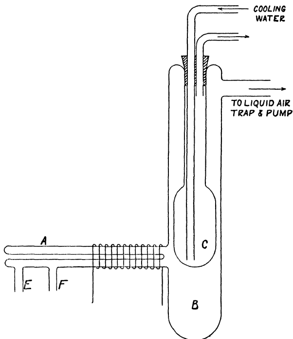
FIG. 5.—Apparatus for the identification of free radicals by combination with mercury.
