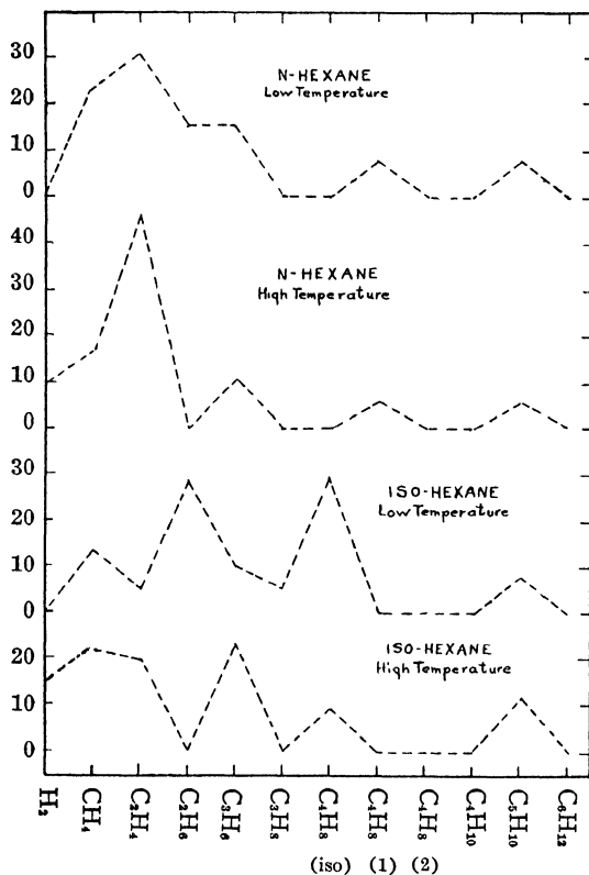
FIG. 20.—Calculated products in the thermal decomposition of hydrocarbons.
