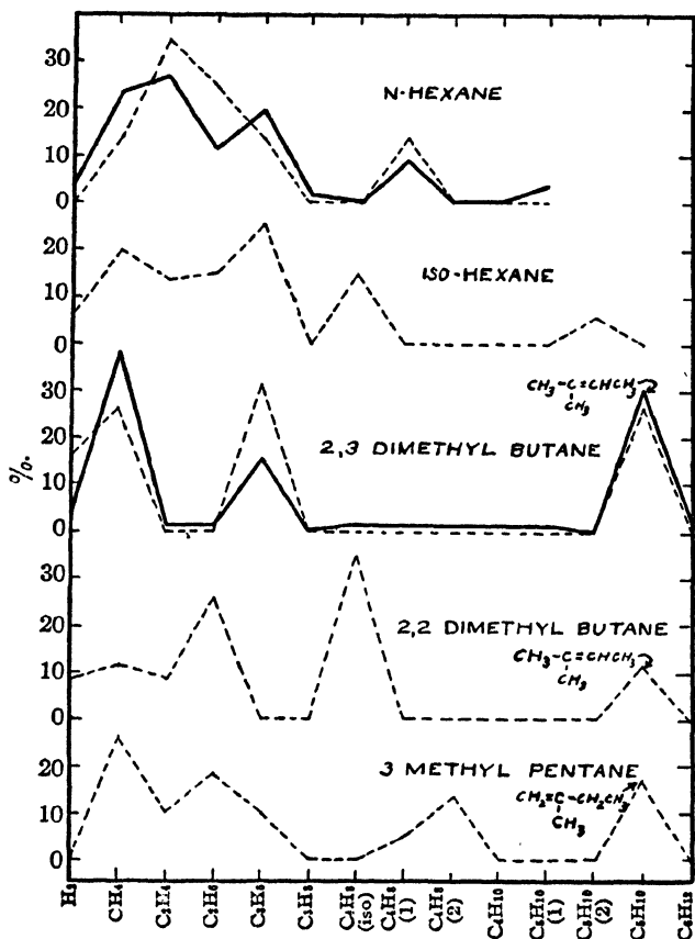
FIG. 17.—Observed (—) and calculated (----) products in the thermal decomposition of the hexanes.
