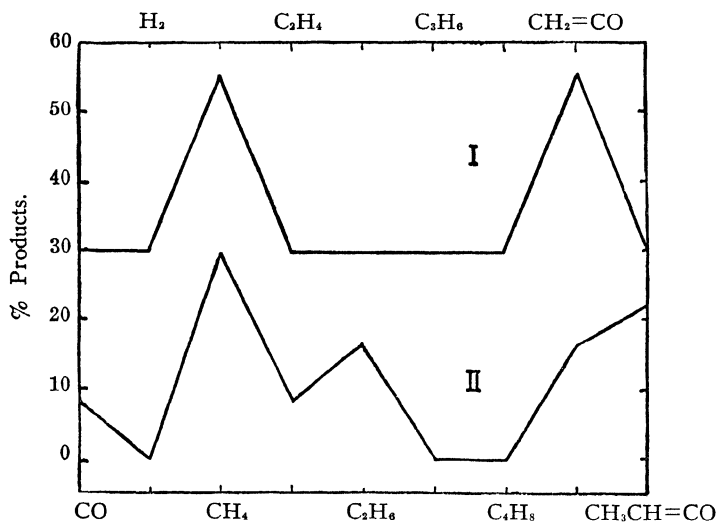
FIG. 23.—Calculated products in the thermal decomposition of acetone (I) and methyl ethyl ketone (II).
