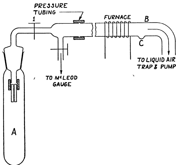
FIG. 3.—Apparatus for preparing free radicals by the thermal decomposition of organic compounds.
