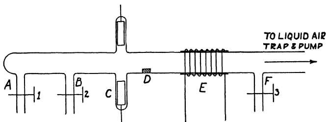
FIG. 4.—Apparatus for preparing free radicals by the electrical decomposition of organic compounds.
