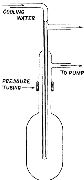
FIG. 8.—Apparatus for subliming alkyl mercuric halides
