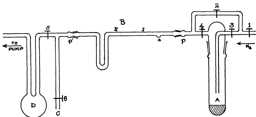
FIG. 1.—Apparatus for preparing methyl radicals from tetramethyl lead, using hydrogen as carrier gas.
