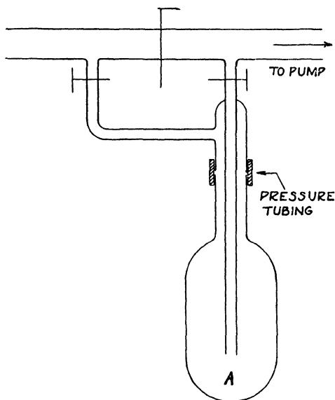
FIG. 7.—Apparatus for preparing alkyl mercuric halides.
