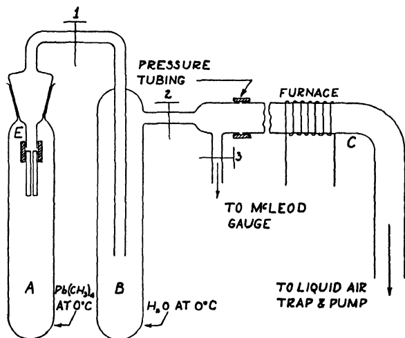
FIG. 2.—Apparatus for preparing methyl radicals from tetramethyl lead, using water vapor as carrier gas.
