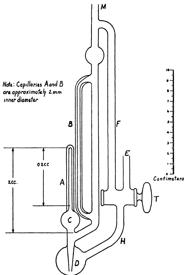
FIG. 6.—McLeod gauge.
