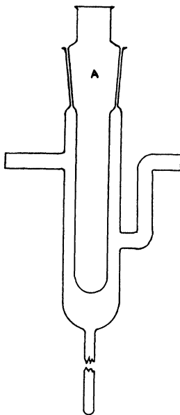
FIG. 10.—Trap for collecting dimethylditelluride.
